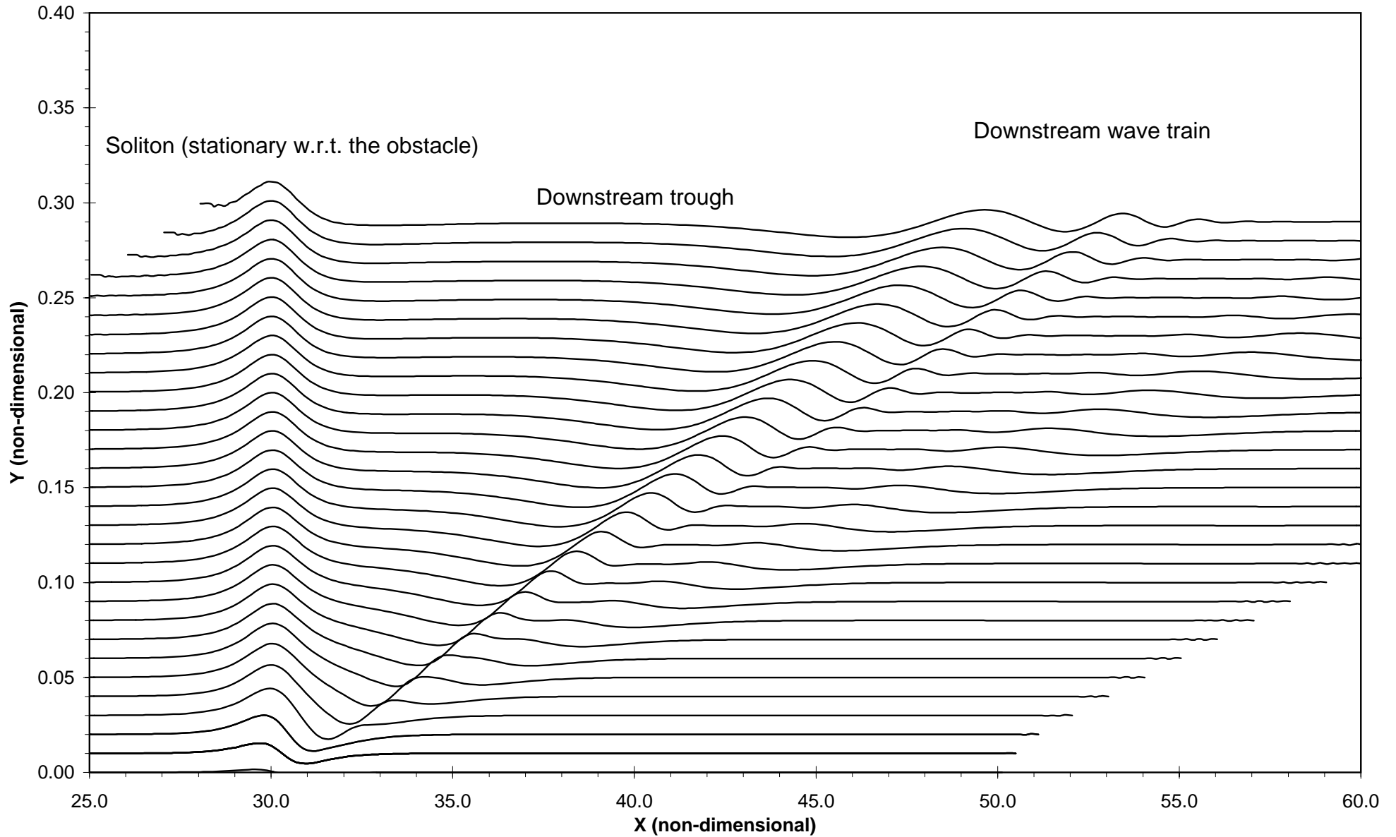
Figure II-6: Sample free surface profile for supercritical flow.
