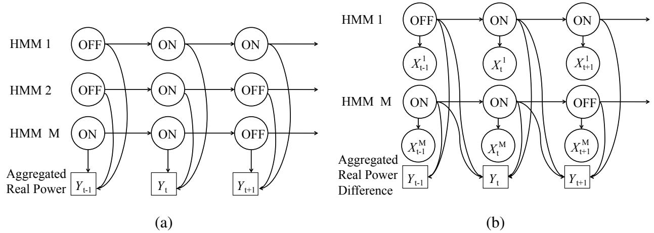
Figure 2.21: Graphical model with M devices. (a) FHMM and (b) Difference FHMM.
