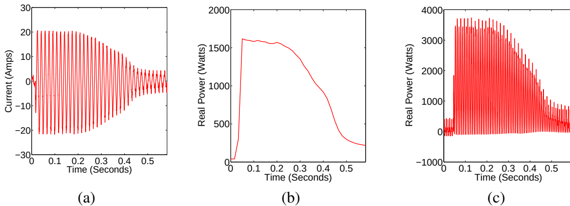
Figure 2.11: (a) Transient and Steady State of a Sinusoidal Current from a Refrigerator. Transient Shapes for a Refrigerator (b) Real Power and (c) Instantaneous Real Power.
