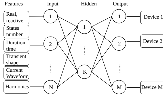
Figure 2.18: Neural Network Approach for Energy Disaggregation.
