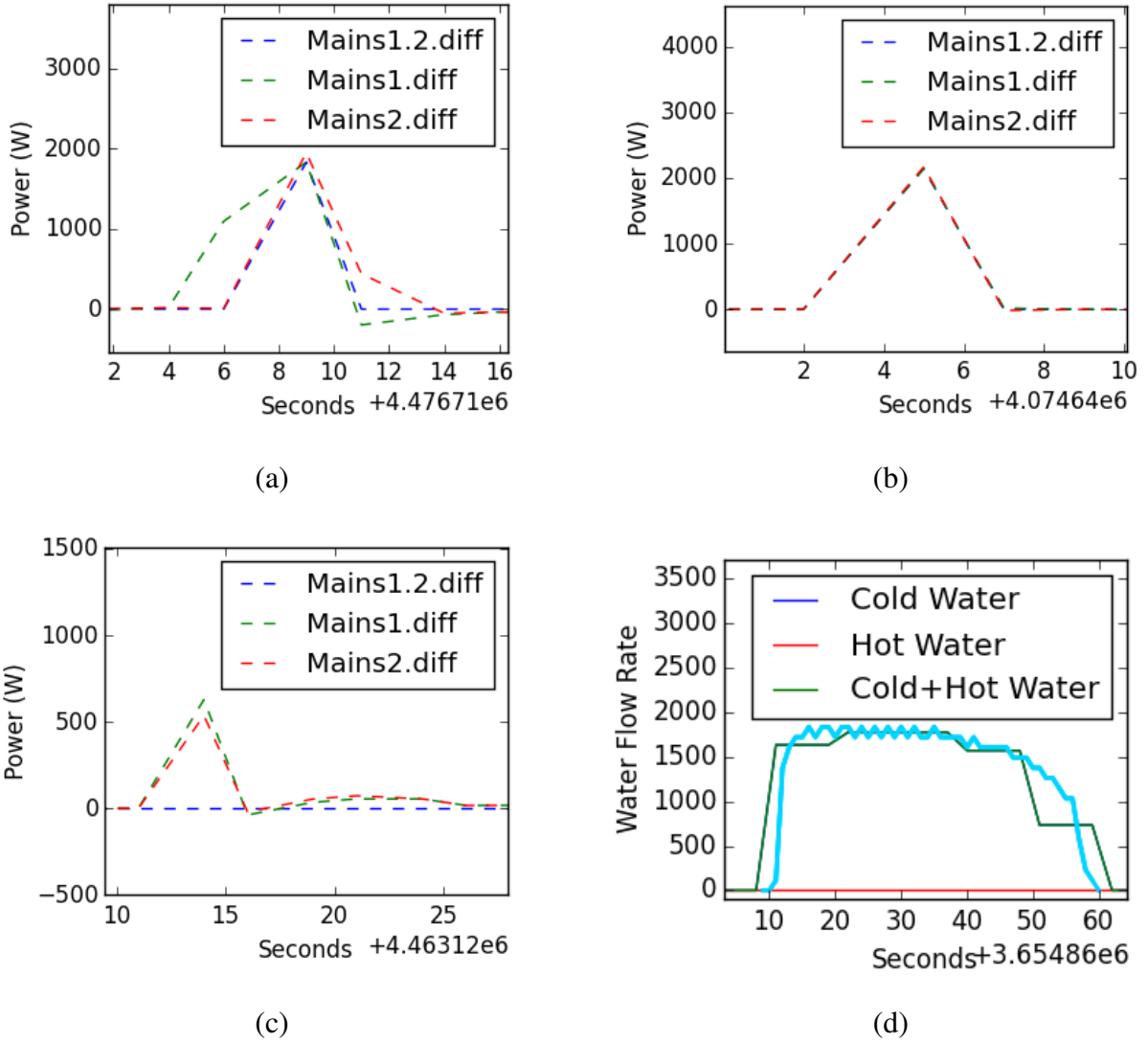
Figure 4.5: Disaggregating dryer and continuous variable load heatingOutdoor with multivariate motif mining. The on event of a device and the corresponding diffs in the two phases for (a) dryer, (b) water heater, (c) heatingOutdoor. (d) Disaggregating the toilet water use end with dynamic time-warping subsequence search. This Y-axis is water flow rate in 10000*liter/minute.
