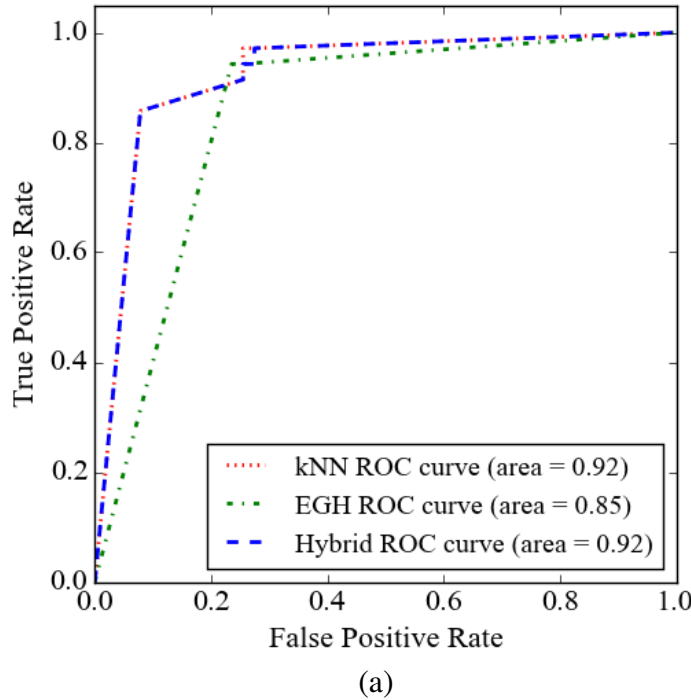
Figure 5.5: ROC curve of house occupancy prediction in Study10 (02/20/2014).
