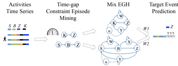
Figure 5.1: Occupancy Prediction Framework.
