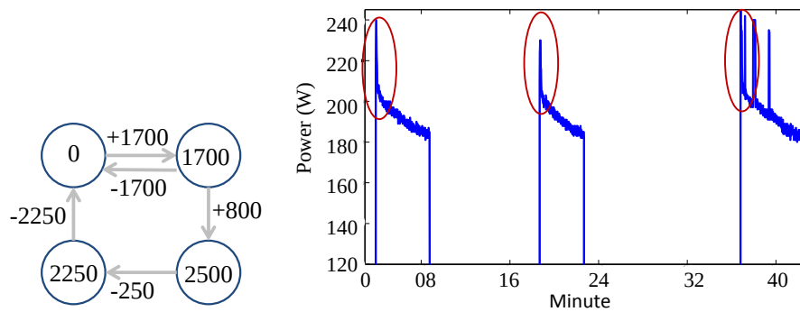
Figure 3.2: Steady state transitions and transient features at startup.
