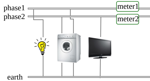
Figure 3.1: A residential setup for data collection.
