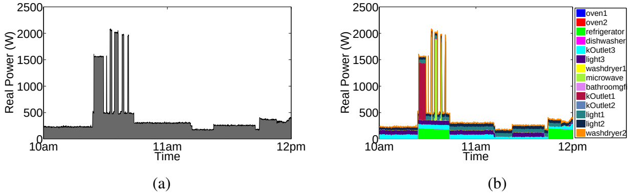
Figure 2.1: (a) Aggregate power input to a disaggregation algorithm. (b) Disaggregated information about devices and their power usage patterns.
