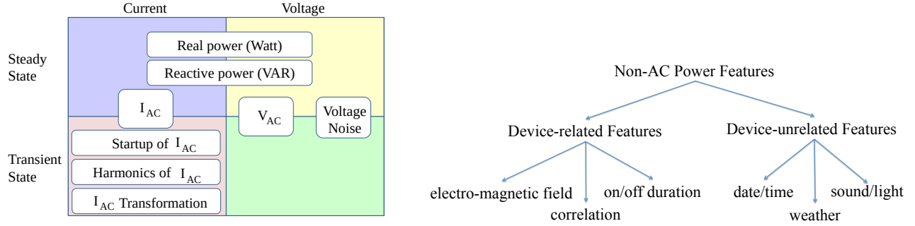
Figure 2.10: Category of (a) AC Power Features and (b) Non-AC Power Features.
