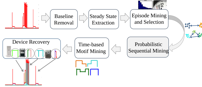
Figure 3.4: Temporal motif mining framework for disaggregation.
