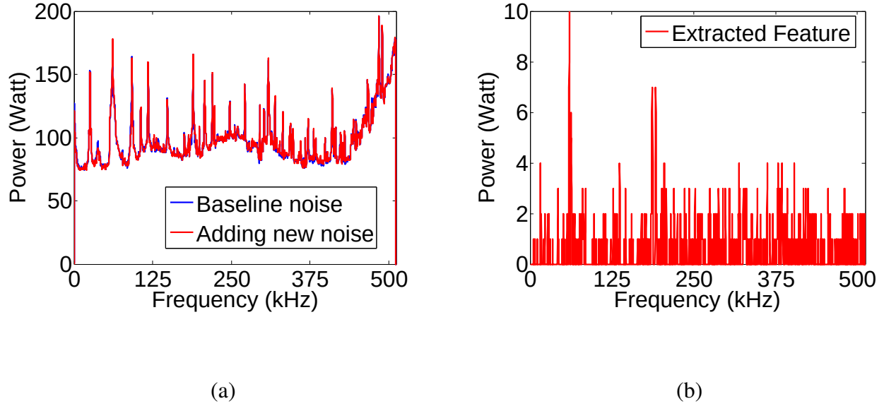
Figure 2.16: (a) Baseline noise with newly added noise. (b) Noise Feature of a device.
