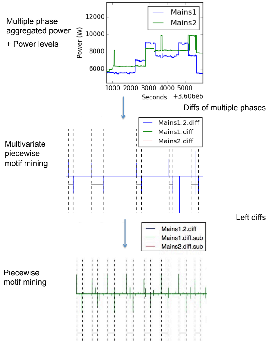
Figure 4.1: Recursive Multivariate Motif Mining Approach.
