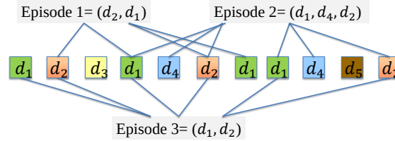
Figure 2.23: Motif Mining Example ([122]).
