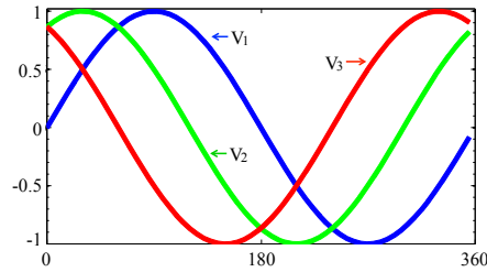
Figure 2.4: Three phase power waveform.
