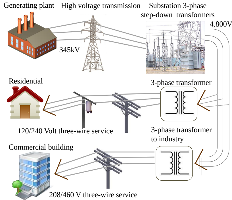
Figure 2.2: Electricity generation and transmission to residential and commercial buildings.
