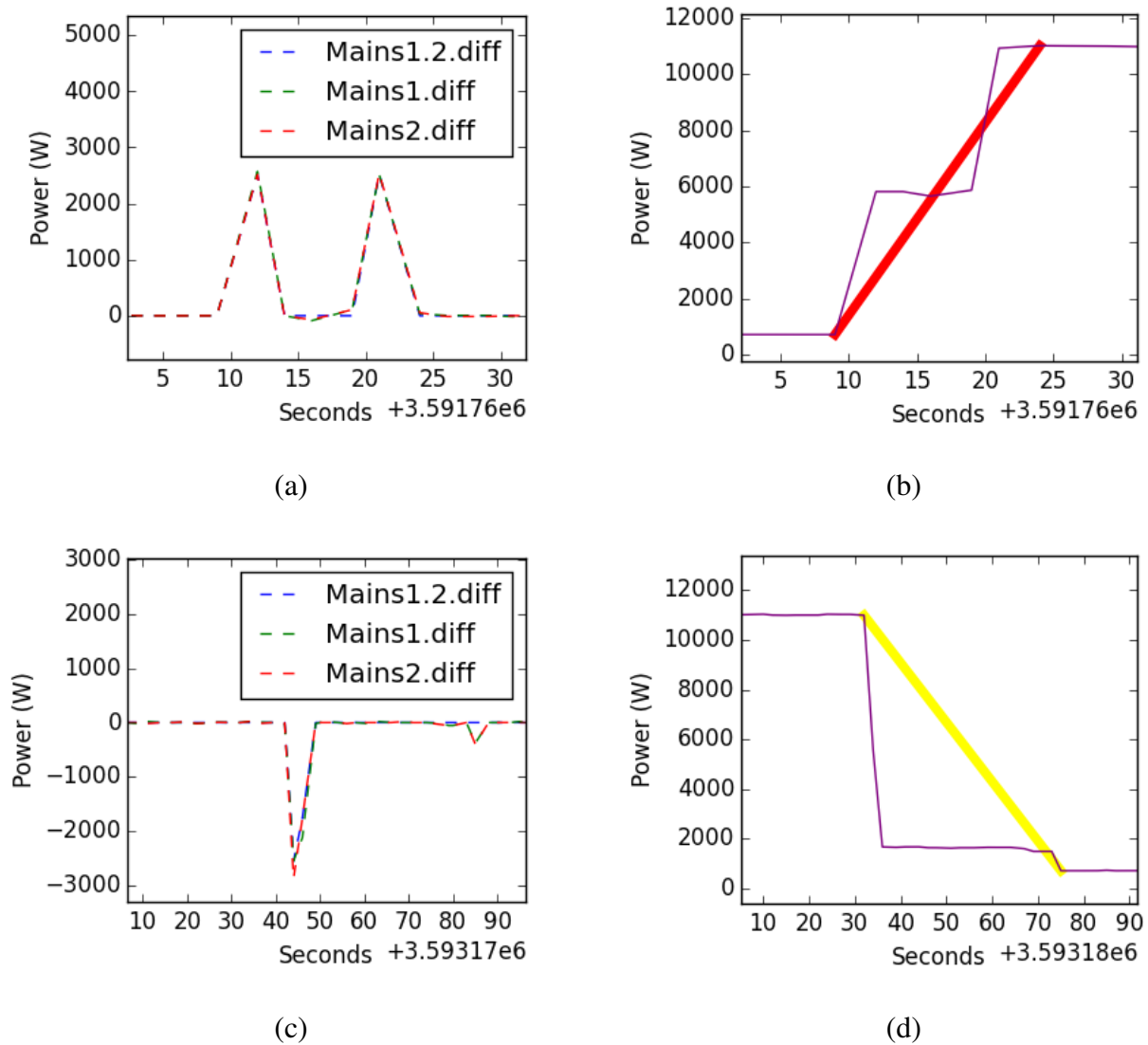
Figure 4.4: (a) On piecewise event and (c) Off piecewise event of heatingIndoor. heatingIndoor is disaggregated by motif mining the on event (b) and off event (d).
