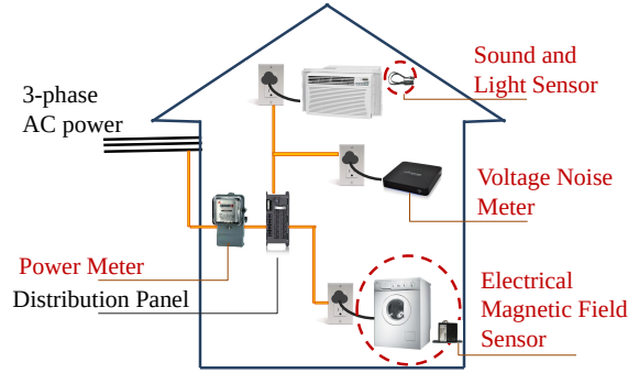
Figure 2.24: Four Types of Meters in a Building.
