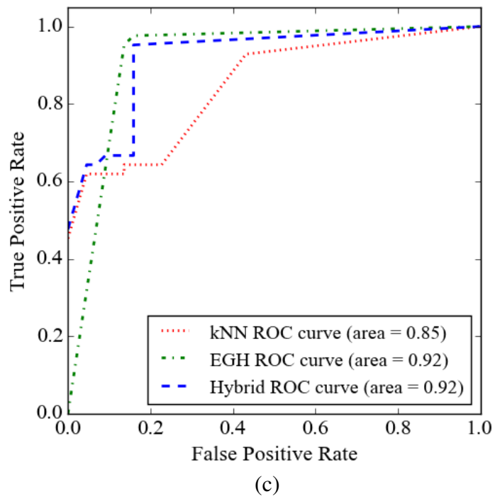
Figure 5.7: ROC curve of house occupancy prediction in (c) Study14 (12/20/2013).
