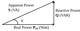
Figure 2.7: Power Triangle.
