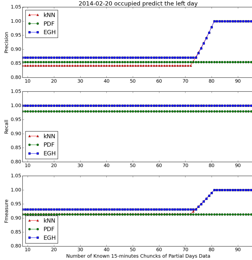
Figure 5.4: Occupancy prediction precision, recall and f-measure comparison of three approaches of person1 on 02/20/2014 on Study10.
