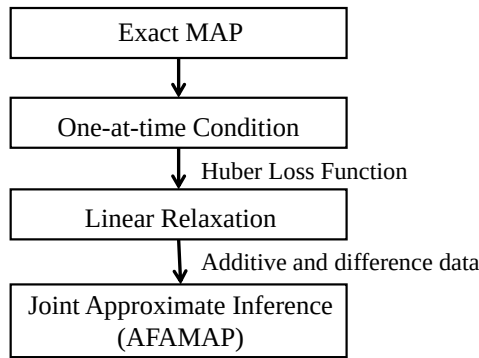
Figure 2.22: AFAMAP Flowchart.
