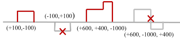
Figure 3.6: Episode constraints.
