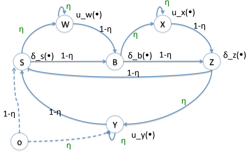
Figure 5.3: States Transition of Episode Generating HMM (EGH).
