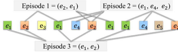
Figure 3.7: Illustration of motif mining. Note that there are 3 non-overlapped occurrences of Episode 3.
