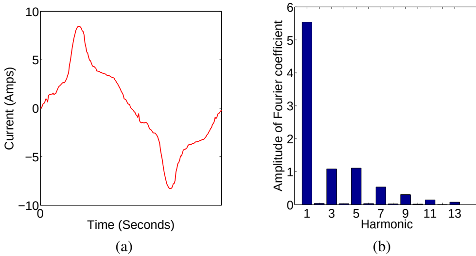
Figure 2.8: Circuit 4 (a) Current Waveform and (b) Harmonics.
