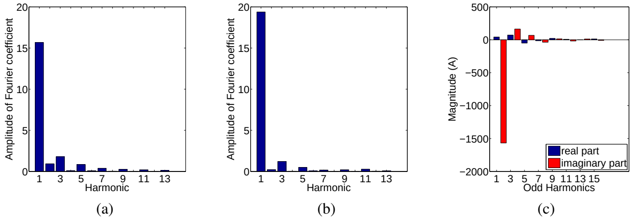
Figure 2.14: Harmonics Feature of (a) a refrigerator and (b) an air compressor (c) real and imaginary part of odd number of harmonics of a refrigerator.
