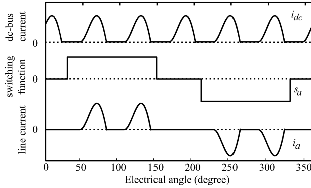
Figure 2.15: Switching-function for VSDs disaggregation (Courtesy:[140]).
