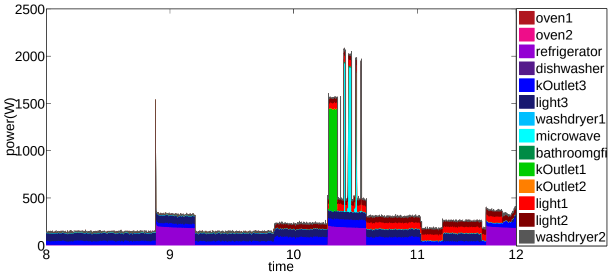
Figure 3.3: Example of energy disaggregation.
