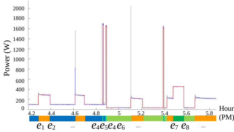
Figure 3.5: Mining episodes from a symbolic time series.
