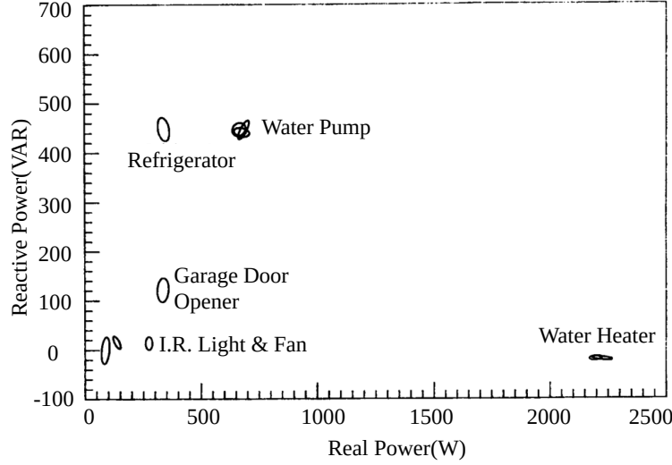
Figure 2.6: Real and reactive power for different devices (courtesy: [55]).
