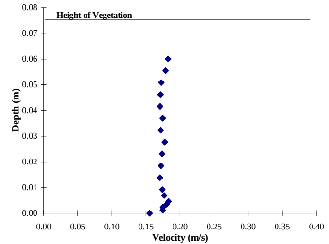
Figure A5: Velocity Profiles for Linear Formation of 76.2 mm Rods with s/d = 8 (Unsubmerged case)
