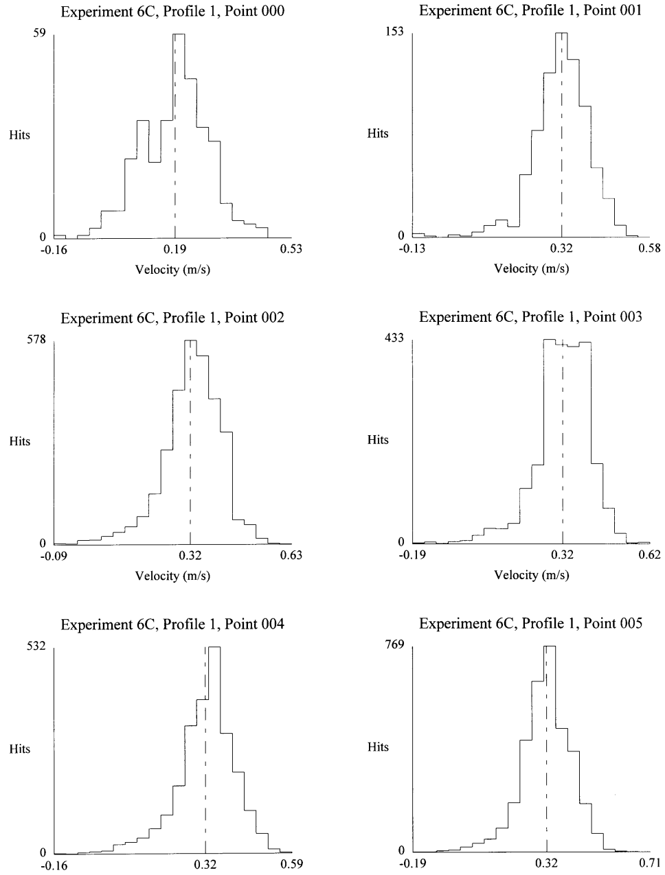
Figure A9: Histograms for Experiment 6C (Linear s/d=16 ), Profile 1
