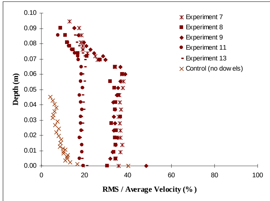
Figure 6.24 Turbulence Intensities for the Profiles of Experiments 7-13 (Double-Layered Vegetation Experiments @ 12 Dowel Diameters[76.2mm] DS)
