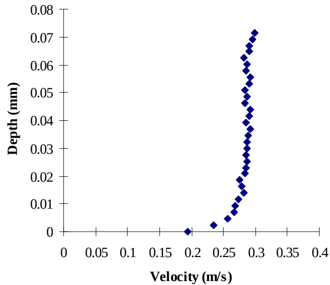
Figure 5.4. Typical logarithmic velocity profile taken during a control run
