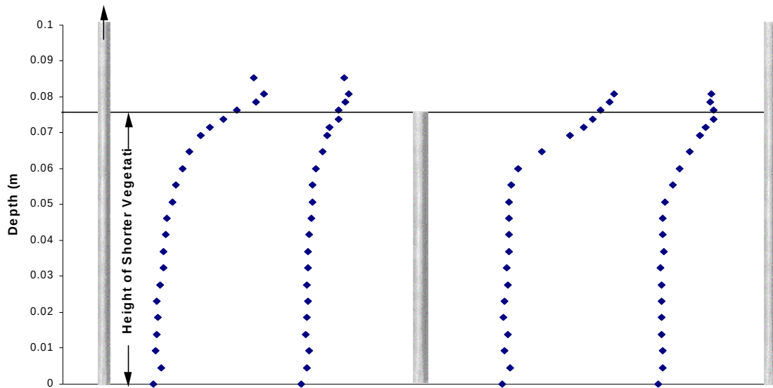
Figure 6.18: Progression of Velocity Profiles DS in Experiment 13 (Inline w/dowels)
