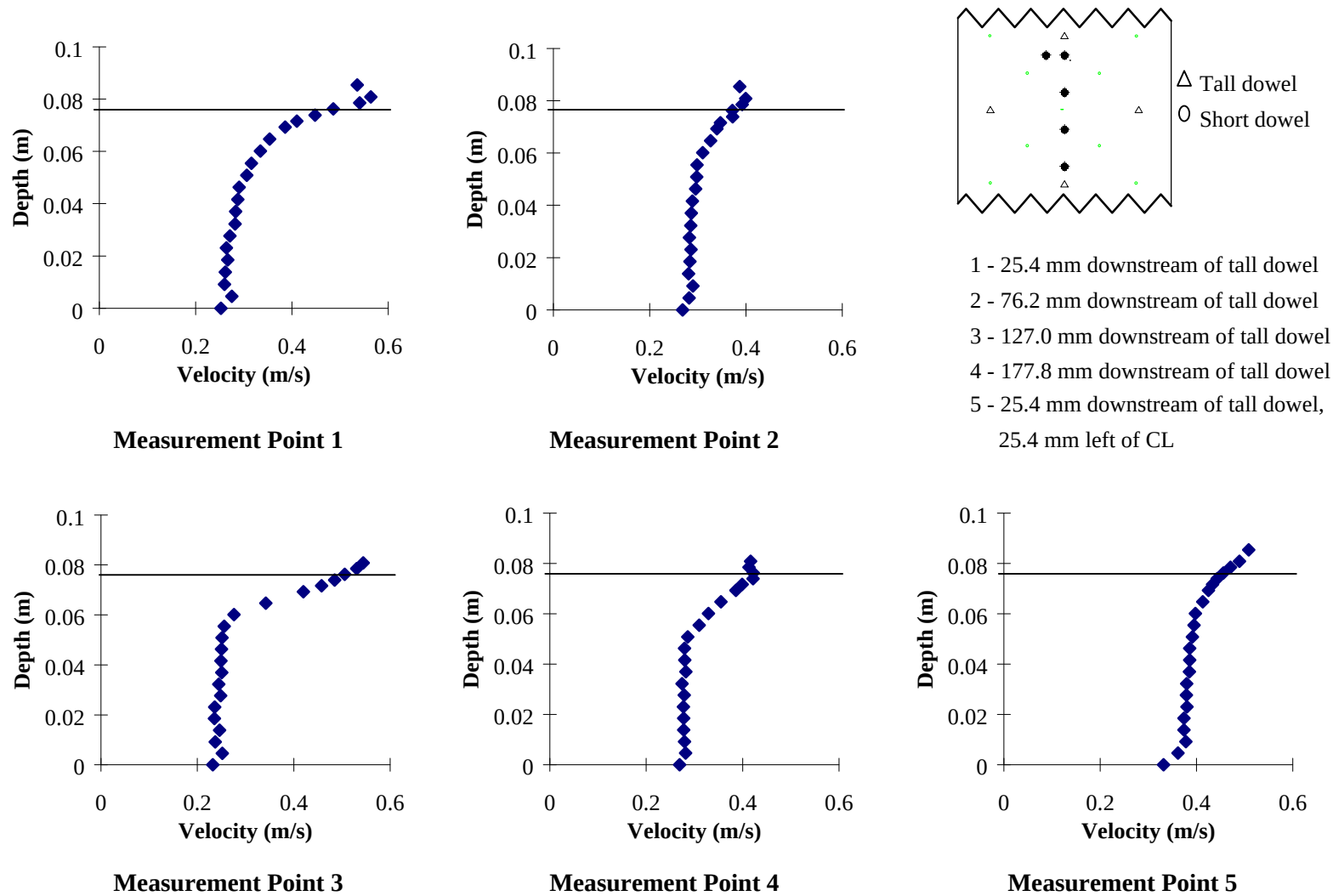
Figure A18: Profiles for Double-layered Experiment 13 (Staggered s/d=8 Short, Staggered s/d = 16 Tall)
