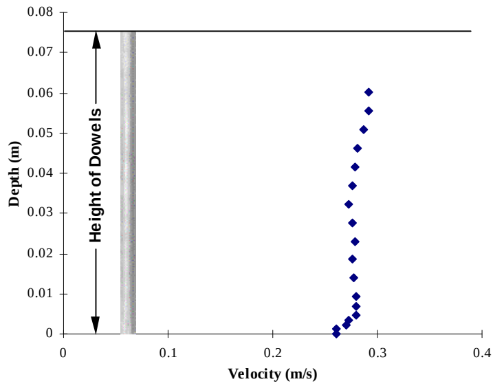
Figure 6.8: Velocity Profile from Experiment 5A (Linear s/d=8 )—Point 3 @ 6 Dowel Diameters DS (38.1 mm)
