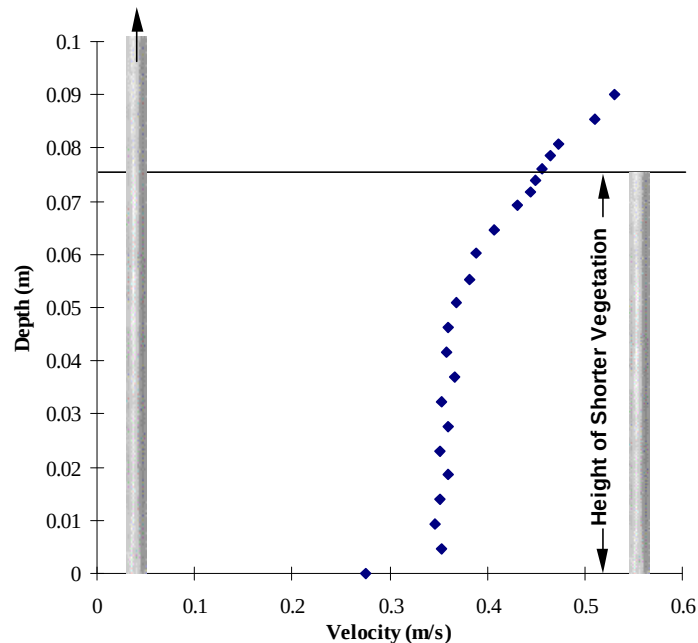
Figure 6.20: Velocity Profile from Experiment 9 [Linear s/d=8 (short), Linear s/d=16 (tall)] — Point 3 @ 4 Dowel Diameters (25.4 mm) DS, 4 Left of Centerline
