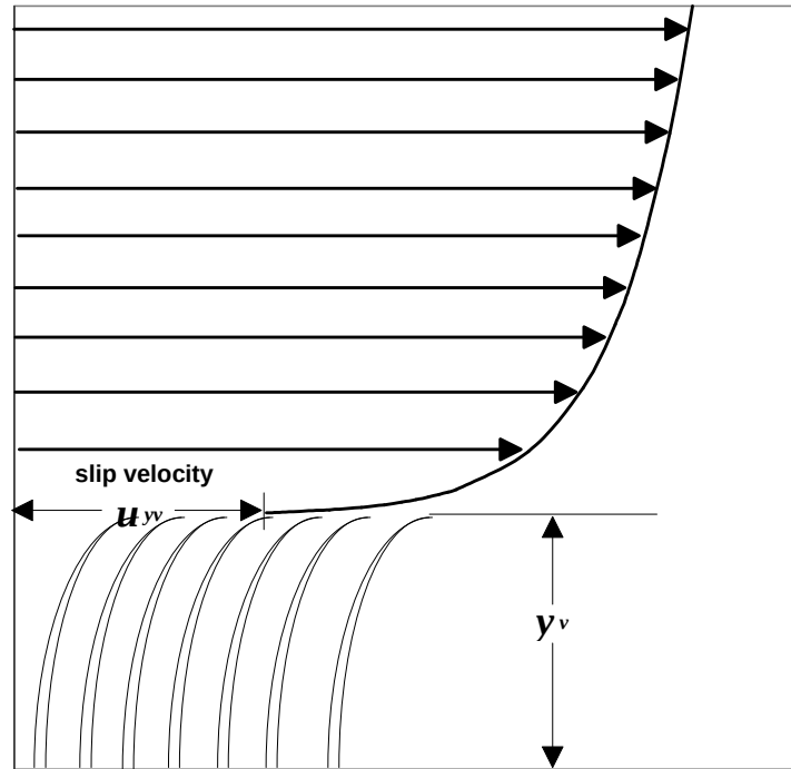
Figure 2.2: Velocity profile over vegetative layer.
