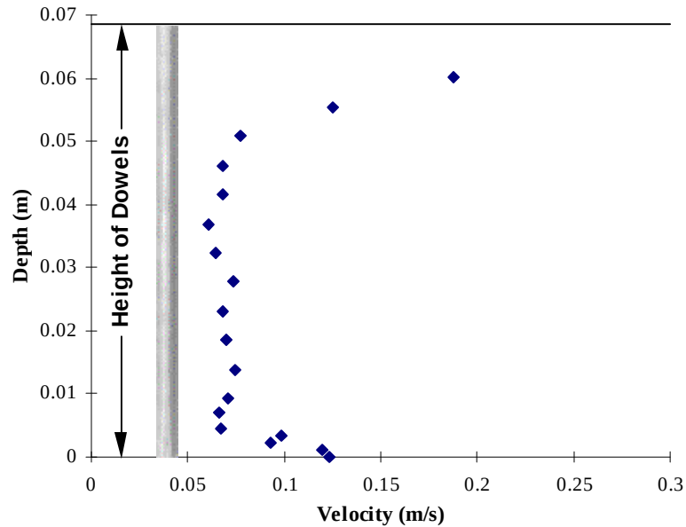
Figure 6.1: Velocity Profile from Experiment 5A (Linear s/d=8 ) — Profile 1 @ 2 Dowel Diameters DS (12.7 mm)
