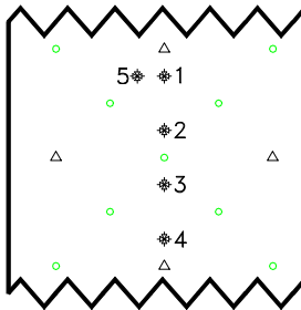
Measurement locations of Experiment 13 for short staggered s/d = 8 , tall staggered s_t/d = 16
