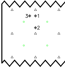
Measurement locations of Experiment 11 for short staggered s/d = 8 , tall linear s_t/d = 16
