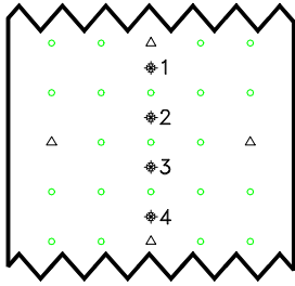
Measurement locations of Experiment 7 for short linear s/d = 8 , tall staggered s_t/d = 16
