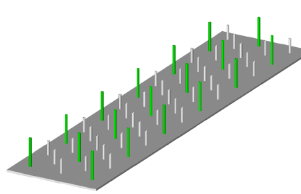
Measurement locations of Experiment 13 for short staggered s/d = 8 , tall staggered s_t/d = 16
