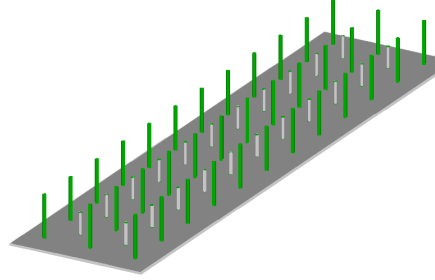
Measurement locations of Experiment 11 for short staggered s/d = 8 , tall linear s_t/d = 16
