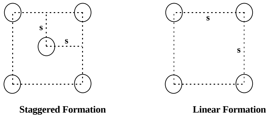
Figure 5.5: Definition of staggered and linear formations used in experiments.
