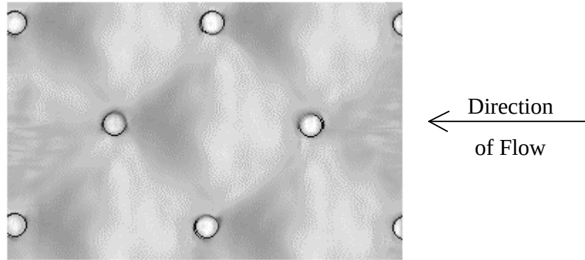
Figure 6.2: Surface wave formation found in staggered array of cylinders
