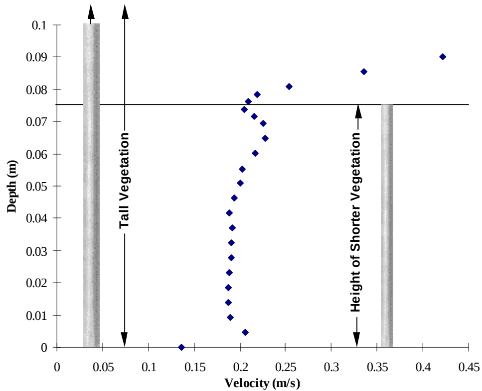
Figure 6.15: Velocity Profile from Experiment 9 [Linear s/d=8 (short), Linear s/d=16 (tall)] — Point 1 @ 4 Dowel Diameters (25.4 mm) DS from Tall Rod
