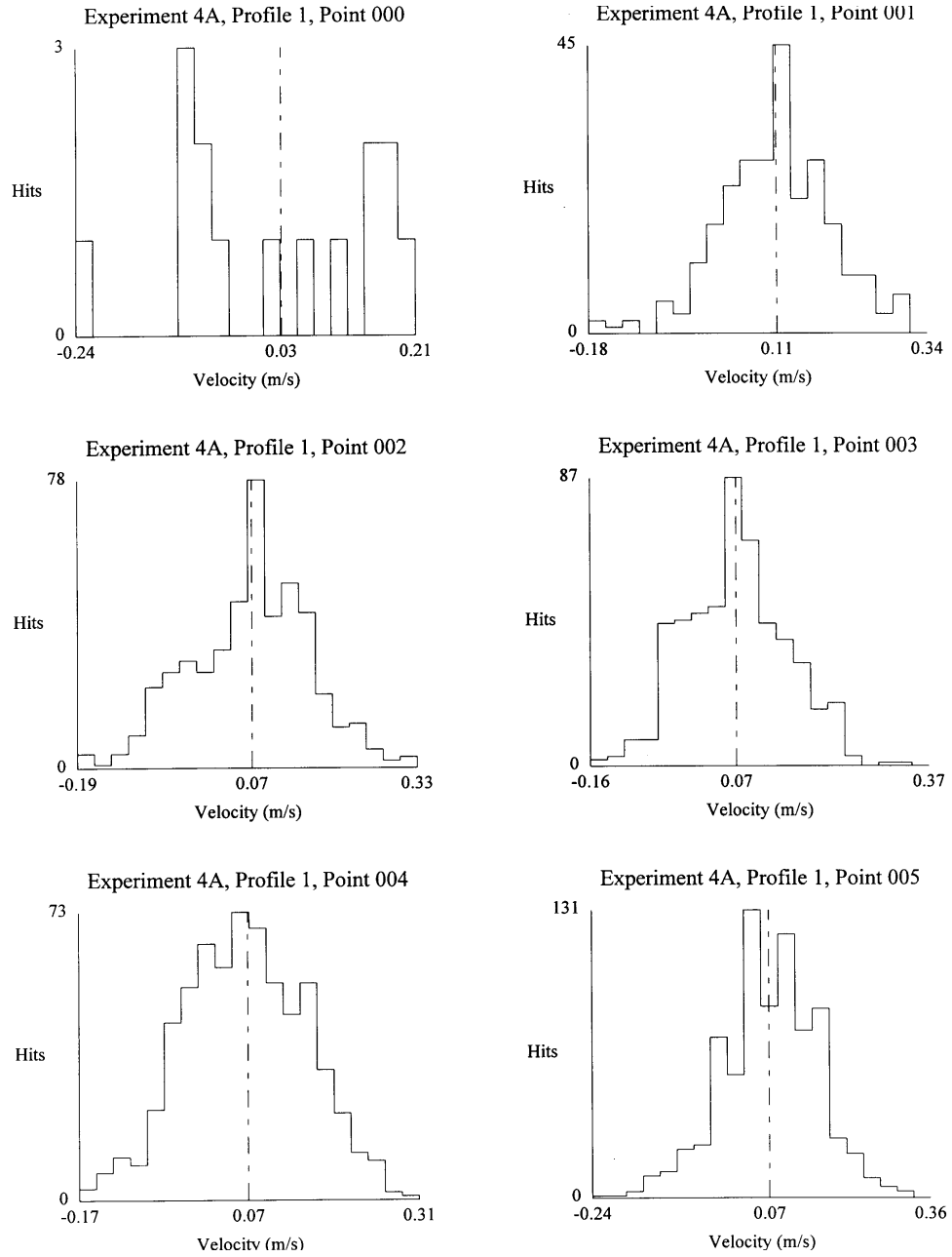
Figure A2: Histograms for Experiment 4A (Staggered s/d=8 ), Profile 1
