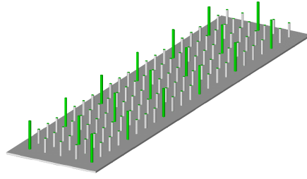
Measurement locations of Experiment 7 for short linear s/d = 8 , tall staggered s_t/d = 16
