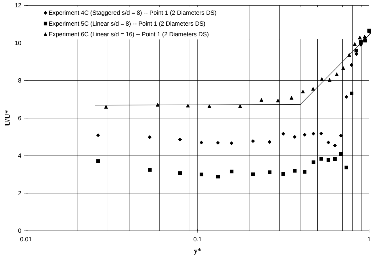
Figure 6.7: Dimensionless Plots of Submerged Experiments In-line with Dowels (Profiles immediately downstream)
