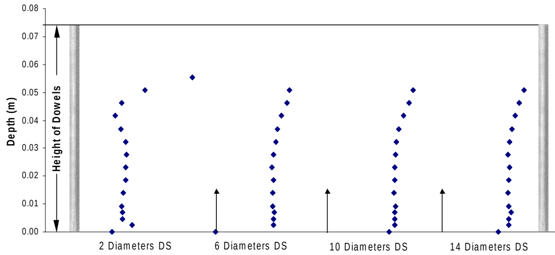
Figure 6.4: Progression of Velocity Profiles DS in Experiment 4A (Inline w/dowels) Staggered s/d=8
