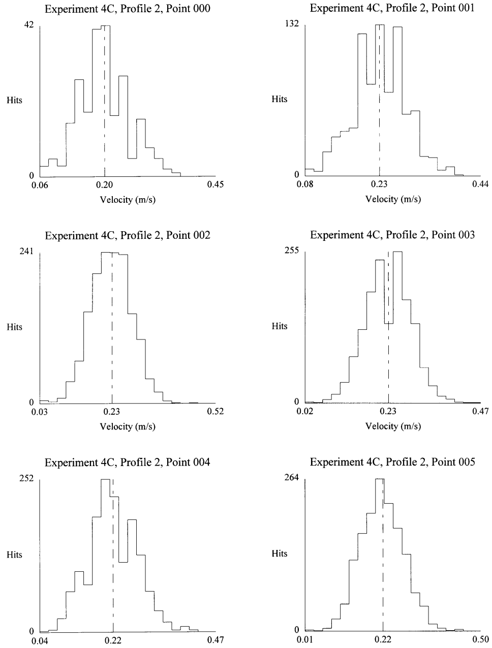
Figure A4: Histograms for Experiment 4C (Staggered s/d=8 ), Profile 2
