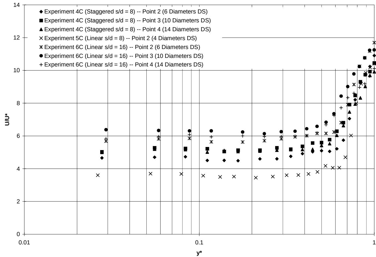
Figure 6.11: Dimensionless Plots of Submerged Experiments Inline with Dowels (Profiles immediately downstream of dowel are excluded)
