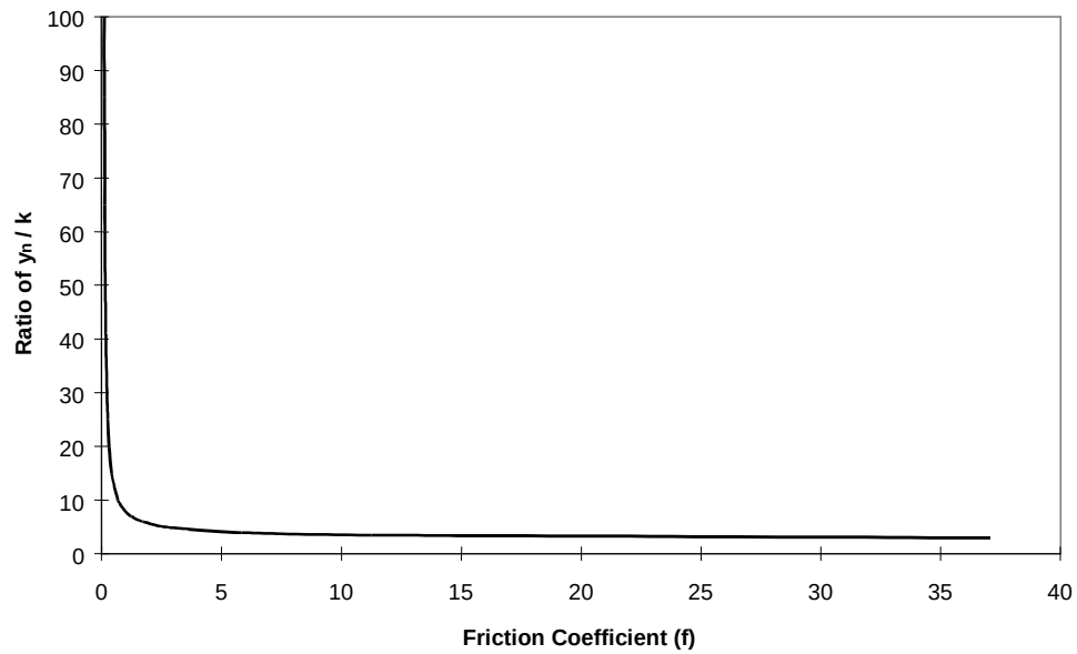
Figure 2.3. Plot of Equation 2.15 for Wide Rectangular Channel.
