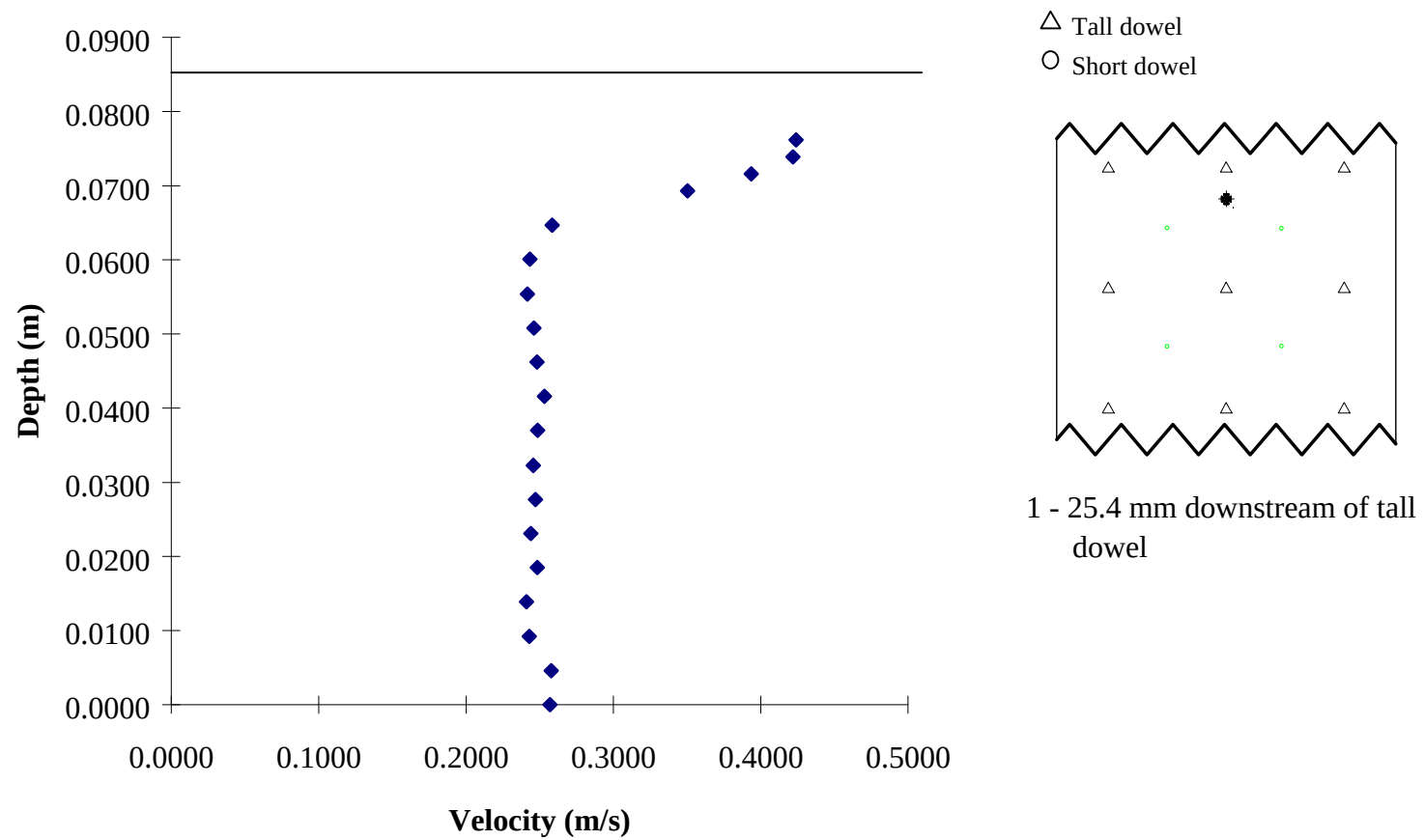
Figure A17: Profiles for Double-layered Experiment 12 (Staggered s/d=8 Short, Linear s/d = 16 Tall)
