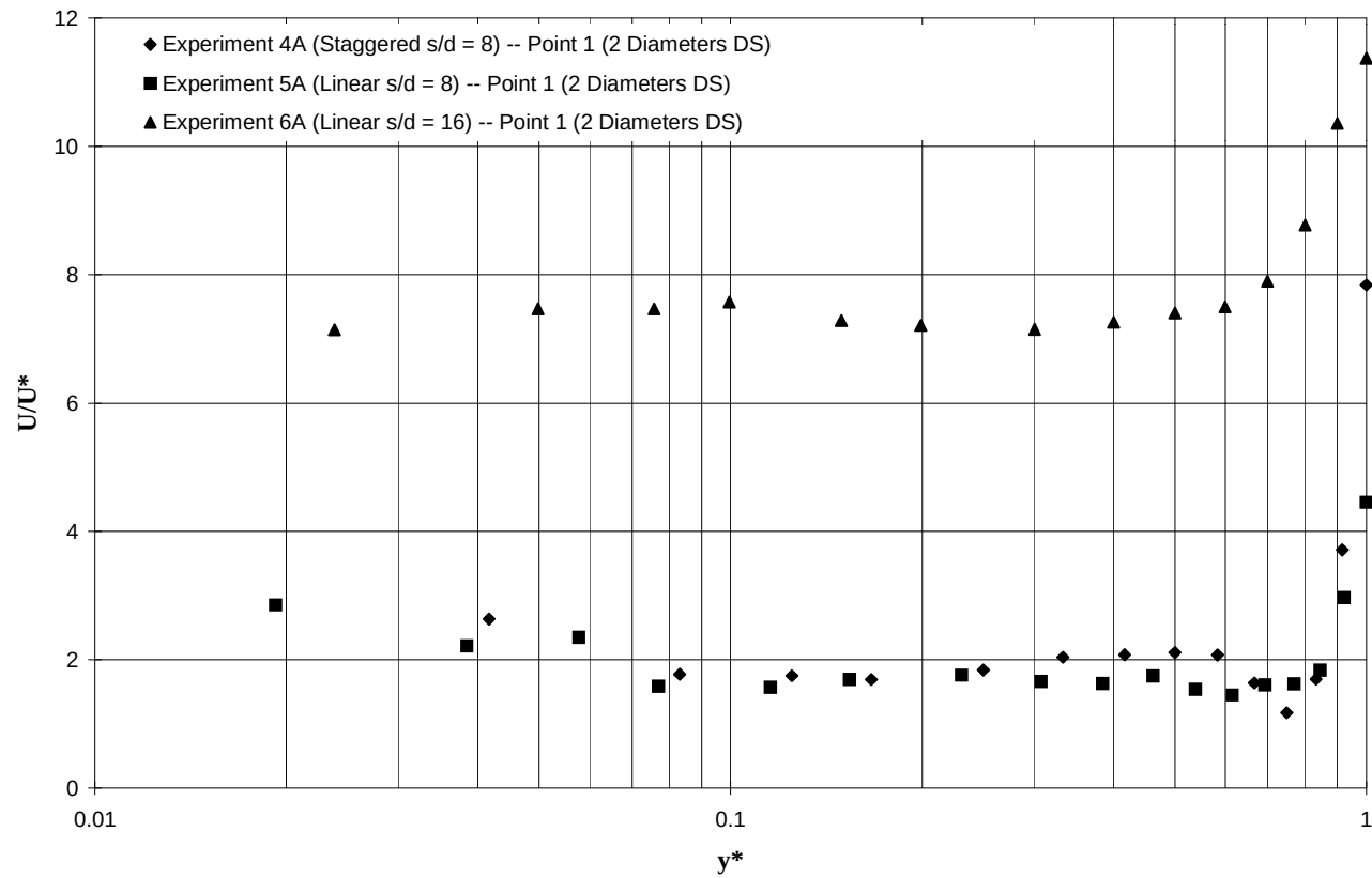
Figure 6.6: Dimensionless Plots of Unsubmerged Experiments In-Line with Dowels (Profiles immediately downstream).
