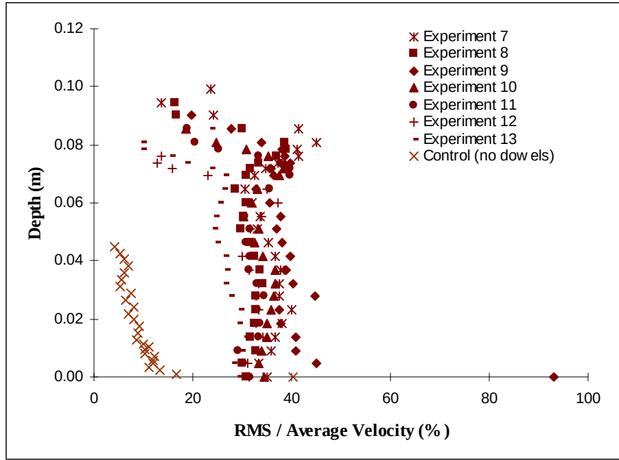
Figure 6.23: Turbulence Intensities for the Profiles of Experiments 7-13 (Double-Layered Vegetation Experiments @ 4 Dowel Diameters [25.4mm] DS)
