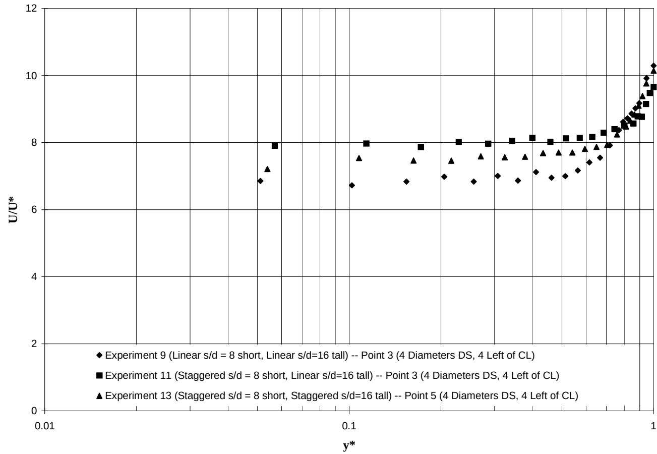
Figure 6.21: Dimensionless Plots of Double Layer Experiments in Unobstructed Locations
