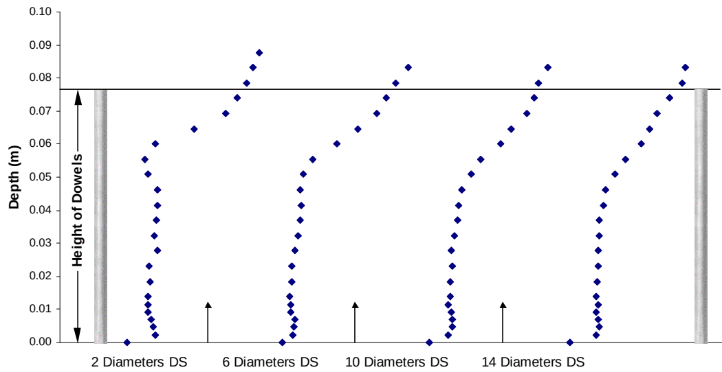
Figure 6.5: Progression of Velocity Profiles DS in Experiment 4C (Inline w/dowels) Staggered s/d=8
