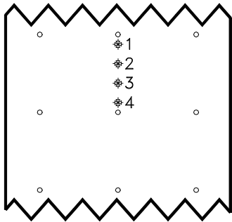
Measurement locations of Experiment 6c for linear s/d = 16
