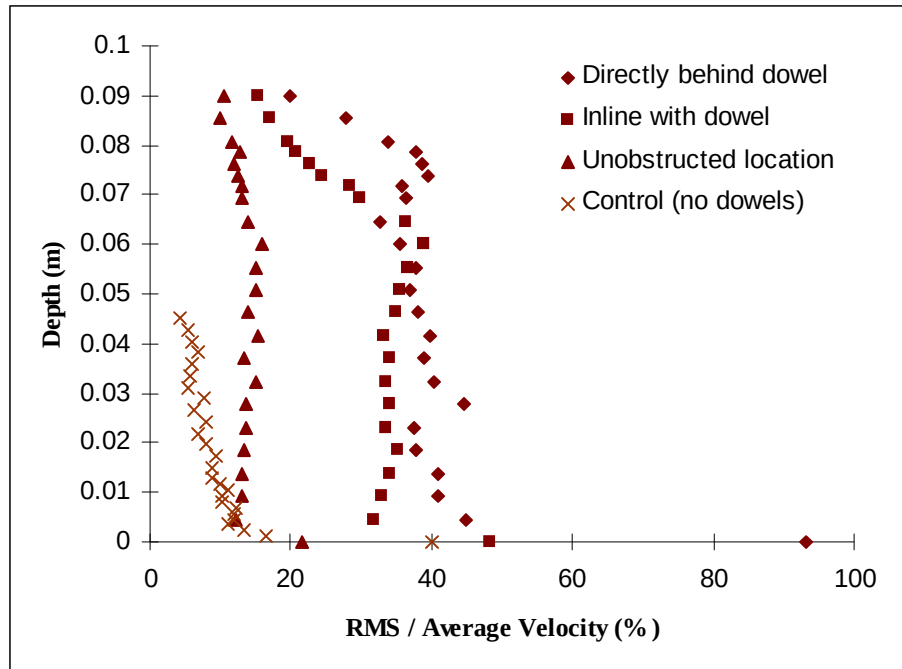
Figure 6.22: Turbulence Intensities for the Profiles of Experiment 9
