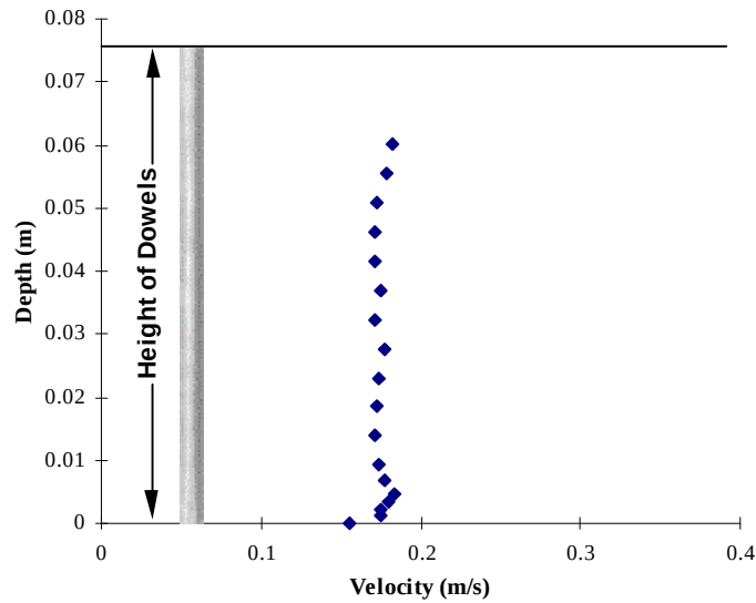
Figure 6.13: Velocity Profile from Experiment 5A (Linear s/d=8 ) — Point 4 @ 4 Dowel Diameters DS (25.4 mm) & 4 Dowel Diameters Left of Center
