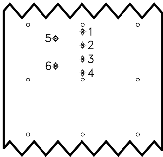
Measurement locations of Experiment 6a for linear s/d = 16
