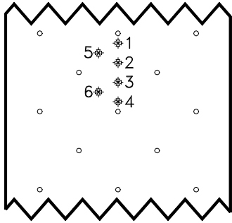
Measurement locations of Experiment 4a for staggered s/d = 8
