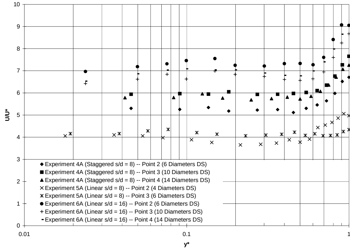
Figure 6.10: Dimensionless Plots of Unsubmerged Experiments Inline with Dowels (Profiles immediately downstream of dowel are excluded).
