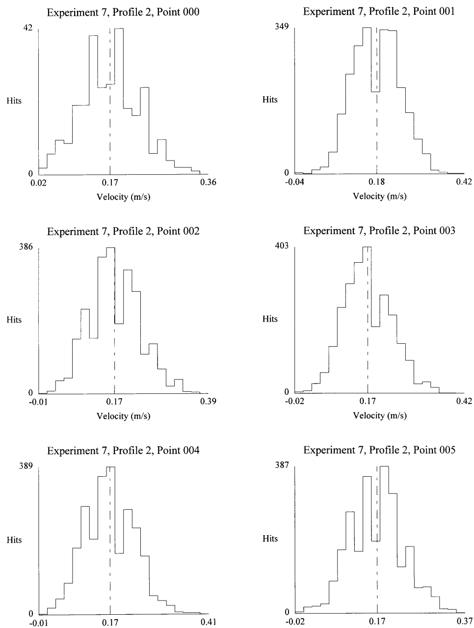
Figure A11: Histograms for Experiment 7 (Linear s/d=8 Short, Staggered s/d=16 Tall), Profile 2
