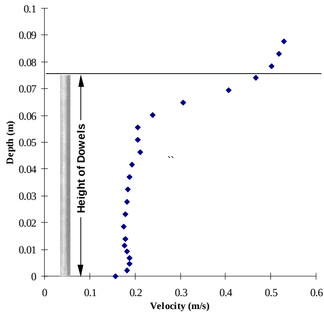
Figure 6.8: Velocity Profile from Experiment 5A (Linear s/d=8 )—Point 3 @ 6 Dowel Diameters DS (38.1 mm)
