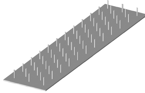
Measurement locations of Experiment 4a for staggered s/d = 8
