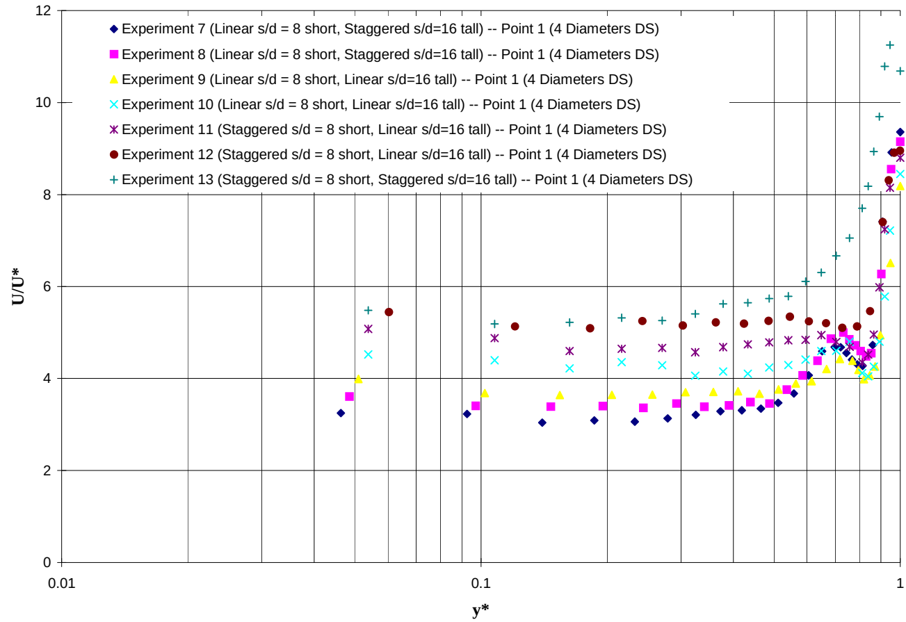
Figure 6.16: Dimensionless Plots of Double Layer Experiments Inline with Dowels (Points immediately downstream of dowels)
