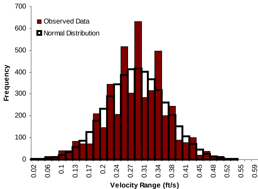
Figure 6.27: Experiment 13 Profile 1 Measurement Point 1
