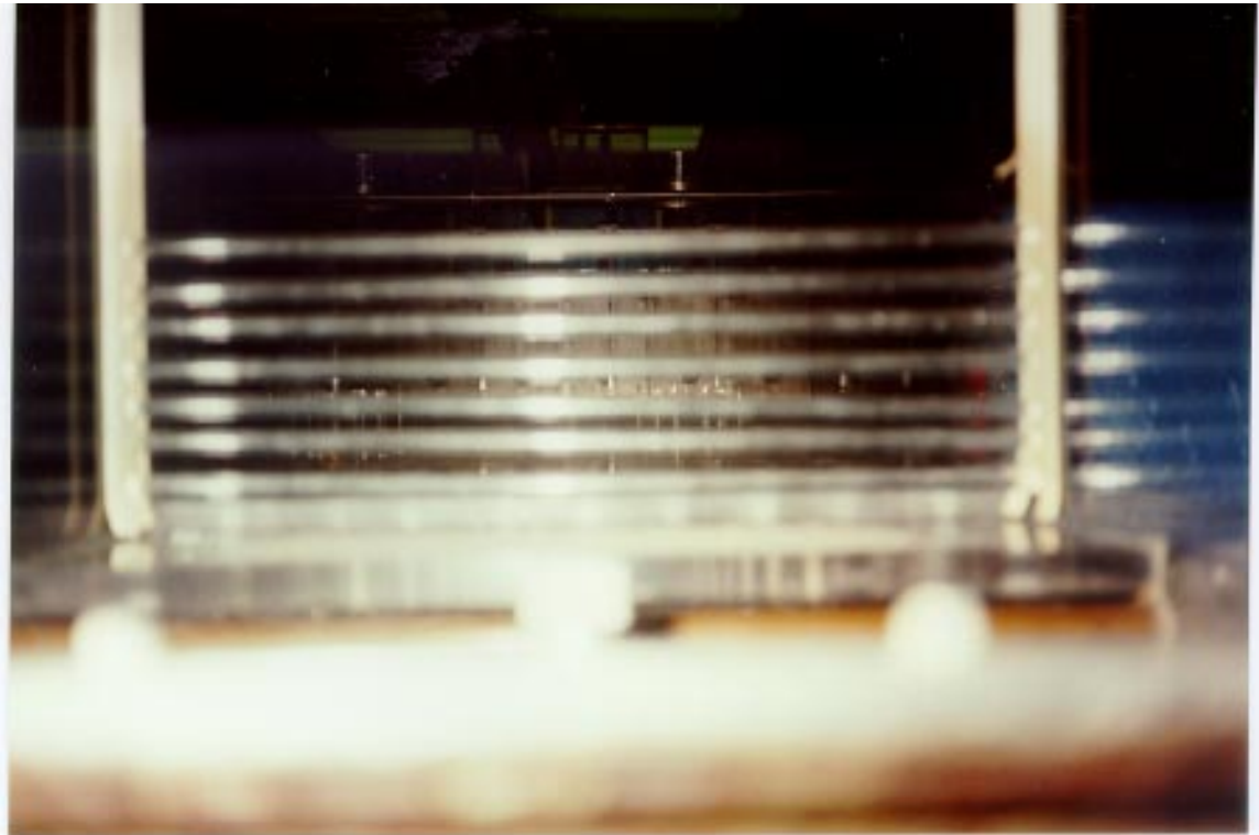
Figure 5.3 Photograph showing the placement of stop logs.
