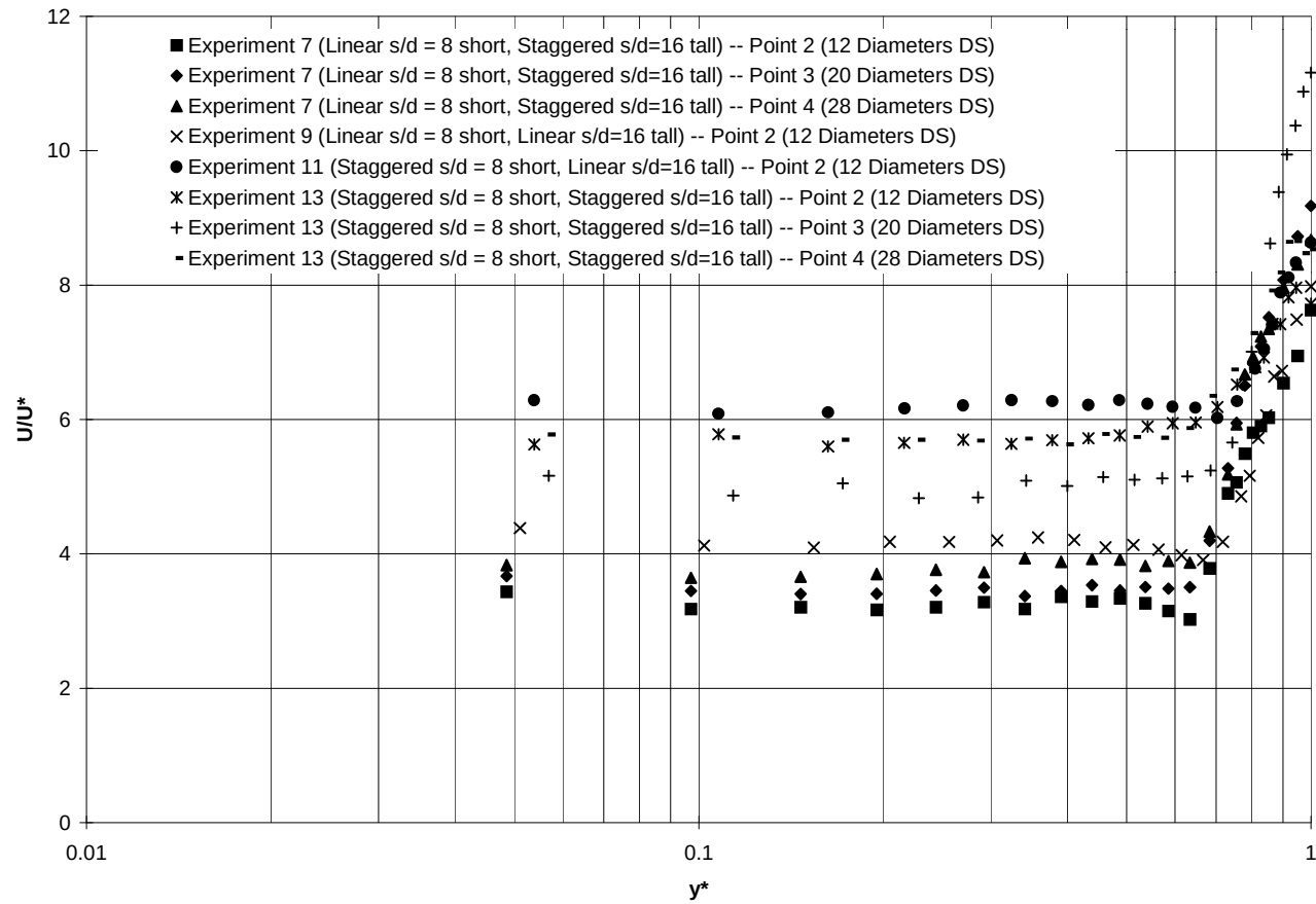
Figure 6.19: Dimensionless Plots of Double Layer Experiments Inline with Dowels (Profiles immediately downstream of dowel are excluded)
