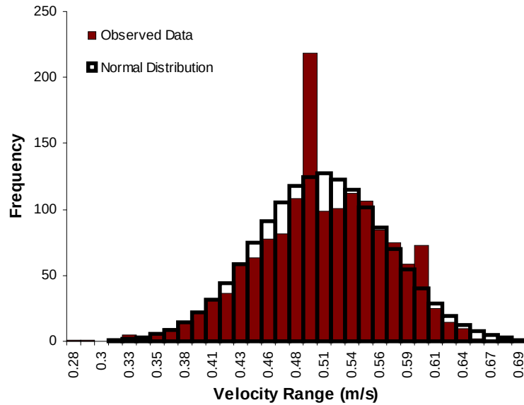
Figure 6.26: Experiment 11 Profile 2 Measurement Point 16
