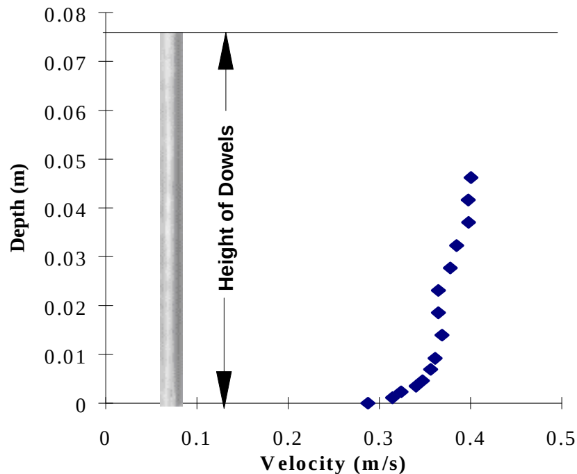
Figure 6.12: Velocity Profile from Experiment 6A (Linear s/d=16 ) — Point 5 @ 4 Dowel Diameters DS (25.4 mm) & 8 Dowel Diameters Left of Center
