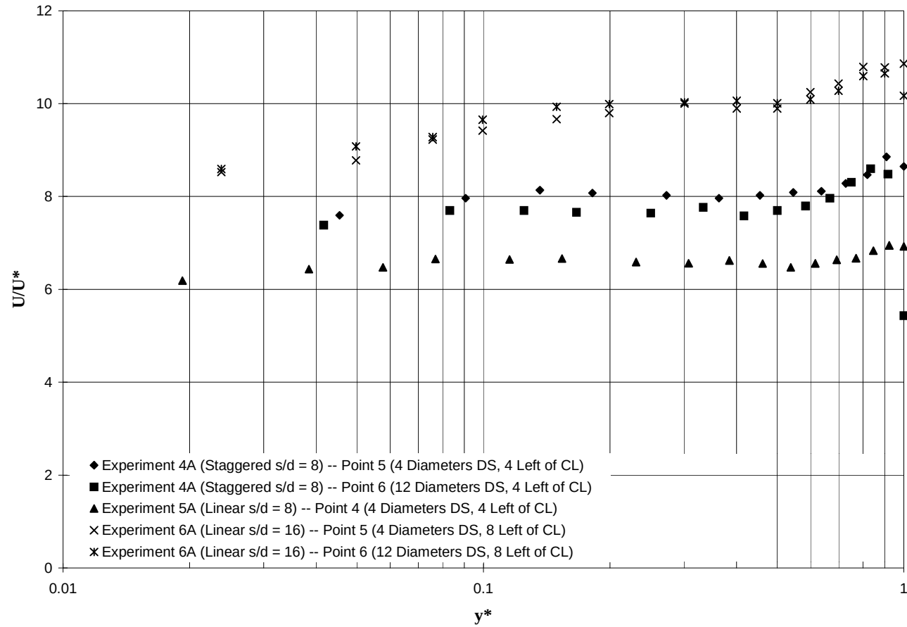
Figure 6.14: Dimensionless Plots of Unsubmerged Experiments in Unobstructed Location
