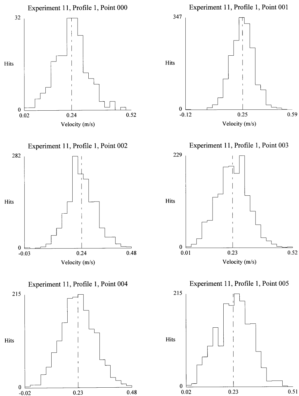
Figure A16: Histograms for Experiment 11 (Staggered s/d=8 Short, Linear s/d=16 Tall), Profile 1
