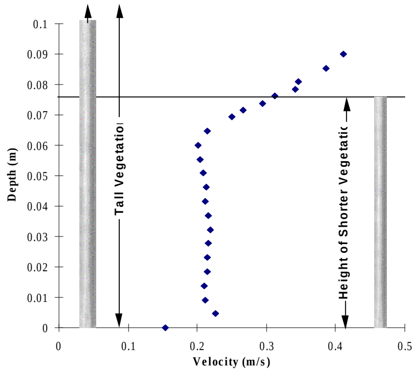
Figure 6.17: Velocity Profile from Experiment 9 [Linear s/d=8 (short), Linear s/d=16 (tall)] —Measurement Point 2 @ 12 Dowel Diameters (76.2 mm) from Tall Rod
