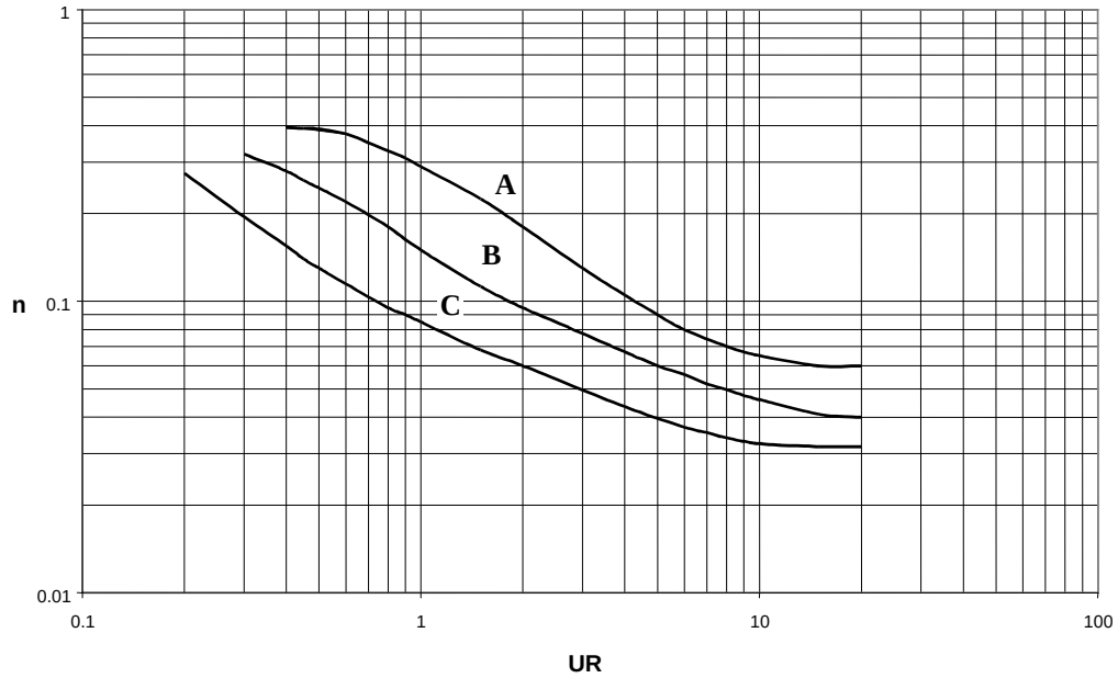
Figure 2.1: Plot of Manning's n as a function of UR for varying grass lengths.
