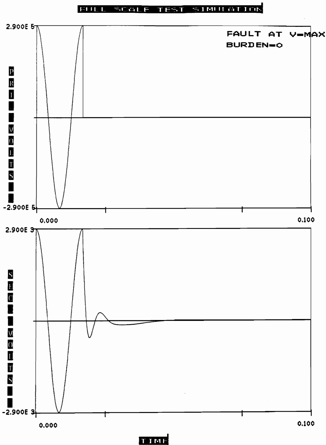
Figure 23. Simulation – fault at V = max and no burden
