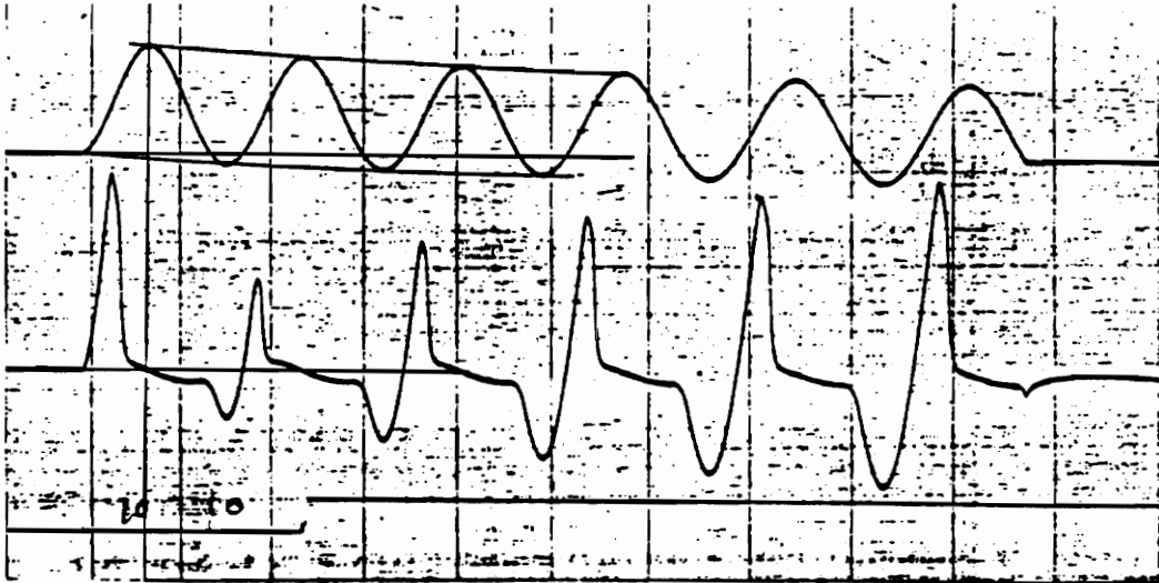
Figure 1. Waveforms of 150/5 ct subjected to 40 KA Primary current with offset
