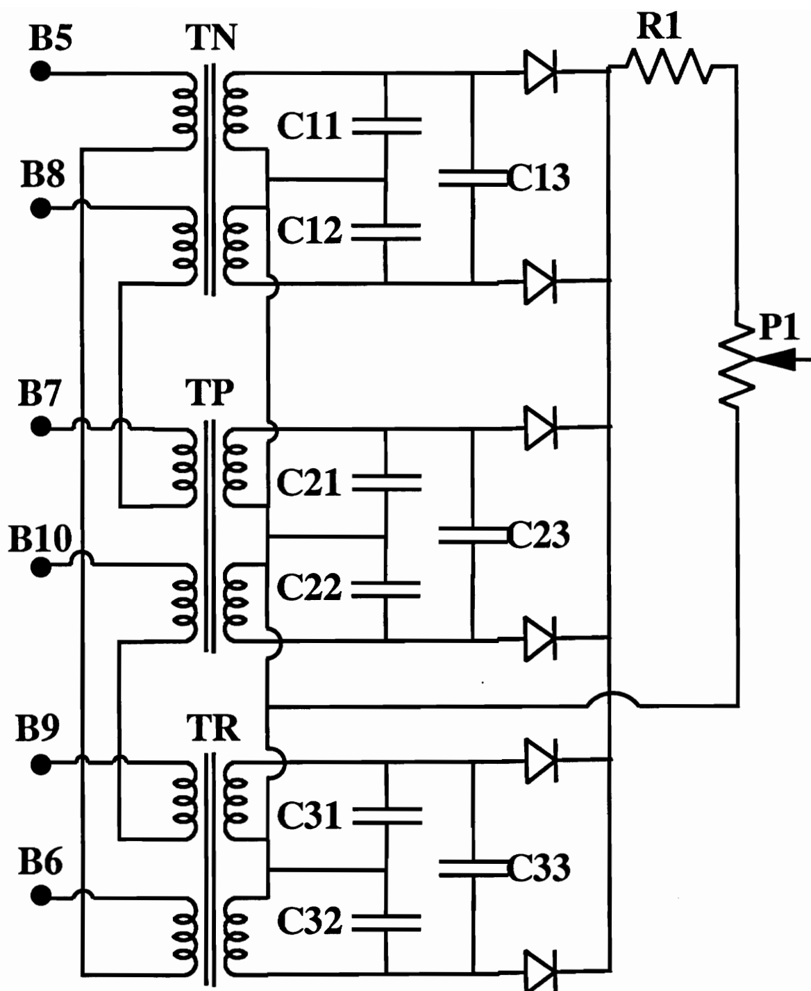
Figure 43. Auction circuit
