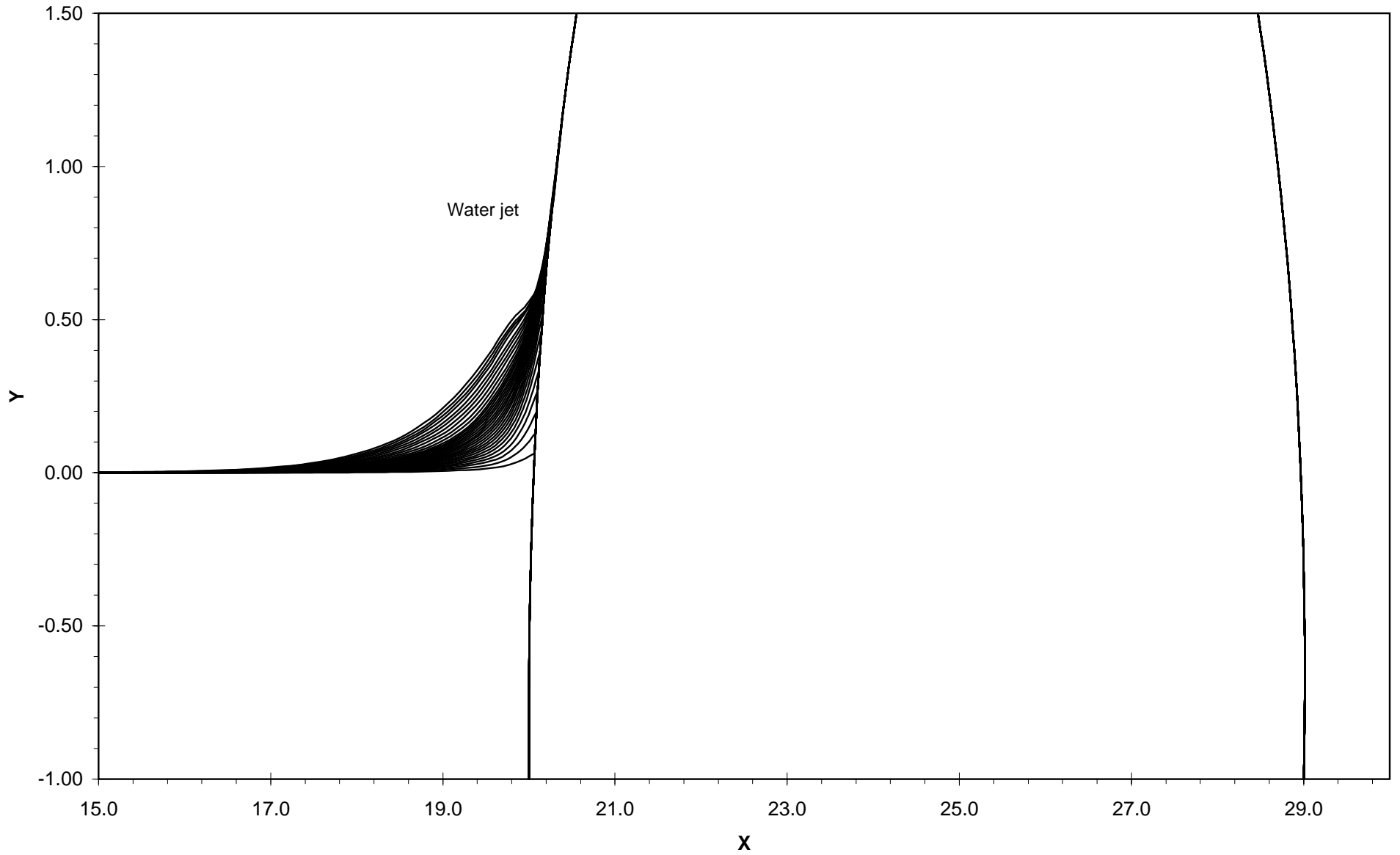
Figure I-7: Plot of the free surface profile for a tall rigid dam showing the formation of a jet of fluid at the solid surface.
