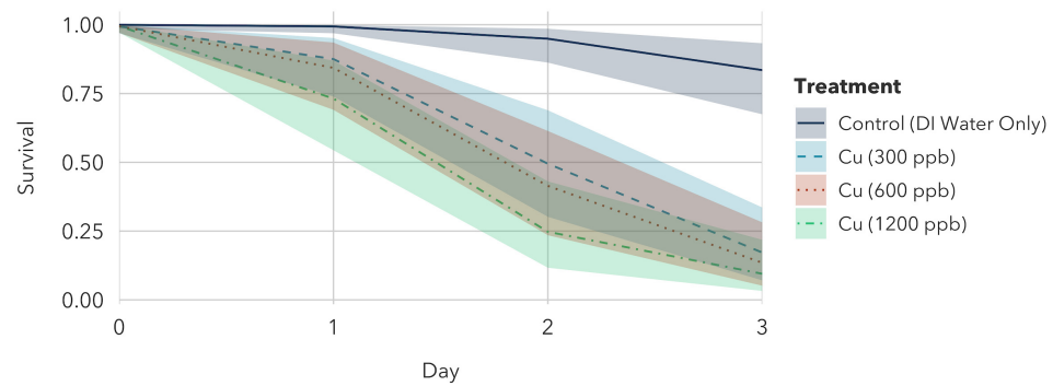
Figure 12. Predicted probabilities of survival of Ae. aegypti larvae in contact with copper sulfate pentahydrate concentrations of 300, 600, and 1200 \mu\text{g}/\text{L} Cu.
