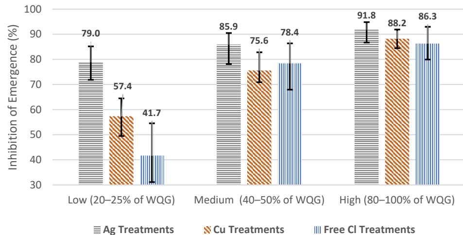
Figure 14. Summary of predicted probabilities of inhibition of emergence results regarding the efficacy of water disinfectants as larval control for older instar Ae. aegypti . IE% calculated from the model generated data from day 16. Error bars represent the 95% confidence interval.
