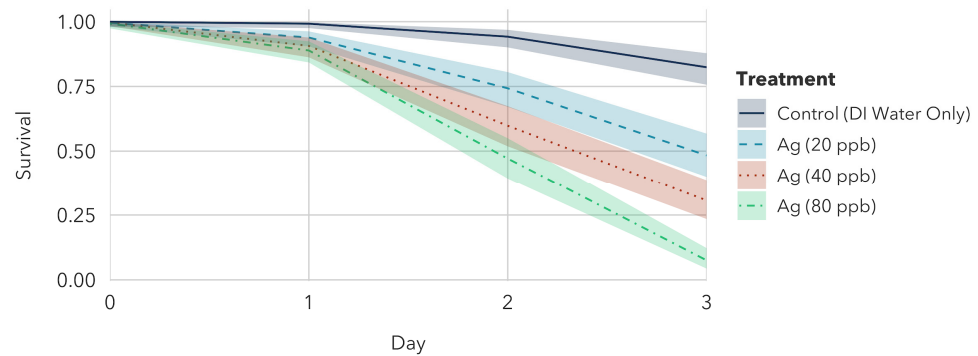
Figure 11. Predicted probabilities of survival of Ae. aegypti larvae in contact with silver nitrate concentrations of 20, 40, and 80 \mu\text{g}/\text{L} Ag.
