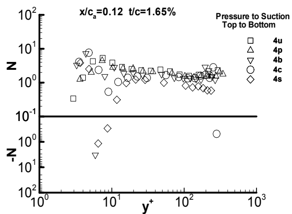
(g) x/c_a = 0.12 t/c = 1.65\%
