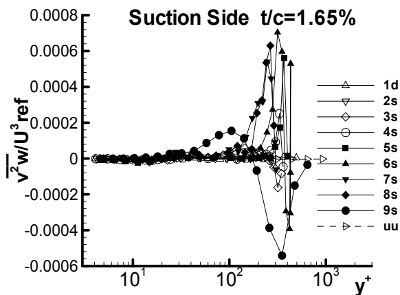
(c) Local Gap Inflow t/c = 1.65\%
