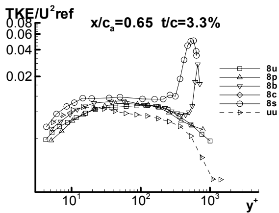
(p) x/c_a = 0.65 t/c = 3.30\%
