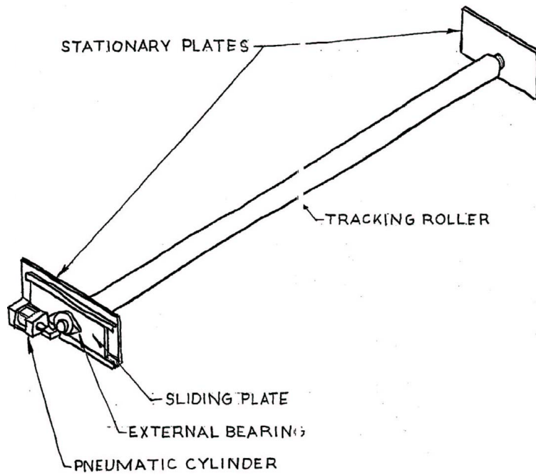
(a) Single Roller
