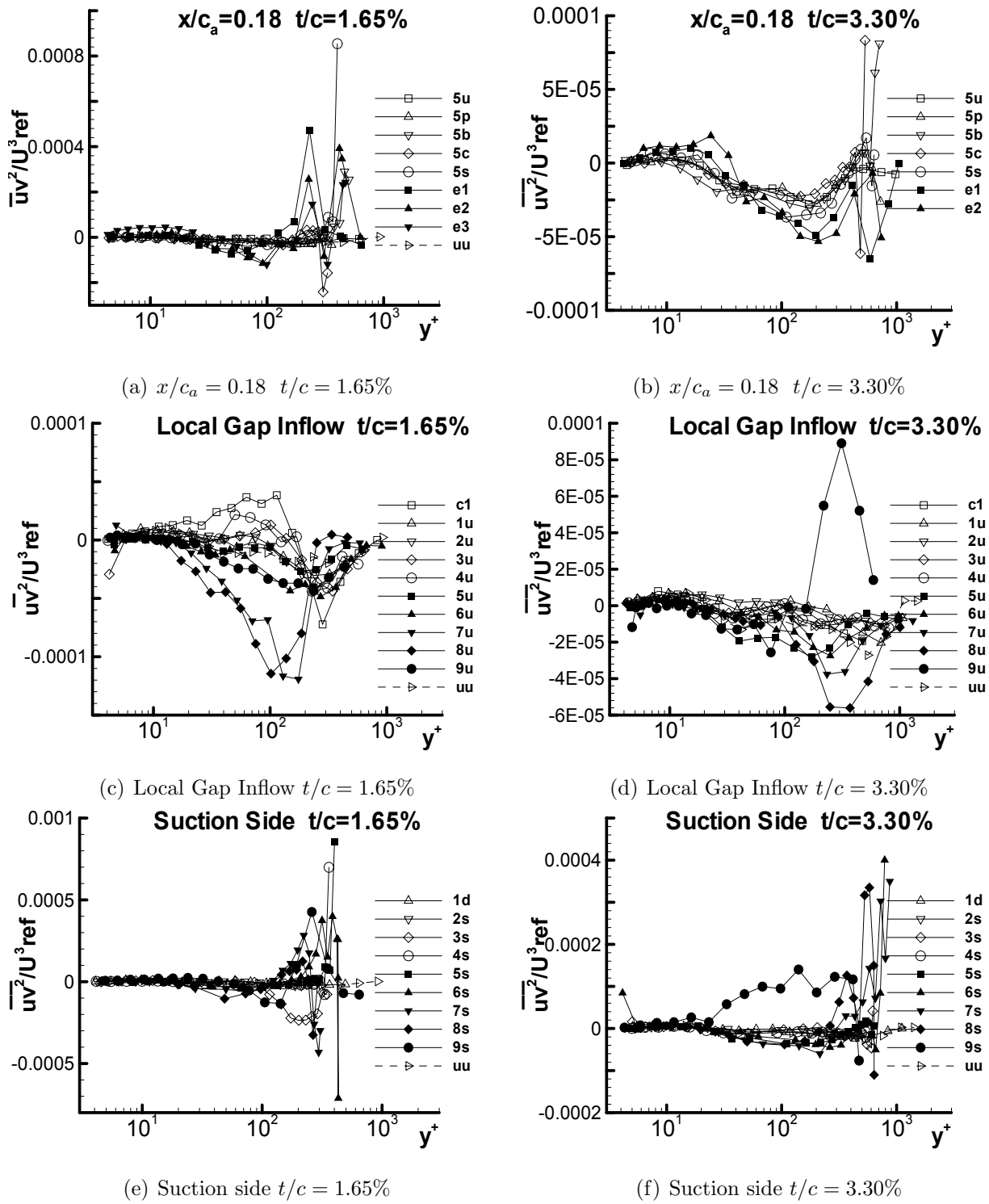
Figure 3.25: Triple product \overline{uv^2}/U^3_{ref} for both 1.65% and 3.30% in chord coordinate system
