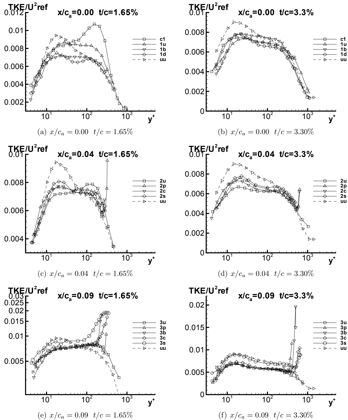
Figure H.7: TKE/U_{ref}^2 for both 1.65% and 3.30%
