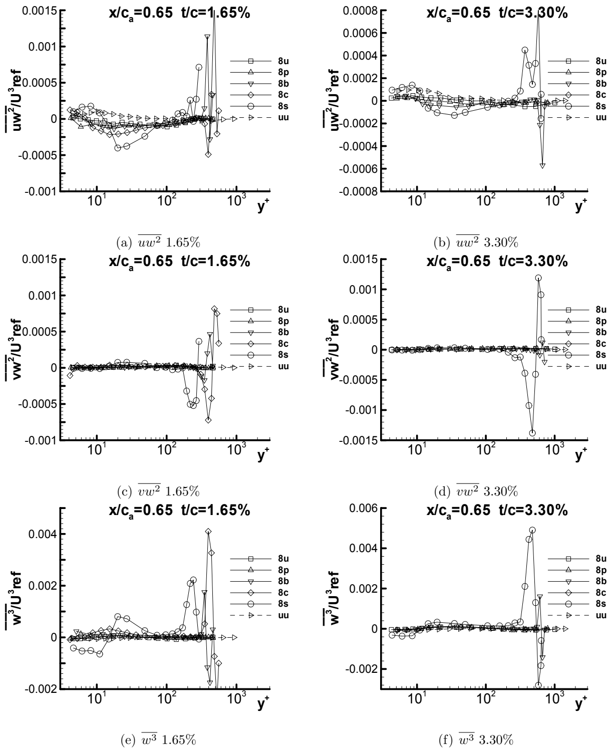
Figure G.26: Triple products \overline{uw^2}/U_{ref}^3 , \overline{vw^2}/U_{ref}^3 , and \overline{w^3}/U_{ref}^3 at x/c_a = 0.65 for both 1.65% and 3.30% in chord coordinate system
