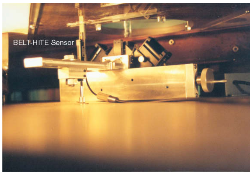
Figure 2.13: Assembly of LDV head and displacement sensor on the positioning plate and under the tunnel
