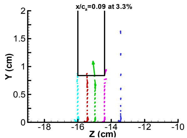
(f) x/c_a = 0.09 t/c = 3.30\%
