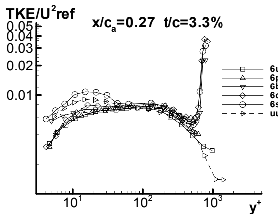
(l) x/c_a = 0.27 t/c = 3.30\%
