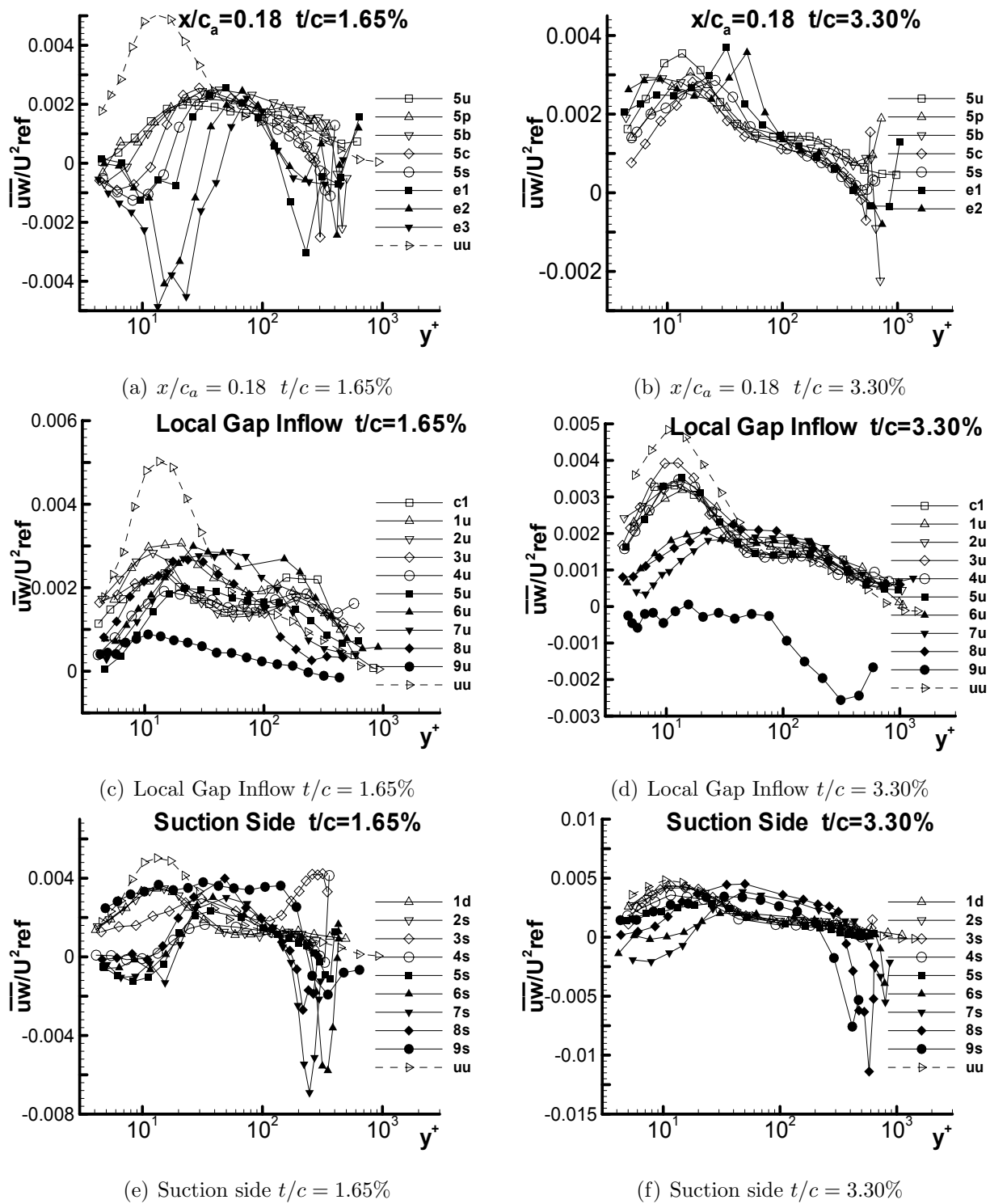
Figure 3.24: Shear stress -\overline{uw}/U^2_{ref} for both 1.65% and 3.30% in chord coordinate system
