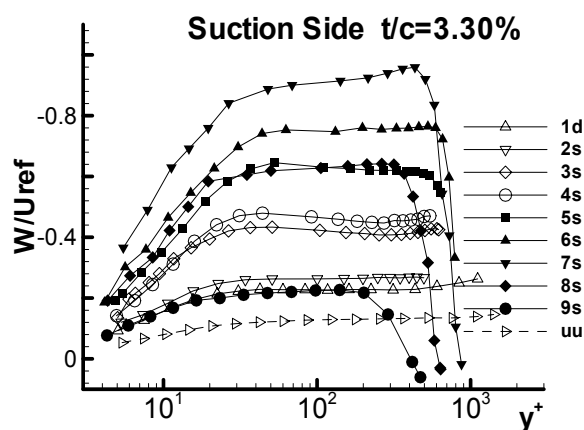
(f) Suction side t/c = 3.30\%
