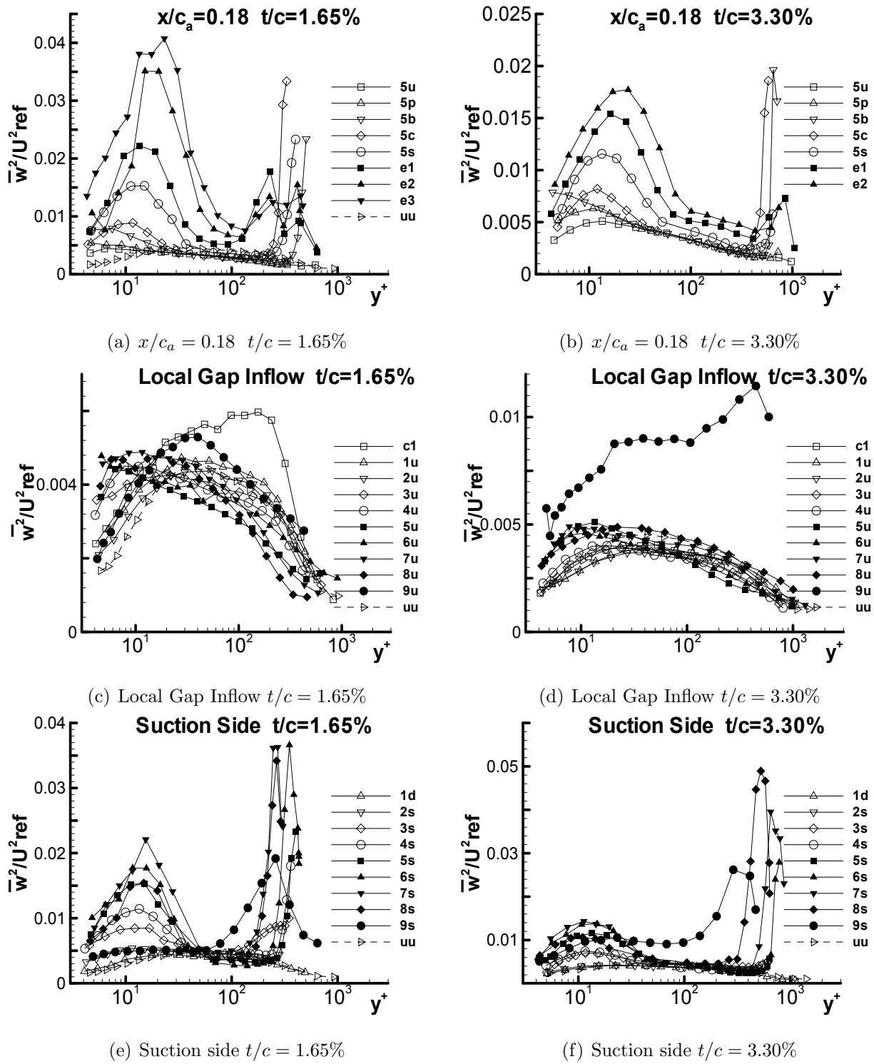
Figure 3.21: Normal stress \overline{w^2}/U^2_{ref} for both 1.65% and 3.30% in chord coordinate system
