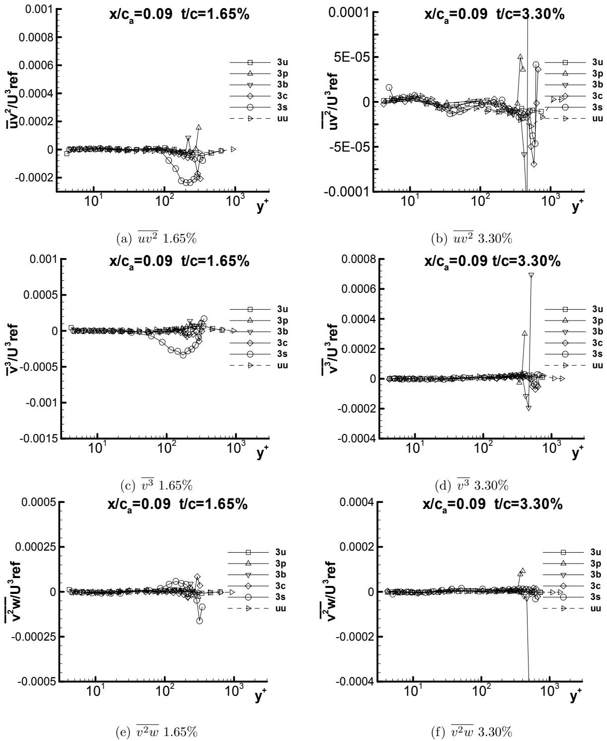
Figure G.3: Triple products \overline{uv^2}/U_{ref}^3 , \overline{v^3}/U_{ref}^3 , and \overline{v^2w}/U_{ref}^3 at x/c_a = 0.09 for both 1.65% and 3.30% in chord coordinate system
