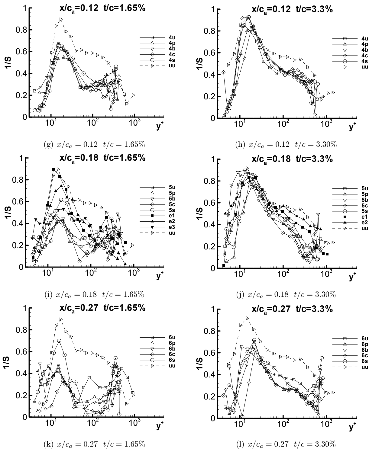
Figure H.13: 1/S for both 1.65% and 3.30% (cont.)
