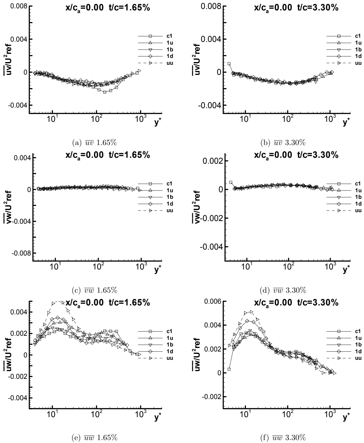
Figure F.10: Reynolds shear stresses -\overline{uv}/U^2_{ref} , -\overline{vw}/U^2_{ref} , and -\overline{uw}/U^2_{ref} at x/c_a = 0.00 for both 1.65% and 3.30% in chord coordinate system
