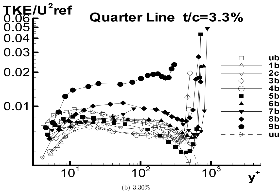
Figure H.9: TKE/U_{ref}^2 underneath quarter line of the blade from the pressure side for both 1.65% and 3.30%
