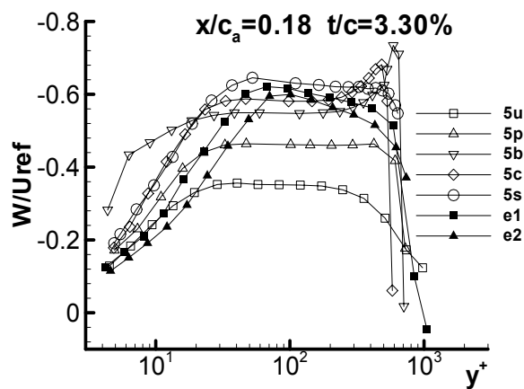
(b) x/c_a = 0.18 t/c = 3.30\%
