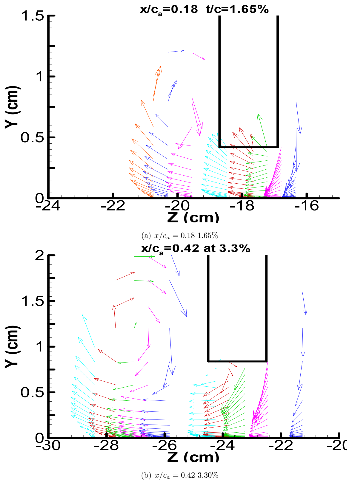
Figure 3.52: VW vector plots at x/c_a = 0.18 with 1.65% and x/c_a = 0.42 with 3.30% in the separation-line coordinate system
