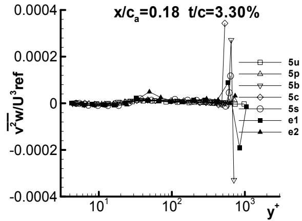
(b) x/c_a = 0.18 \quad t/c = 3.30\%
