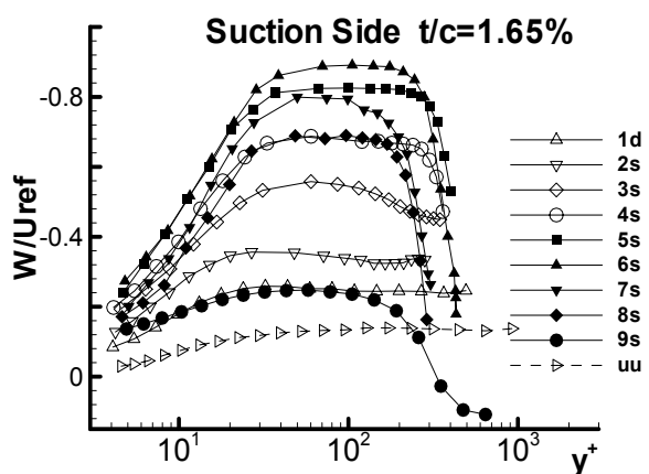
(e) Suction side t/c = 1.65\%
