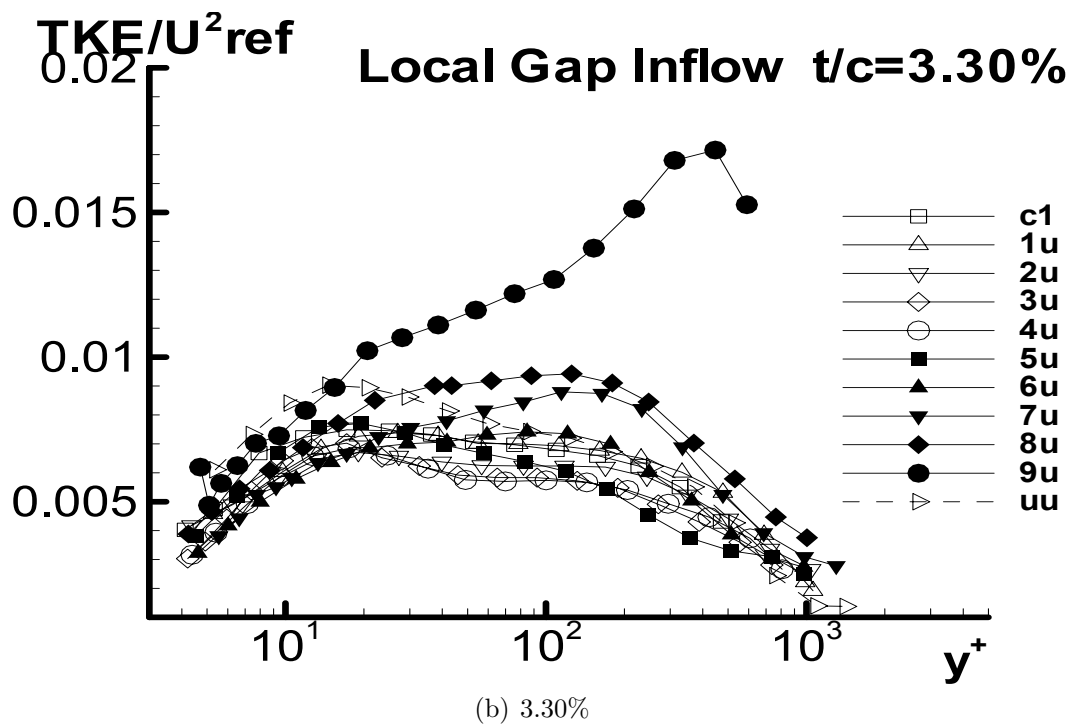
Figure H.8: TKE/U^2_{ref} of local gap inflow for both 1.65% and 3.30%
