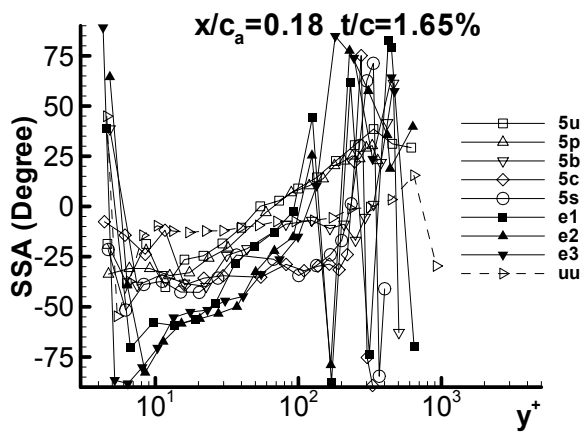
(i) x/c_a = 0.18 t/c = 1.65\%
