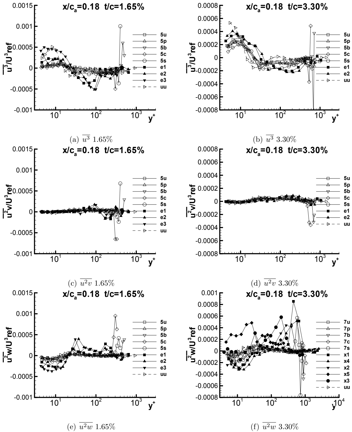
Figure G.14: Triple products \overline{u^3}/U_{ref}^3 , \overline{u^2v}/U_{ref}^3 , and \overline{u^2w}/U_{ref}^3 at x/c_a = 0.18 for both 1.65% and 3.30% in chord coordinate system
