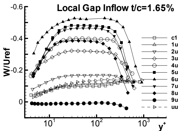
(c) Local Upstream t/c = 1.65\%
