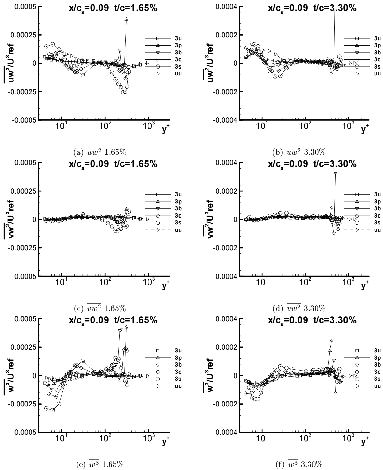
Figure G.21: Triple products \overline{uw^2}/U^3_{ref} , \overline{vw^2}/U^3_{ref} , and \overline{w^3}/U^3_{ref} at x/c_a = 0.09 for both 1.65% and 3.30% in chord coordinate system
