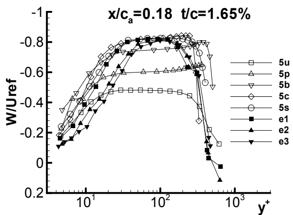
(a) x/c_a = 0.18 t/c = 1.65\%
