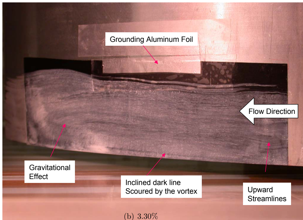
Figure 4.3: Blade suction surface oil flow visualizations for 1.65% and 3.30% with moving wall
