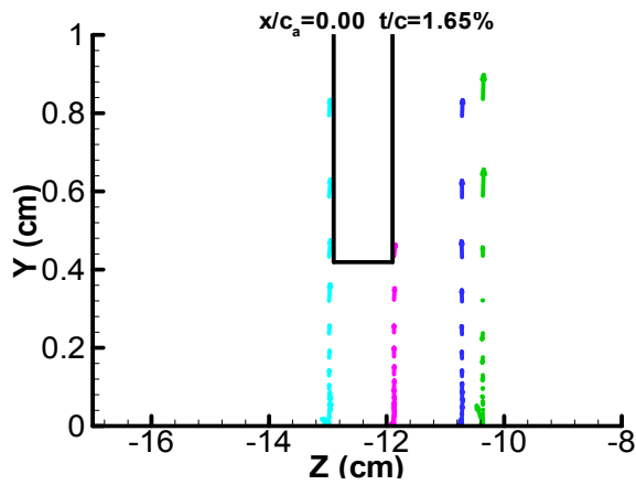
(a) x/c_a = 0.00 t/c = 1.65\%
