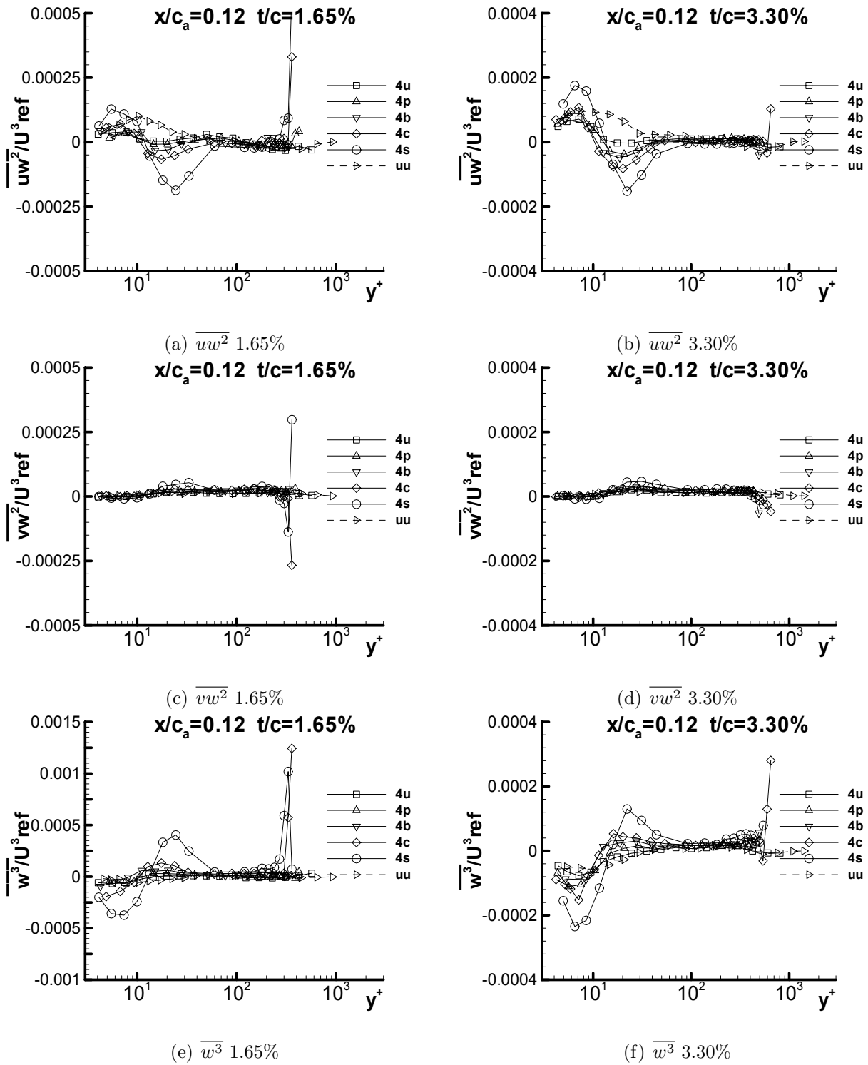
Figure G.22: Triple products \overline{uw^2}/U_{ref}^3 , \overline{vw^2}/U_{ref}^3 , and \overline{w^3}/U_{ref}^3 at x/c_a = 0.12 for both 1.65% and 3.30% in chord coordinate system
