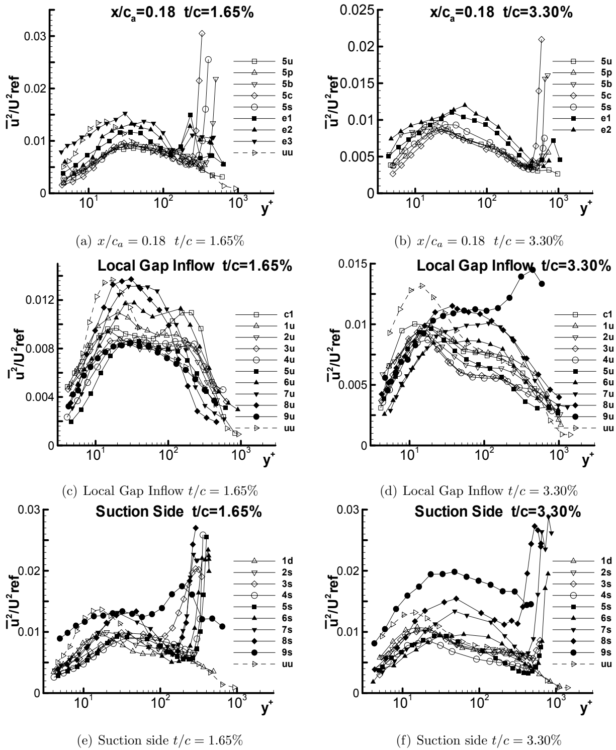
Figure 3.19: Normal stress \bar{u}^2/U_{ref}^2 for both 1.65% and 3.30% in chord coordinate system
