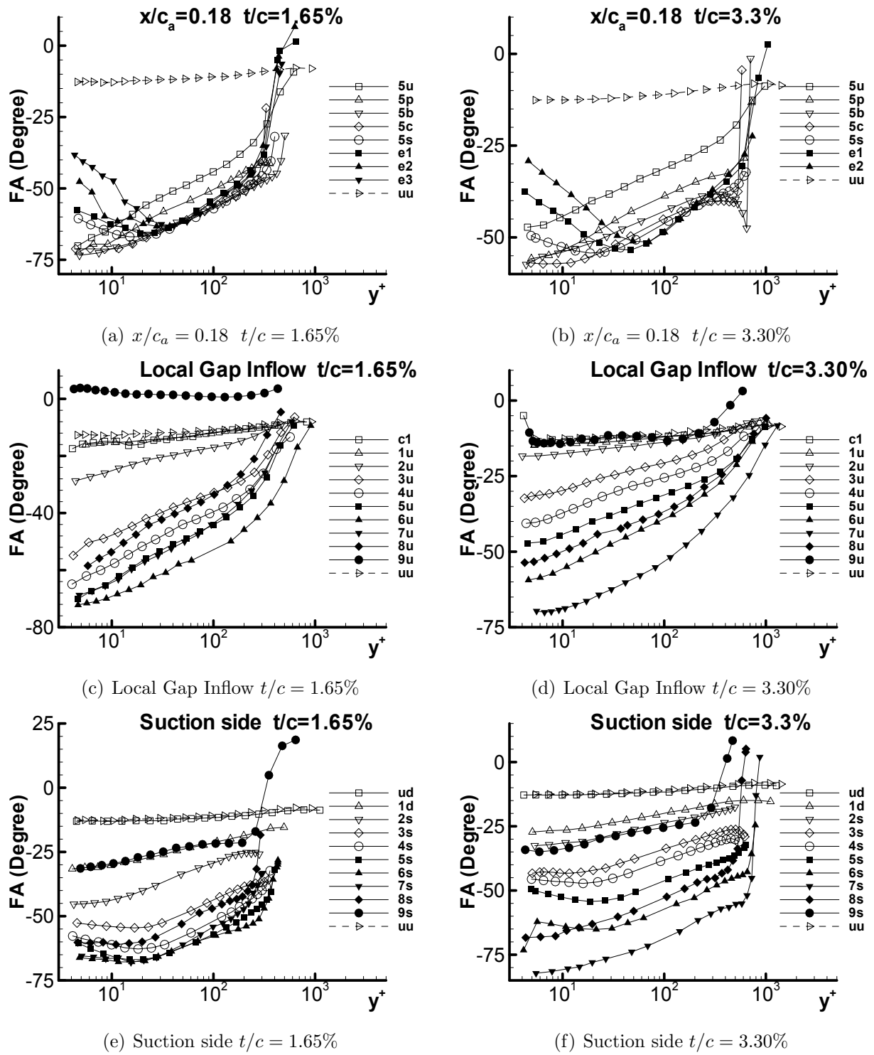
Figure 3.31: Flow angle for both 1.65% and 3.30% in chord coordinate system
