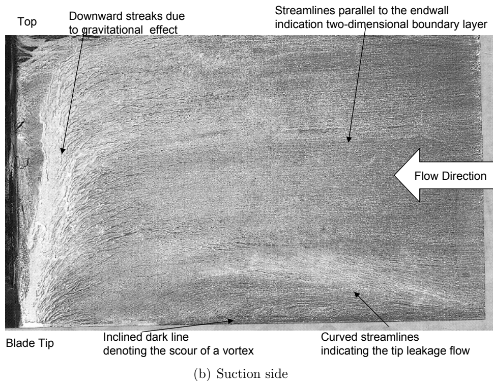
Figure 3.8: Blade surface oil flow visualizations for 3.30%
