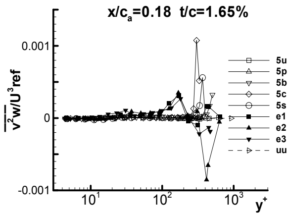
(a) x/c_a = 0.18 \quad t/c = 1.65\%
