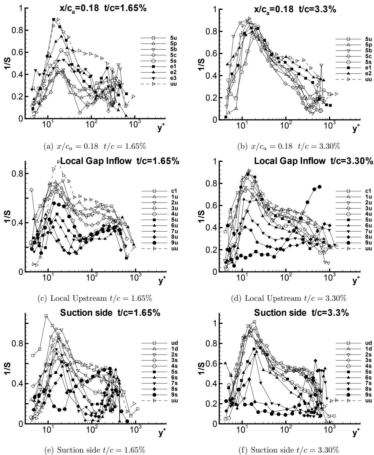
Figure 3.37: 1/S for both 1.65% and 3.30%
