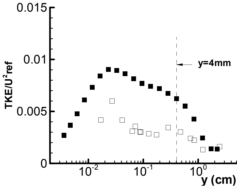
(a) Turbulent kinetic energy
