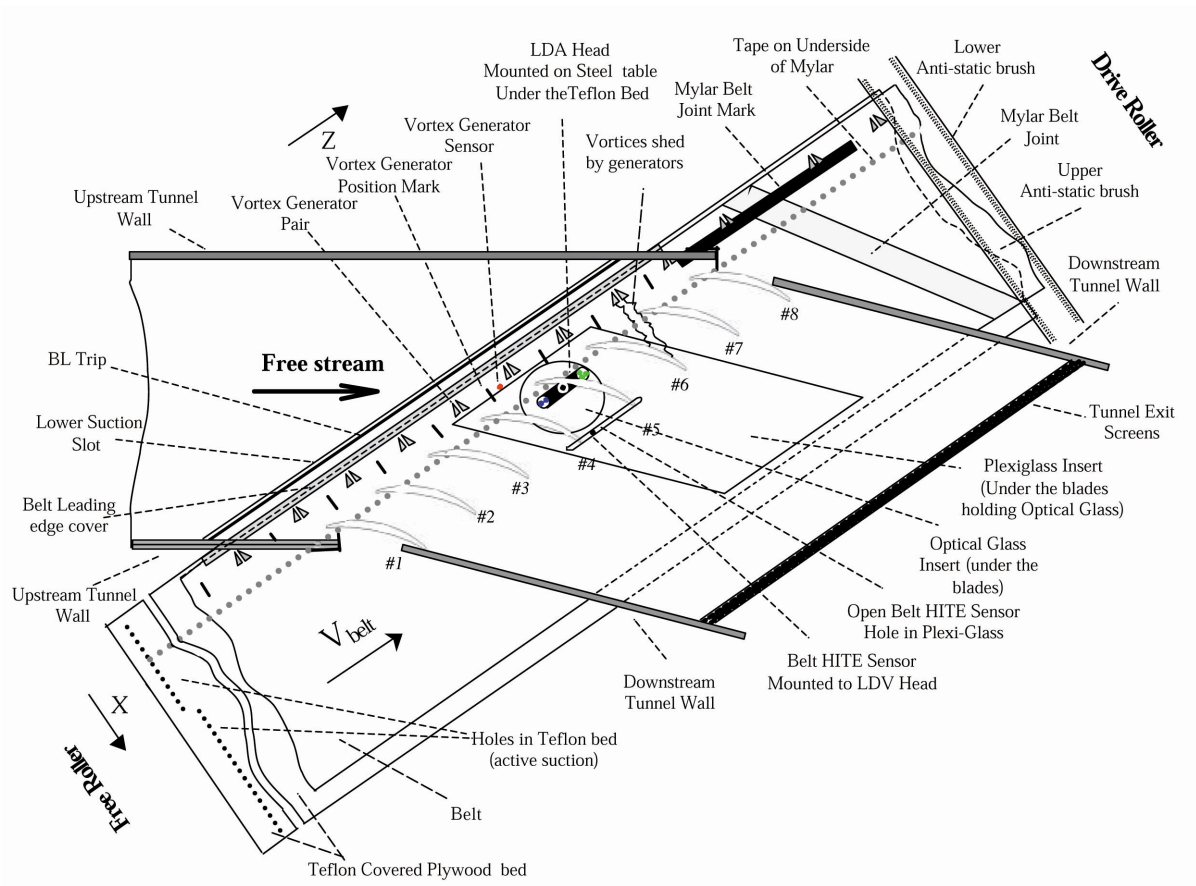
Figure 2.1: Top view of experimental test section setup in the Cascade Wind Tunnel from Kuhl (2001)
