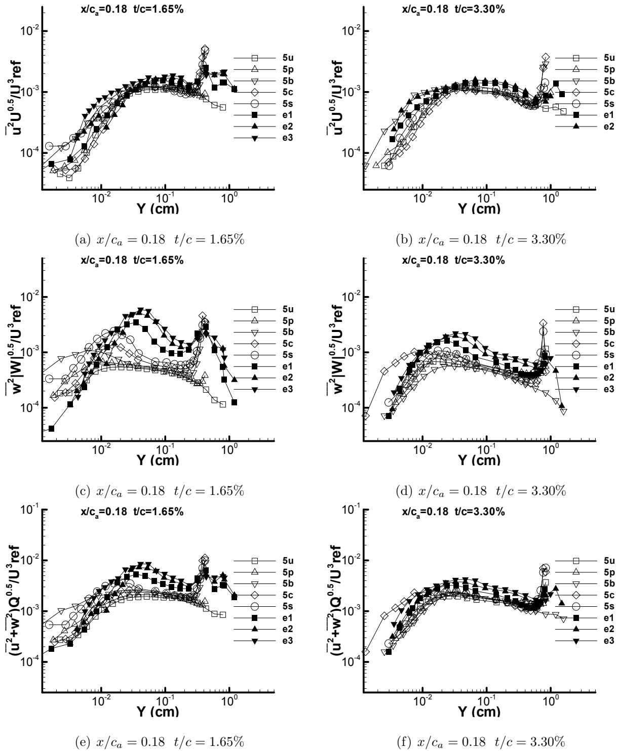
Figure 3.43: \overline{u^2} U^{0.5} / U_{ref}^3 , \overline{w^2} |W|^{0.5} / U_{ref}^3 , (\overline{u^2} + \overline{w^2}) Q^{0.5} / U_{ref}^3 at x/c_a = 0.18 for both 1.65% and 3.30% in chord coordinate system
