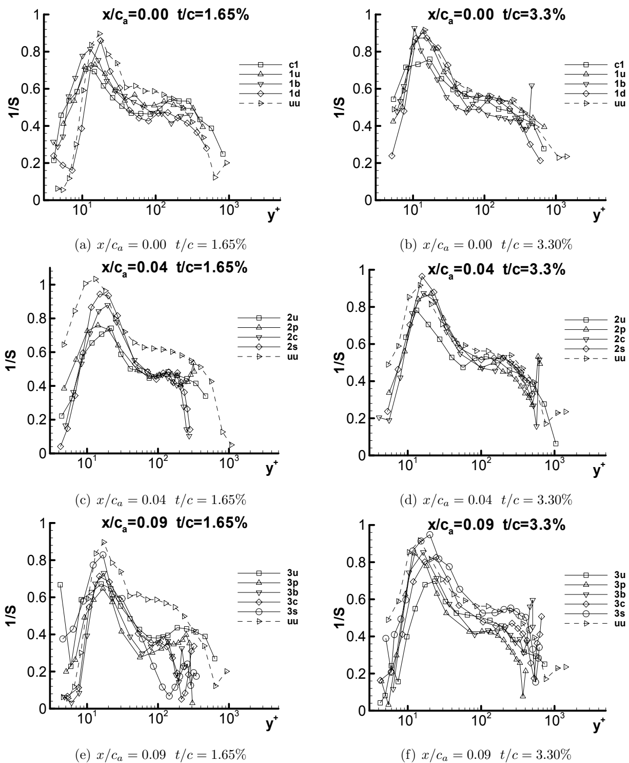
Figure H.13: 1/S for both 1.65% and 3.30%
