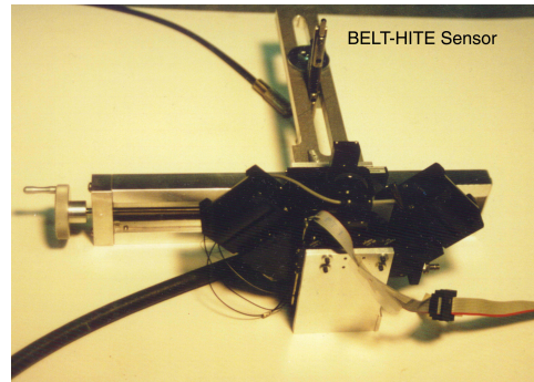
Figure 2.12: Assembly of LDV head and displacement sensor along with a traverse
