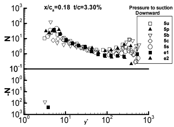
(j) x/c_a = 0.18 t/c = 3.30\%
