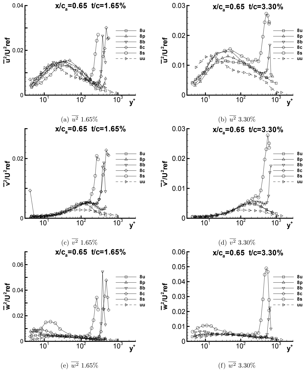
Figure F.8: Reynolds normal stresses \bar{u}^2/U_{ref}^2 , \bar{v}^2/U_{ref}^2 , and \bar{w}^2/U_{ref}^2 at x/c_a = 0.65 for both 1.65% and 3.30% in chord coordinate system
