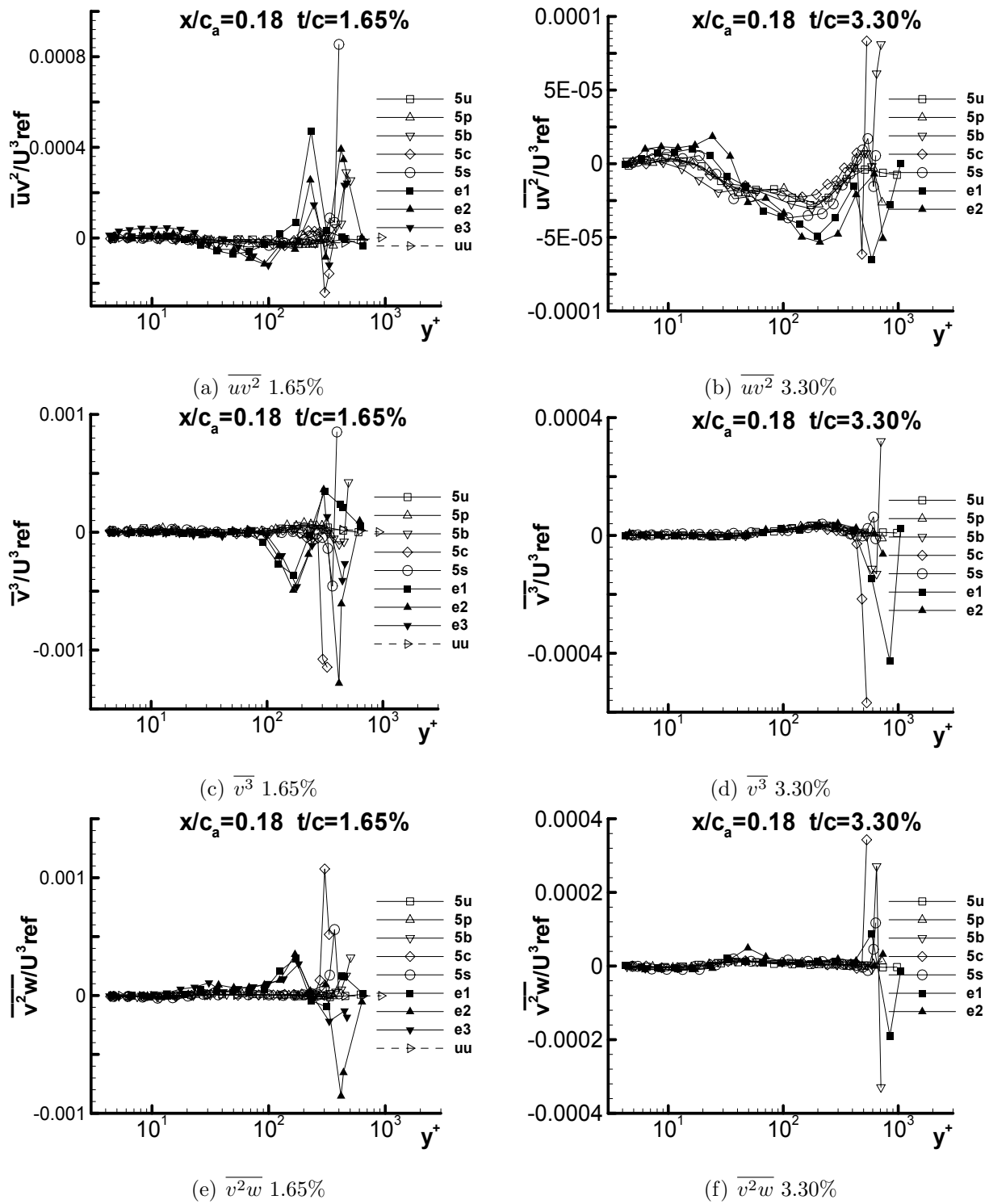
Figure G.5: Triple products \overline{uv^2}/U_{ref}^3 , \overline{v^3}/U_{ref}^3 , and \overline{v^2w}/U_{ref}^3 at x/c_a = 0.18 for both 1.65% and 3.30% in chord coordinate system
