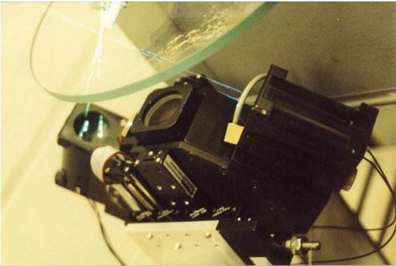
Figure 2.10: Miniature 3D fiber-optic LDV head
