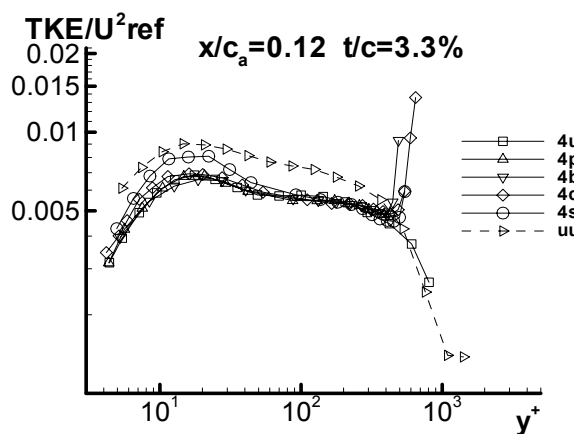
(h) x/c_a = 0.12 t/c = 3.30\%
