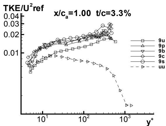
(r) x/c_a = 1.00 t/c = 3.30\%
