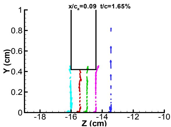
(e) x/c_a = 0.09 t/c = 1.65\%
