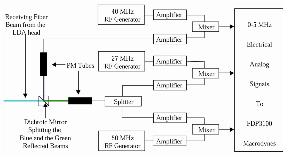
Figure 2.14: Schematic of LDV signal conditioning for the Cascade Wind Tunnel
