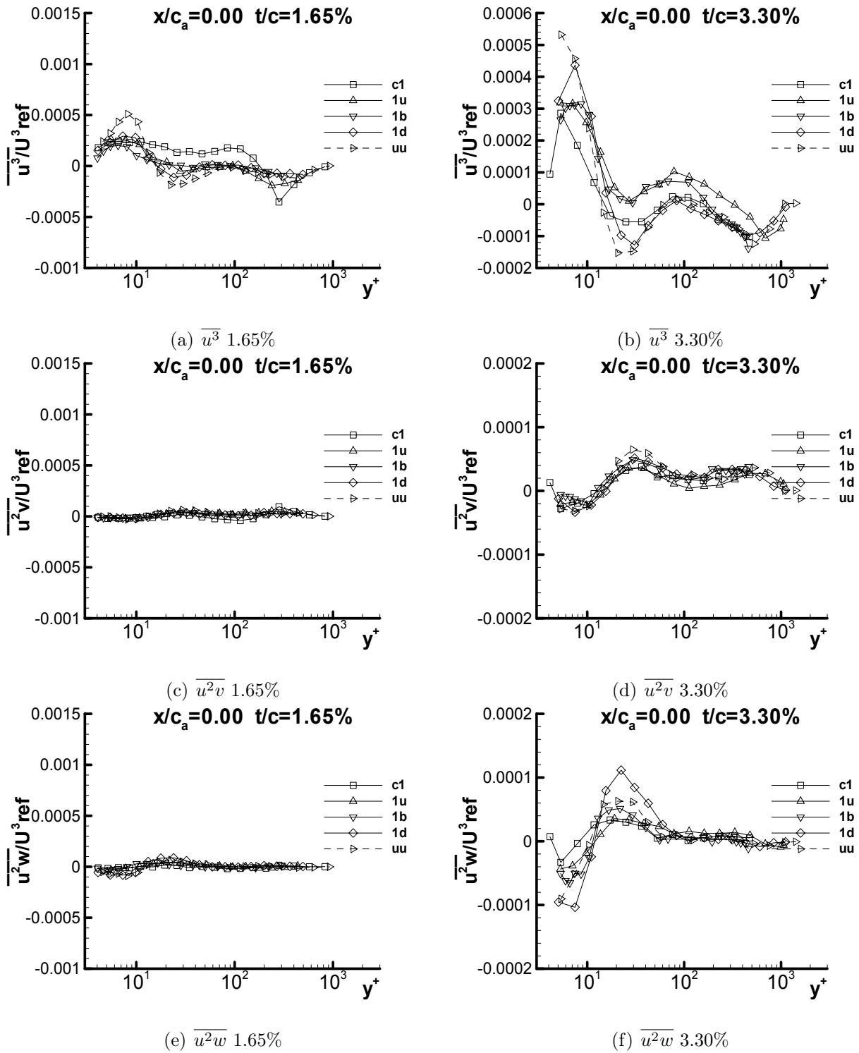
Figure G.10: Triple products \overline{u^3}/U^3_{ref} , \overline{u^2v}/U^3_{ref} , and \overline{u^2w}/U^3_{ref} at x/c_a = 0.00 for both 1.65% and 3.30% in chord coordinate system
