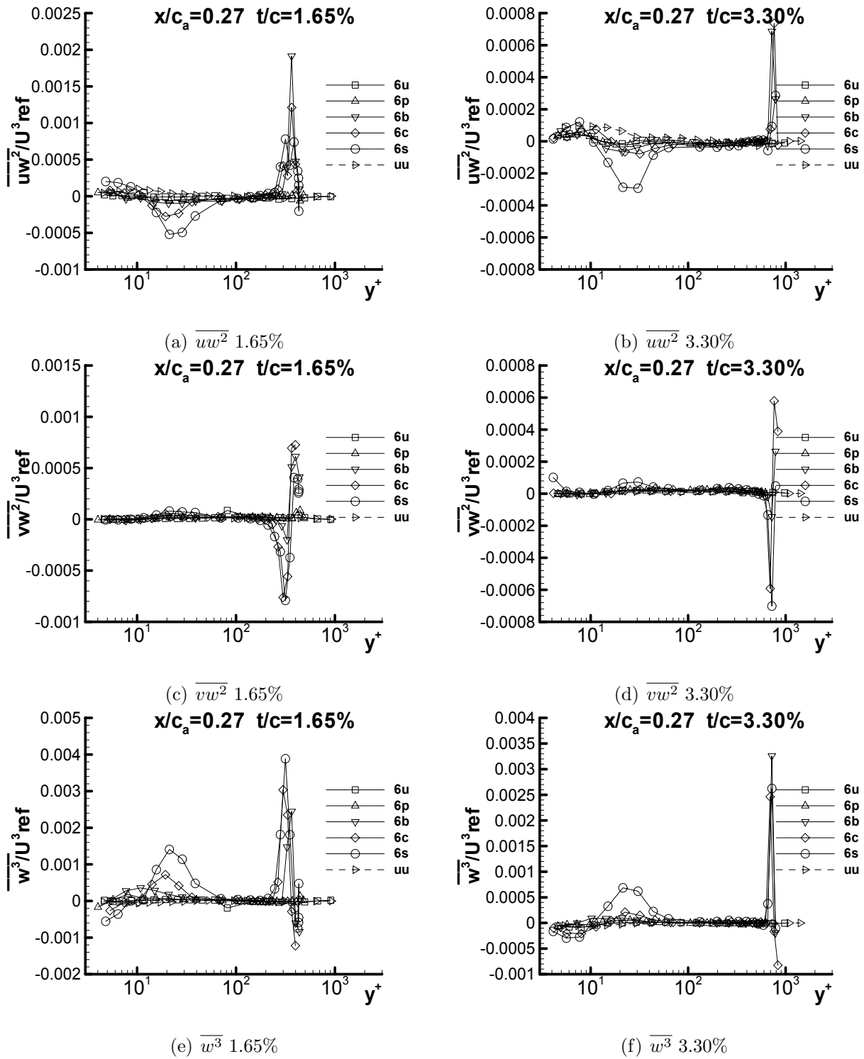
Figure G.24: Triple products \overline{uw^2}/U_{ref}^3 , \overline{vw^2}/U_{ref}^3 , and \overline{w^3}/U_{ref}^3 at x/c_a = 0.27 for both 1.65% and 3.30% in chord coordinate system
