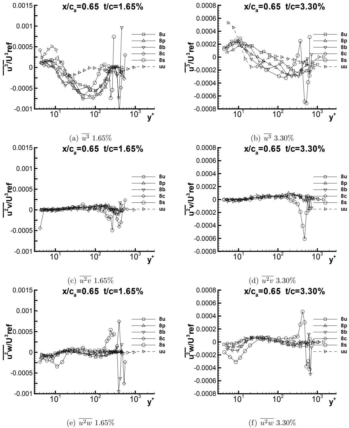
Figure G.17: Triple products \overline{u^3}/U^3_{ref} , \overline{u^2v}/U^3_{ref} , and \overline{u^2w}/U^3_{ref} at x/c_a = 0.65 for both 1.65% and 3.30% in chord coordinate system
