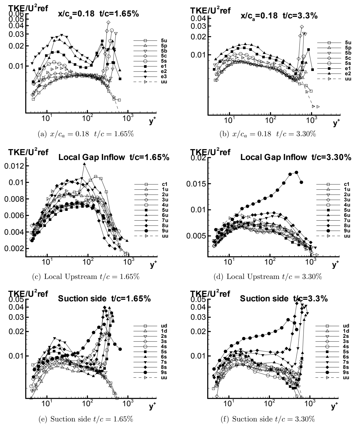
Figure 3.35: Turbulent kinetic energy TKE/U_{ref}^2 for both 1.65% and 3.30%
