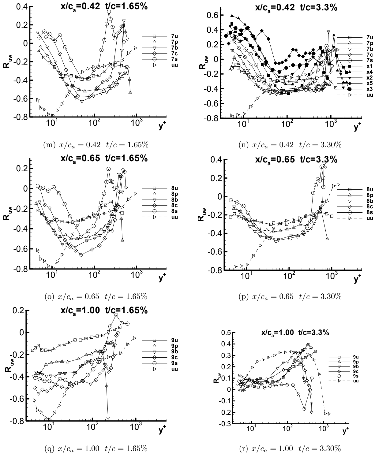
Figure H.17: Correlation coefficients of \overline{vw} for both 1.65% and 3.30% in chord coordinate system (cont.)
