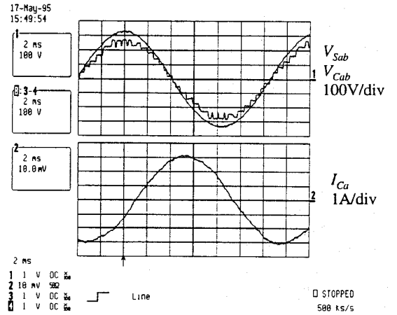
Fig. 15. Experimental results showing line-to-line voltages of the source and the inverter, V_{S_{ab}} and V_{C_{ab}} , and the line current, I_{C_a} , at -1 kvar output.
