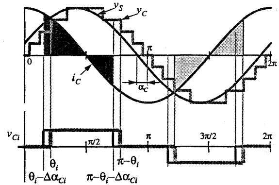
Fig. 9. Control principle of each dc capacitor voltage.
