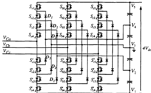
Fig. 2. Structure of the 5-level diode clamped inverter.
