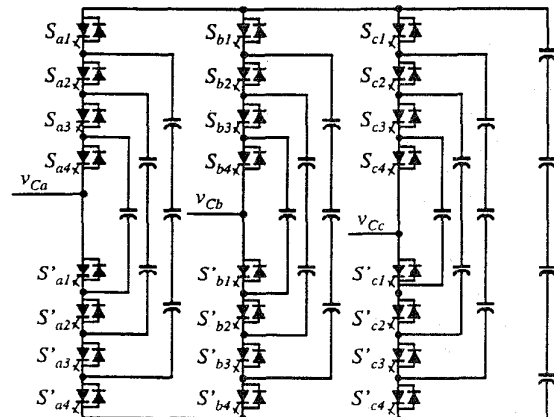
Fig. 3. Structure of the 5-level flying capacitor inverter.
