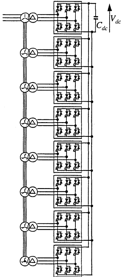
Fig. 1. Structure of the conventional 48-pulse inverter.
