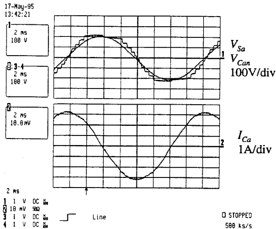
Fig. 11. Experimental results showing phase voltages of the source and the inverter, V_{S_a} and V_{C_{an}} , and the line current, I_{C_a} , at +1 kvar output.
