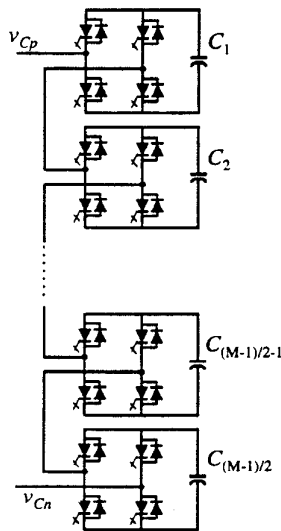
Fig. 4. Single phase structure of multilevel cascade inverter.
