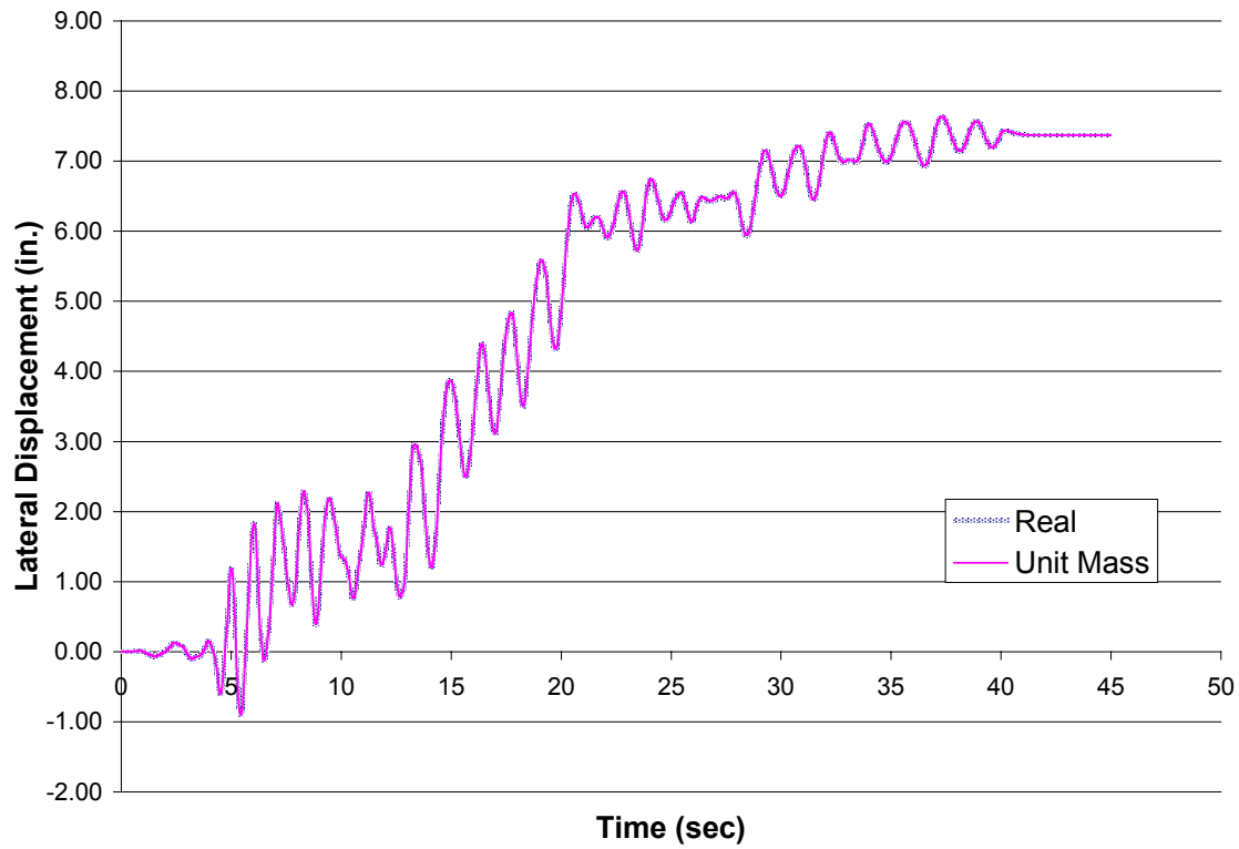
Figure B3.2 – Chalfant Valley (EQ3), Response Histories for Seven Story Comparative Models with Vertical Accelerations Included
