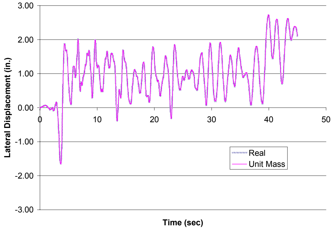
Figure B8.1 – Taft (EQ4), Response Histories for Nine Story Comparative Models without Vertical Accelerations Included
