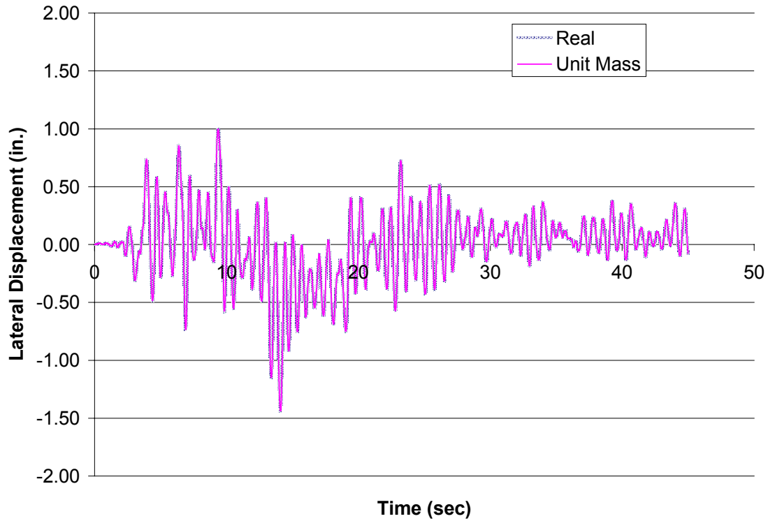
Figure B5.1 – Taft (EQ4), Response Histories for Three Story Comparative Models without Vertical Accelerations Included
