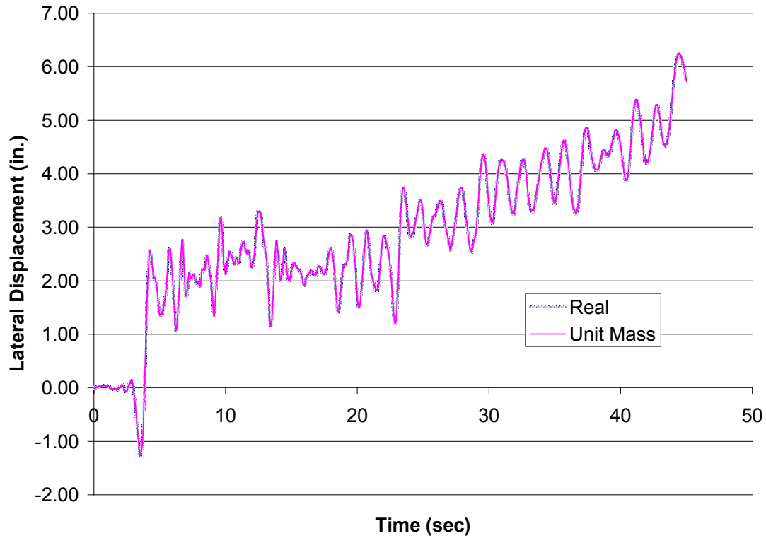
Figure B7.1 – Taft (EQ4), Response Histories for Seven Story Comparative Models without Vertical Accelerations Included
