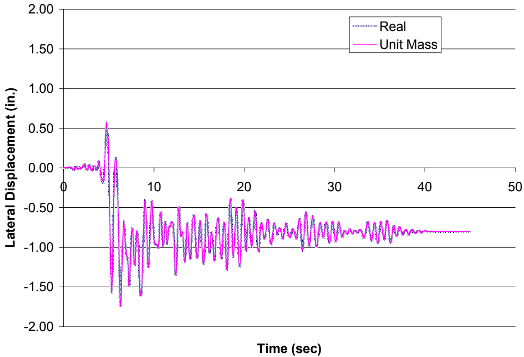
Figure B1.1 – Chalfant Valley (EQ3), Response Histories for Three Story Comparative Models without Vertical Accelerations Included
