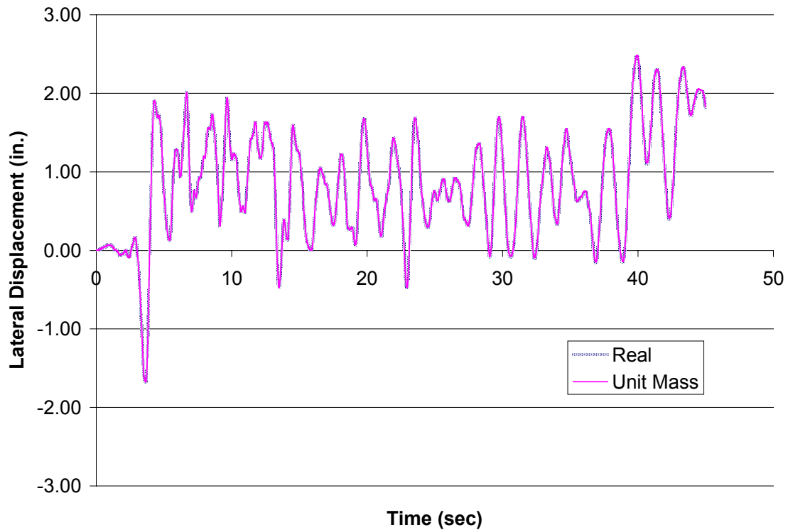
Figure B8.2 – Taft (EQ4), Response Histories for Nine Story Comparative Models with Vertical Accelerations Included
