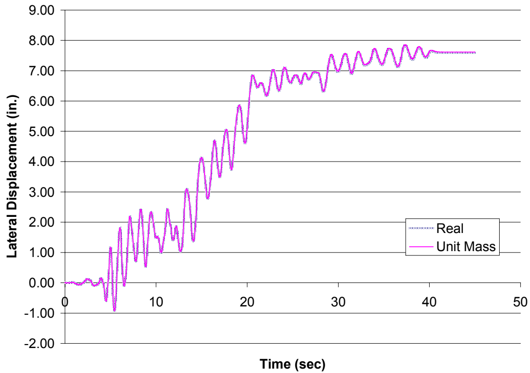
Figure B3.1 – Chalfant Valley (EQ3), Response Histories for Seven Story Comparative Models without Vertical Accelerations Included
