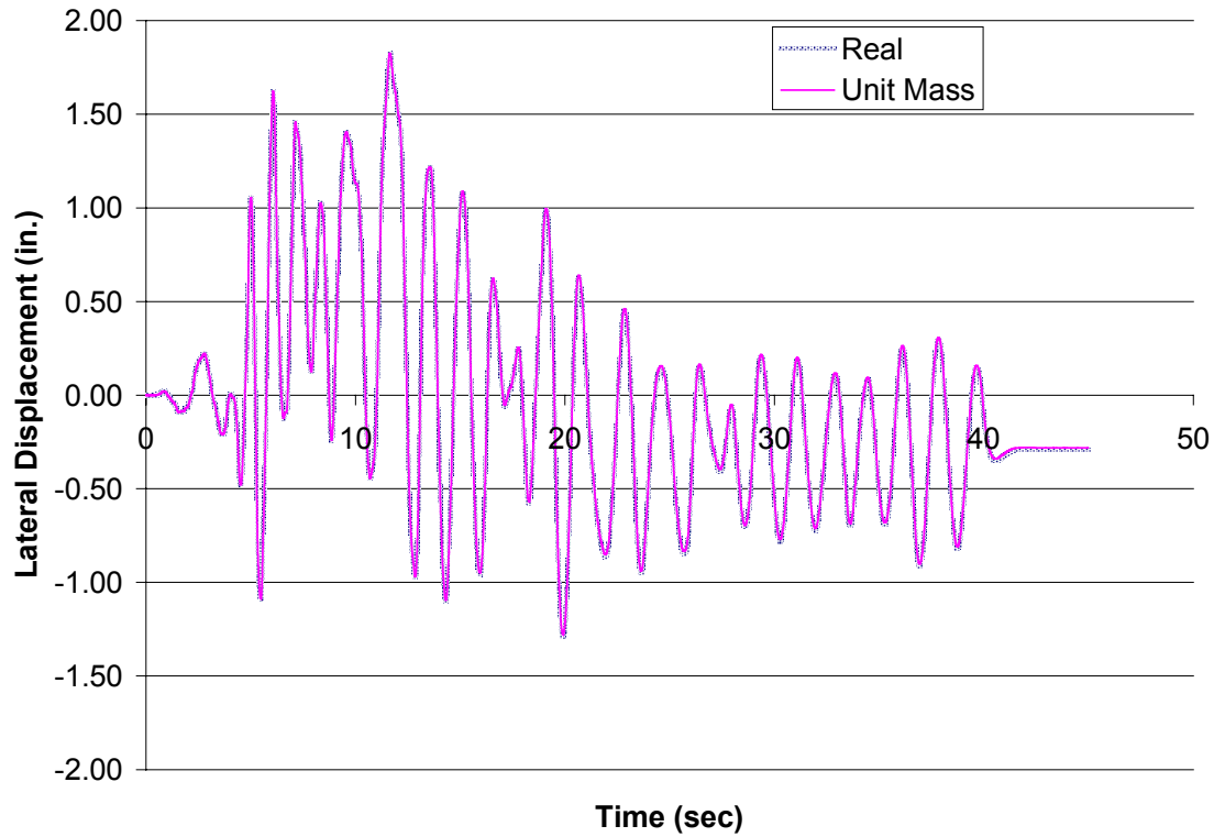
Figure B4.1 – Chalfant Valley (EQ3), Response Histories for Nine Story Comparative Models without Vertical Accelerations Included
