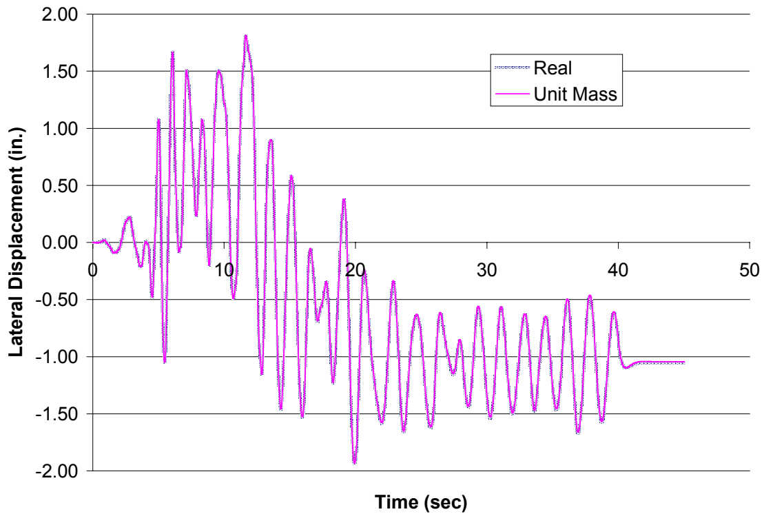
Figure B4.2 – Chalfant Valley (EQ3), Response Histories for Nine Story Comparative Models with Vertical Accelerations Included
