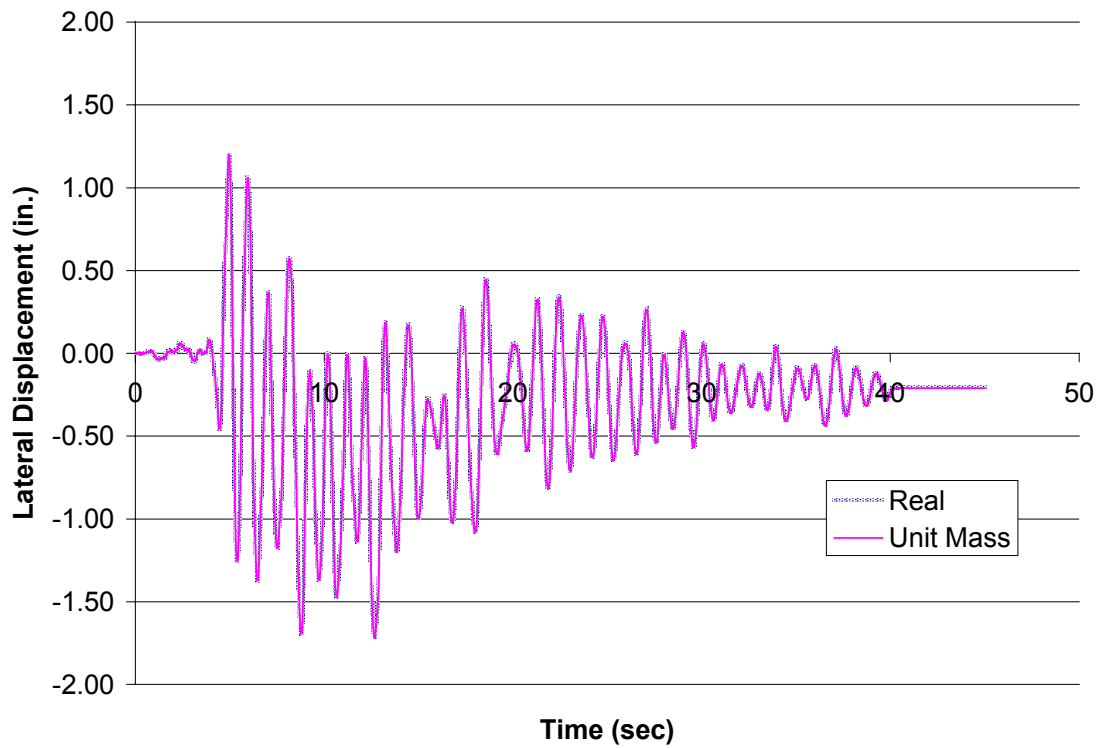
Figure B2.2 – Chalfant Valley (EQ3), Response Histories for Five Story Comparative Models with Vertical Accelerations Included
