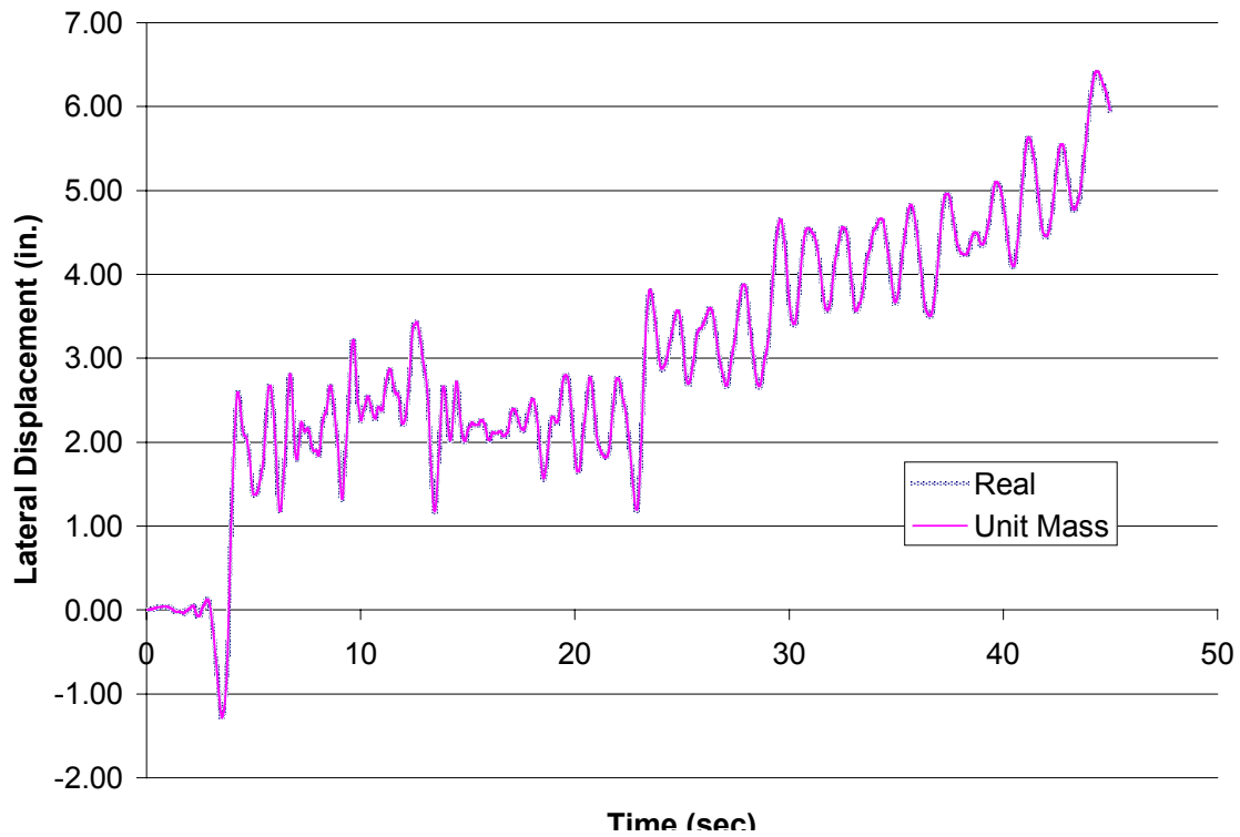
Figure B7.2 – Taft (EQ4), Response Histories for Seven Story Comparative Models with Vertical Accelerations Included
