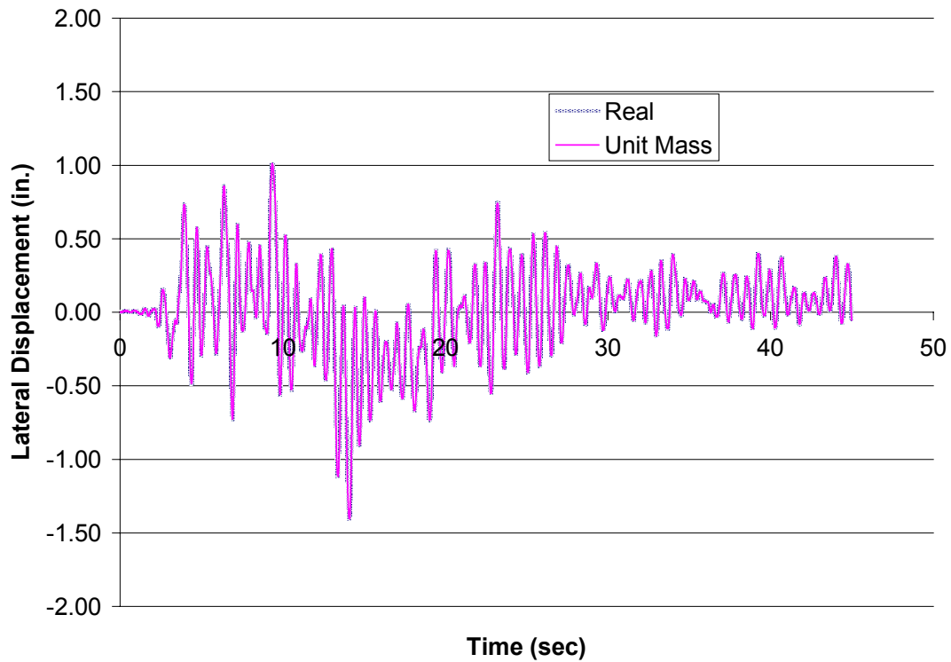
Figure B5.2 – Taft (EQ4), Response Histories for Three Story Comparative Models with Vertical Accelerations Included
