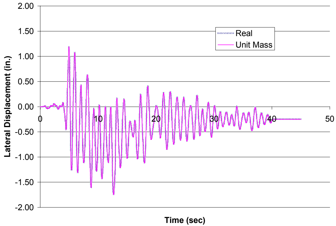
Figure B2.1 – Chalfant Valley (EQ3), Response Histories for Five Story Comparative Models without Vertical Accelerations Included
