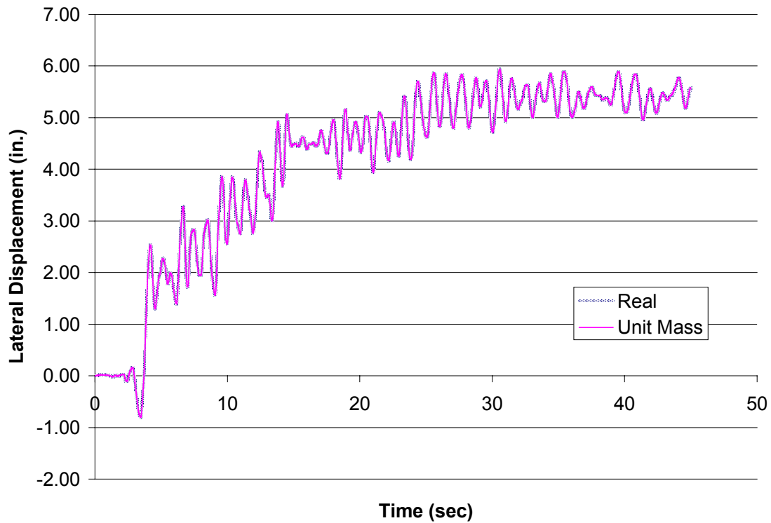
Figure B6.2 – Taft (EQ4), Response Histories for Five Story Comparative Models with Vertical Accelerations Included
