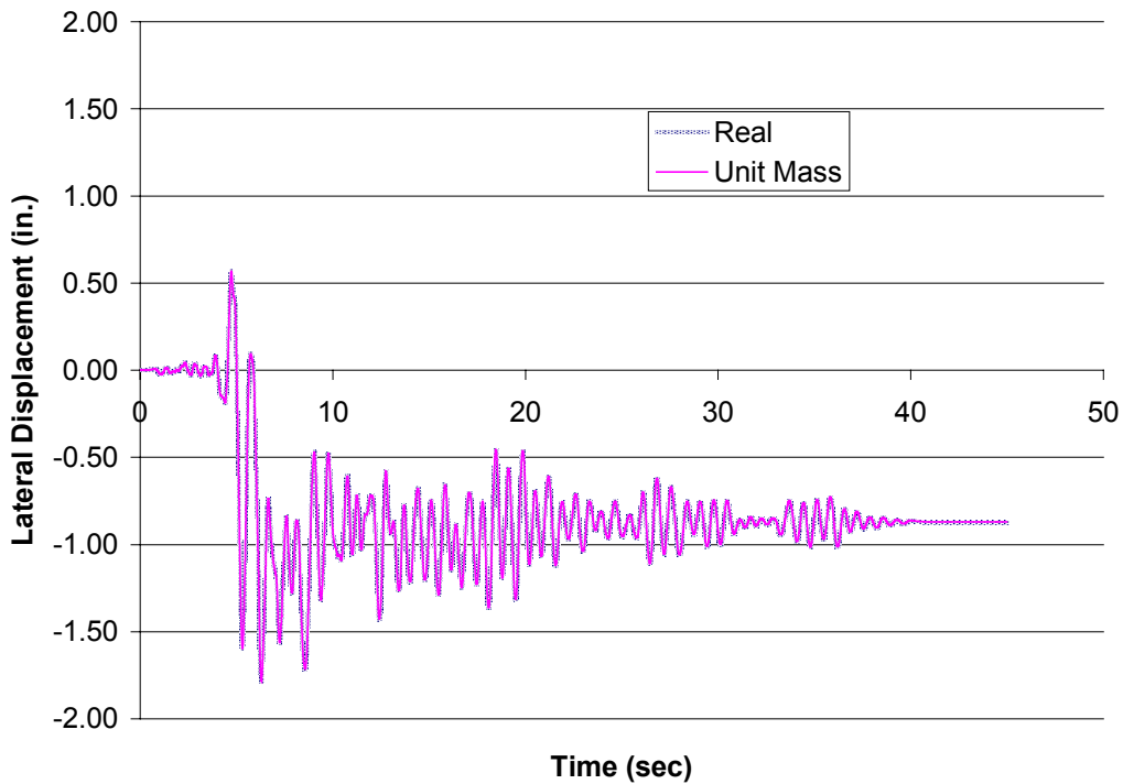
Figure B1.2 – Chalfant Valley (EQ3), Response Histories for Three Story Comparative Models with Vertical Accelerations Included
