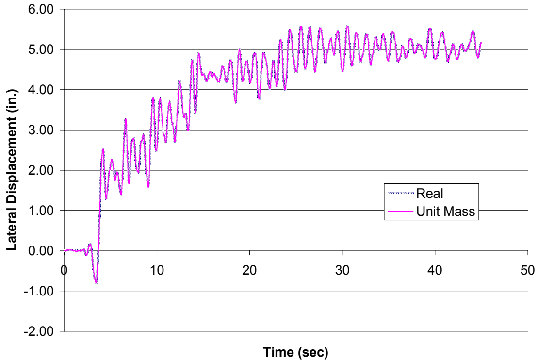
Figure B6.1 – Taft (EQ4), Response Histories for Five Story Comparative Models without Vertical Accelerations Included
