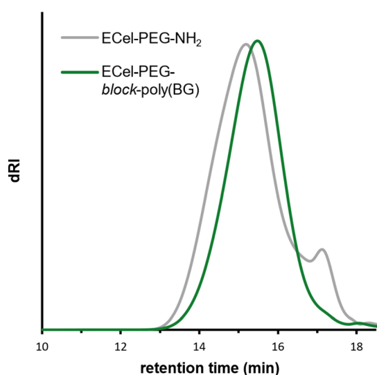
Fig. 3 SEC-MALS traces (dRI trace shown) of polymerization of BG-NTA using macroinitiator ECEl-PEG-NH 2 (ECEl-PEG- block -poly(BG), green) along with SEC trace of macroinitiator ECEl-PEG-NH 2 (grey). 1 H NMR spectra can be found in Fig. S10 & S14. † SEC eluent was DMAc/LiCl. M n (NMR) was estimated to be 40.4 kg mol -1 using poly(BG); ECEl ratio. M n (SEC-MALS) was estimated to be 36.7 kg mol -1 (D = 1.4) using a weighted ratio of dn/dc values for poly(BG) and ECEl.
