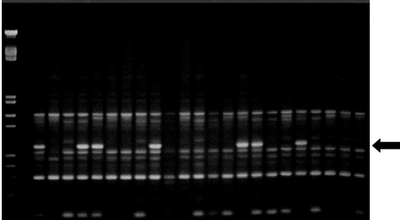
Figure 3.1. Distorted segregation among 22 anther-derived monoloids of BARD1-3 revealed by RAPD primer OPG-12. From left to right is a lambda DNA size marker, check lane containing all PCR reaction components except for genomic DNA, the anther donor BARD1-3, and 22 anther-derived monoloids.
