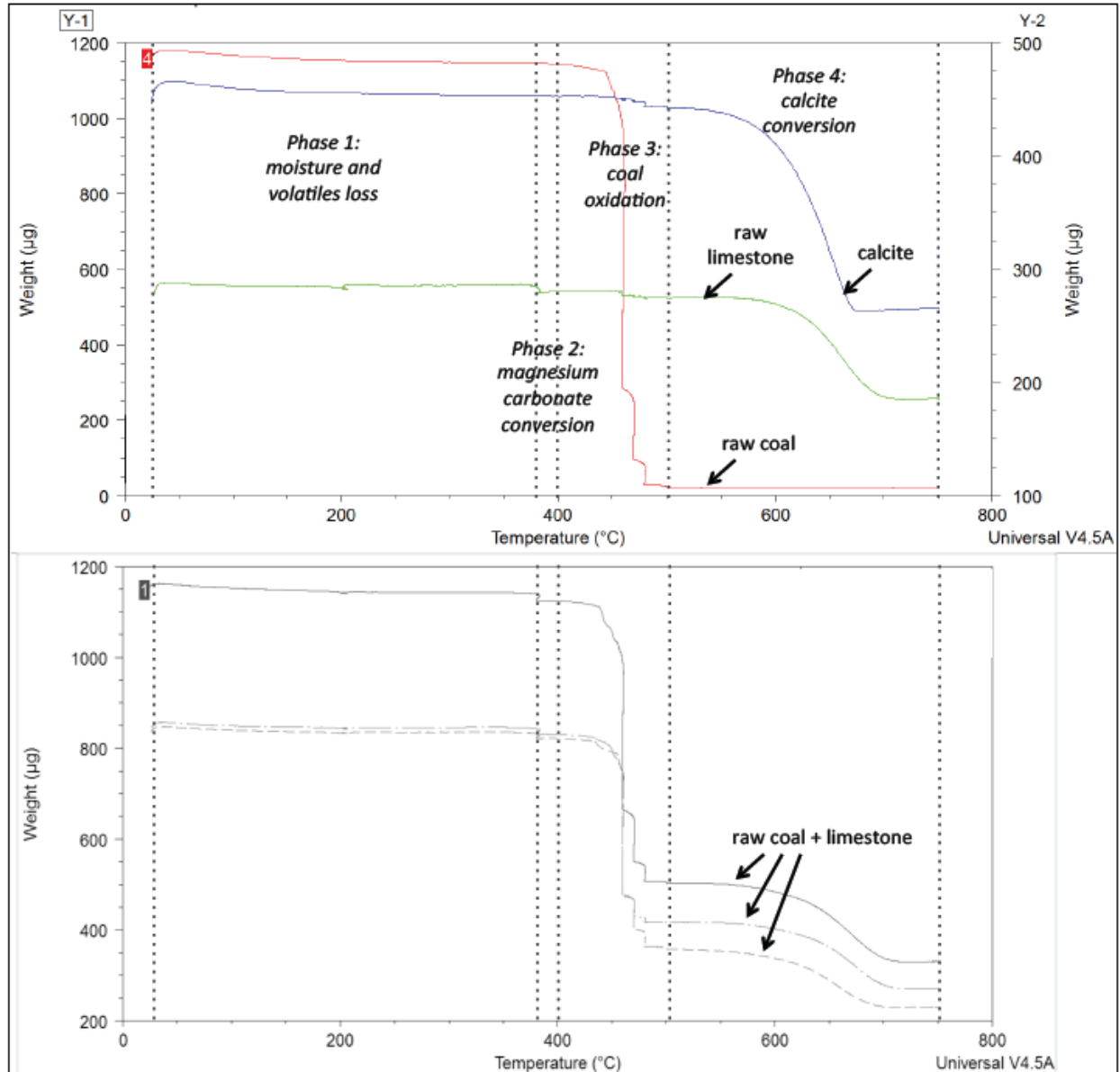
Fig. 4 Example thermograms for reagent grade calcite only, raw limestone only and raw coal dust only (top), and samples containing both raw coal and raw limestone dust (bottom). The TGA experiment method used here includes four major phases, which drive off moisture and volatiles at temperatures less than about 380°C, convert a minor fraction of the limestone to an oxide between about 380 and 400°C oxidize coal particles between about 400 and 500°C, and convert calcite to calcium oxide between about 500 and 750°C. The residue at the end of the experiments represents calcium oxide and/or inert mineral content in the raw coal.
