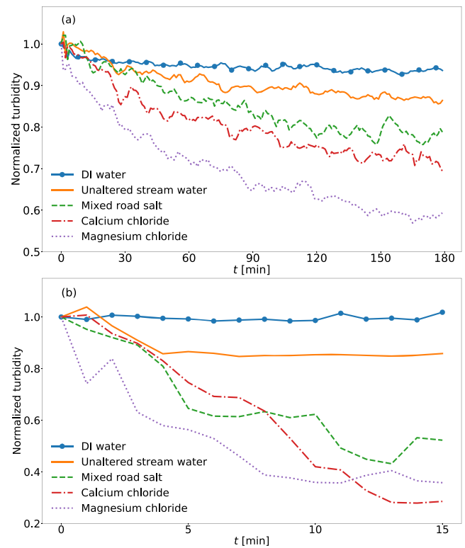
Figure 3. Time series of normalized turbidity at (a) turbulent shear rate of 20 s^{-1} and (b) stagnant water.
