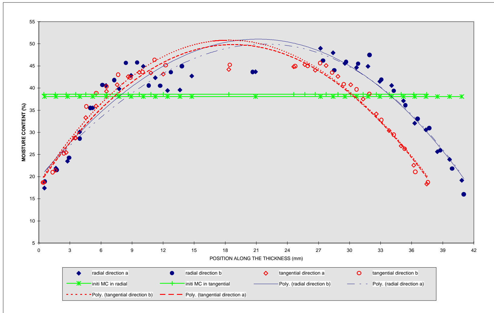
Figure 3.21. Moisture gradients measured with the flaking technique along the radial and tangential direction after 8 days drying
