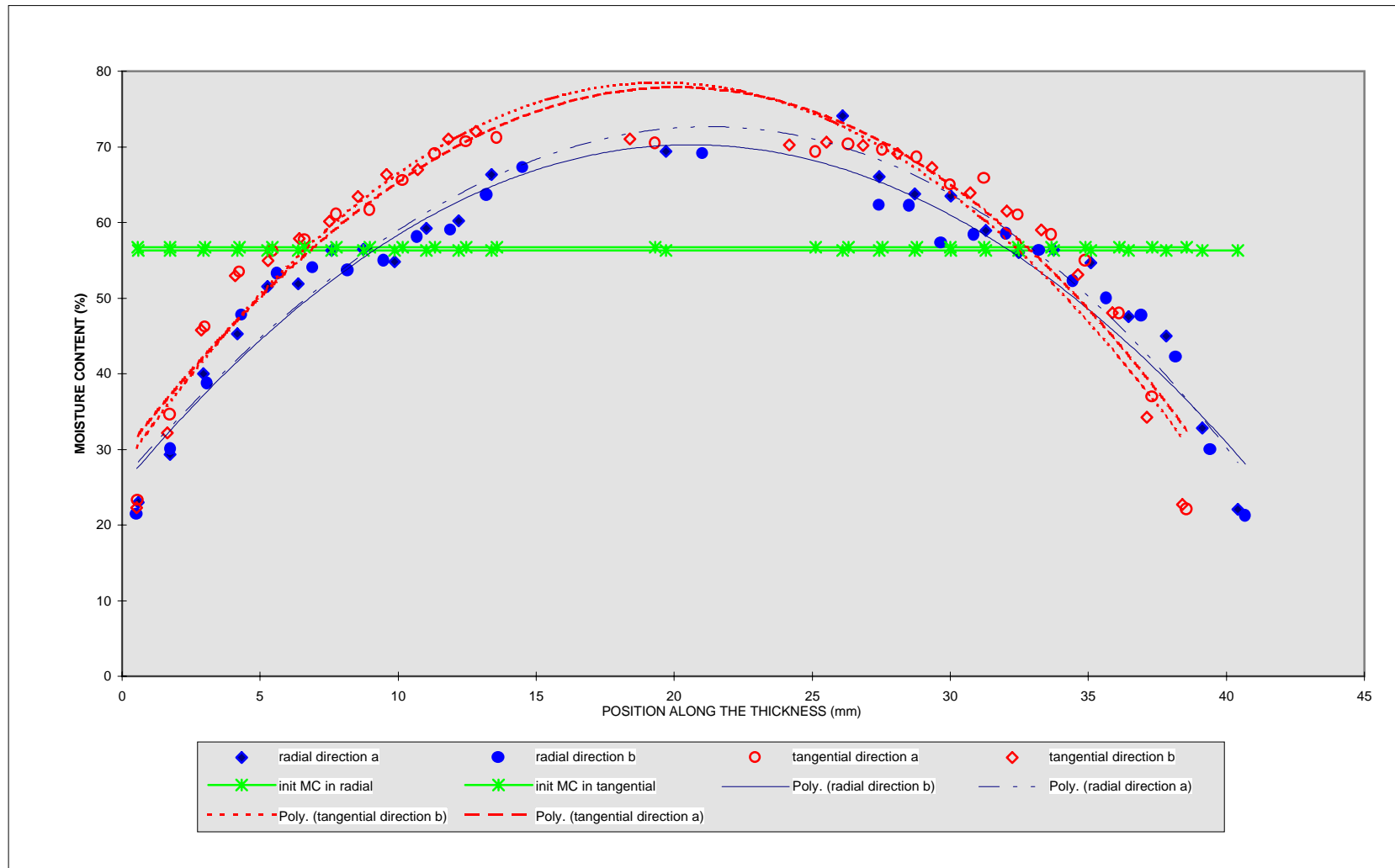
Figure 3.19. Moisture gradients measured with the flaking technique along radial and tangential direction after 4 days drying
