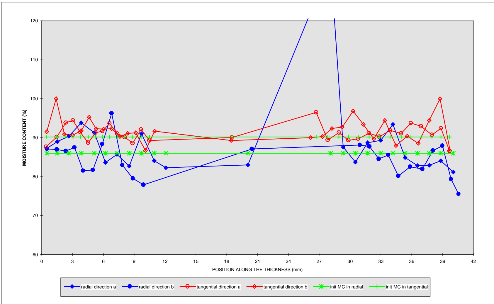
Figure 3.17. Moisture gradients measured with the flaking technique along the radial and tangential direction under green condition
