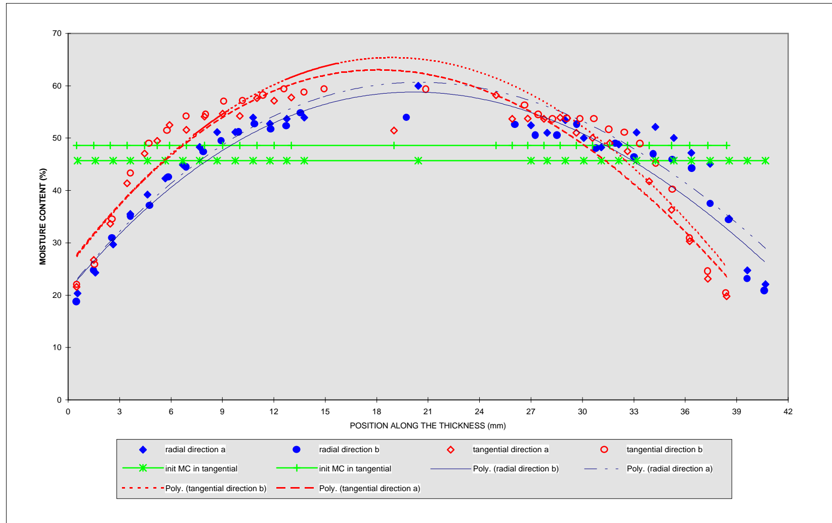
Figure 3.20. Moisture gradients measured with the flaking technique along radial and tangential direction after 6 days drying
