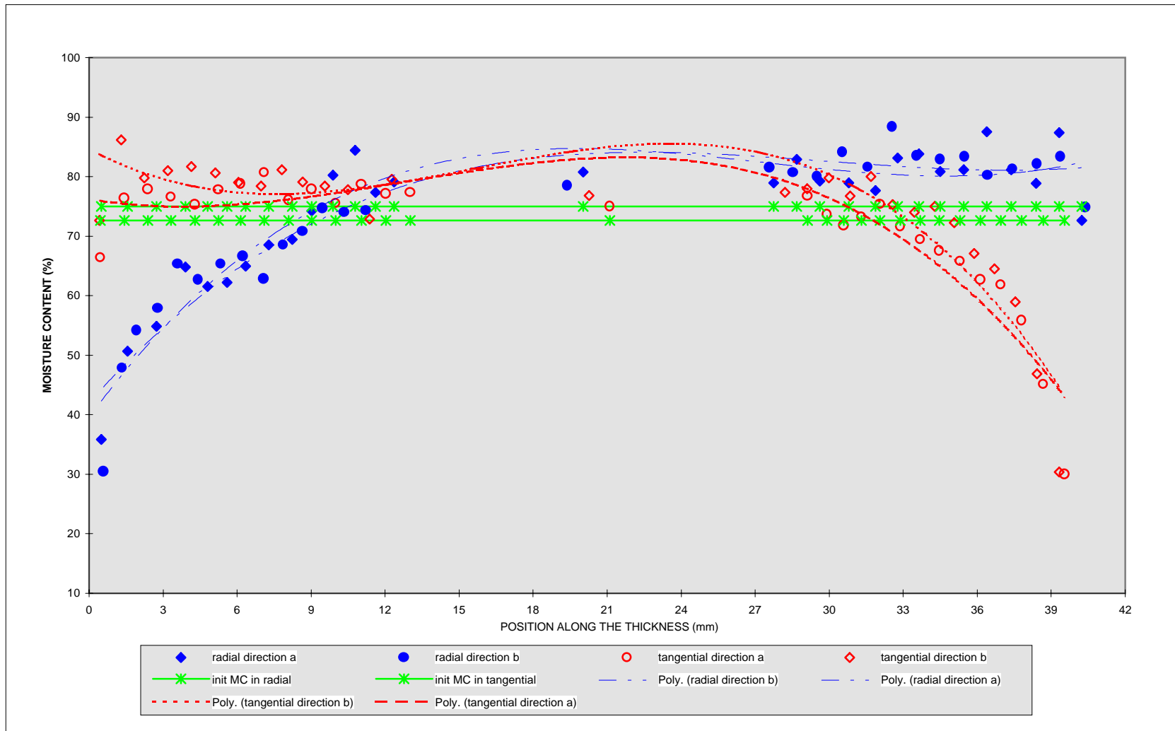
Figure 3.18. Moisture gradients measured with the flaking technique along radial and tangential direction after 2 days drying
