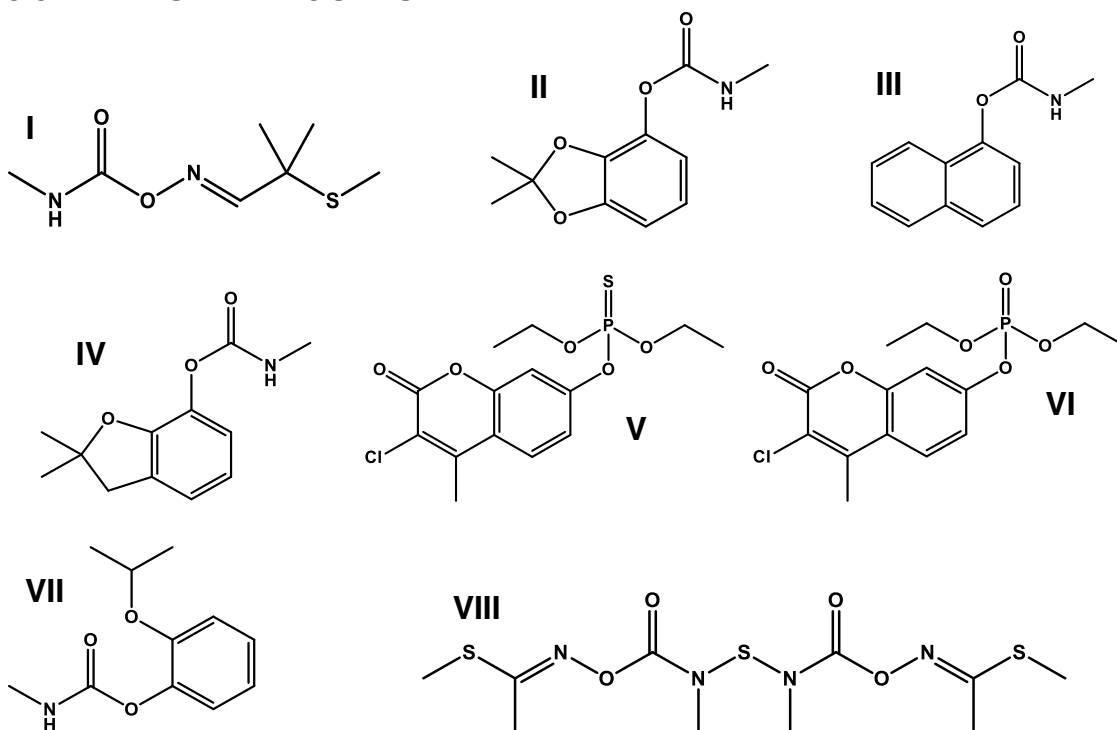
Figure 1. Chemical structures (and International Union of Pure and Applied Chemistry (IUPAC) names) of known AChE inhibitors used in this study: (I) aldicarb (2-Methyl-2-(methylthio)propanal O -( N -methylcarbamoyl)oxime), (II) bendiocarb ((2,2-Dimethyl-1,3-benzodioxol-4-yl) N -methylcarbamate), (III) carbaryl (1-naphthyl methylcarbamate), (IV) carbofuran (2,2-Dimethyl-2,3-dihydro-1-benzofuran-7-yl methylcarbamate), (V) coumaphos ( O,O -Diethyl O -3-chloro-4-methyl-2-oxo-2H-chromen-7-yl phosphorothioate), (VI) coumaphos-oxon ((3-chloro-4-methyl-2-oxochromen-7-yl) diethyl phosphate), (VII) propoxur (2-Isopropoxyphenyl N -methylcarbamate), and (VIII) thiodicarb (methyl (1 E )- N -[methyl-[methyl-[( E )-1-methylsulfanylethylideneamino]Oxycarbonylamino]sulfanylcabamoyl]oxyethanimidothioate).
