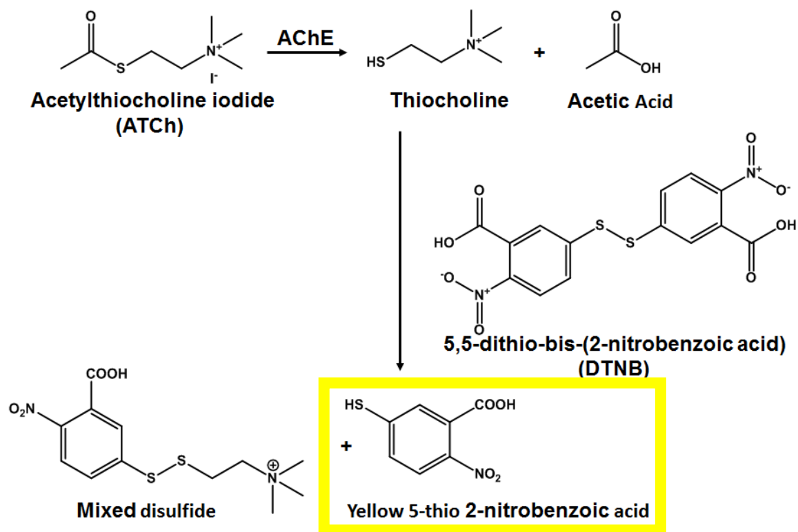
Figure 5. Reaction that takes place in the Ellman Assay: acetylthiocholine iodide is hydrolyzed by AChE, forming thiocholine and acetic acid. Thiocholine reacts with DTNB to form yellow 5-thio-2-nitrobenzoic acid and mixed disulfide products. A strong yellow color in microplate wells after this assay indicate low inhibition of AChE.
