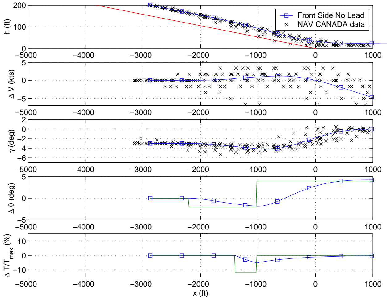
Figure 4.7: Long Initial Condition Response with No Lead
