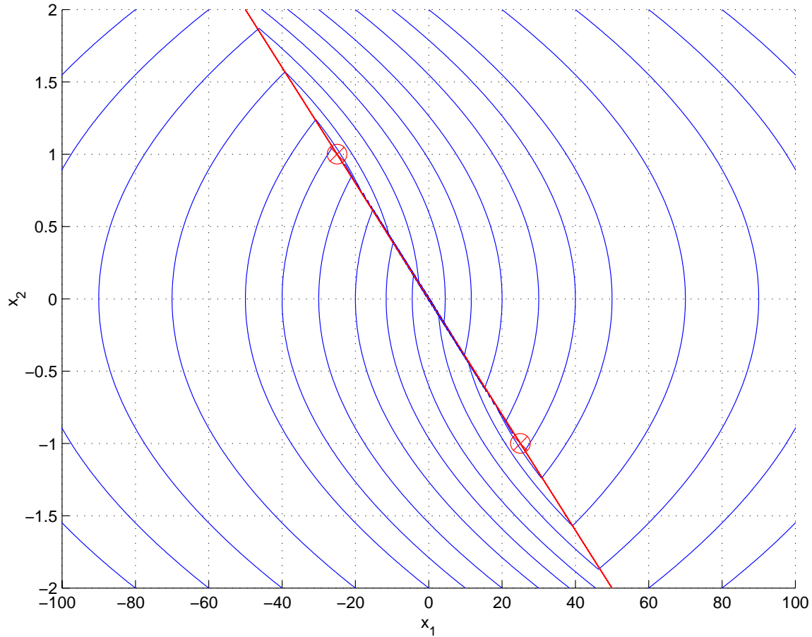
Figure 2.1: Second Order System Sliding Mode Example
