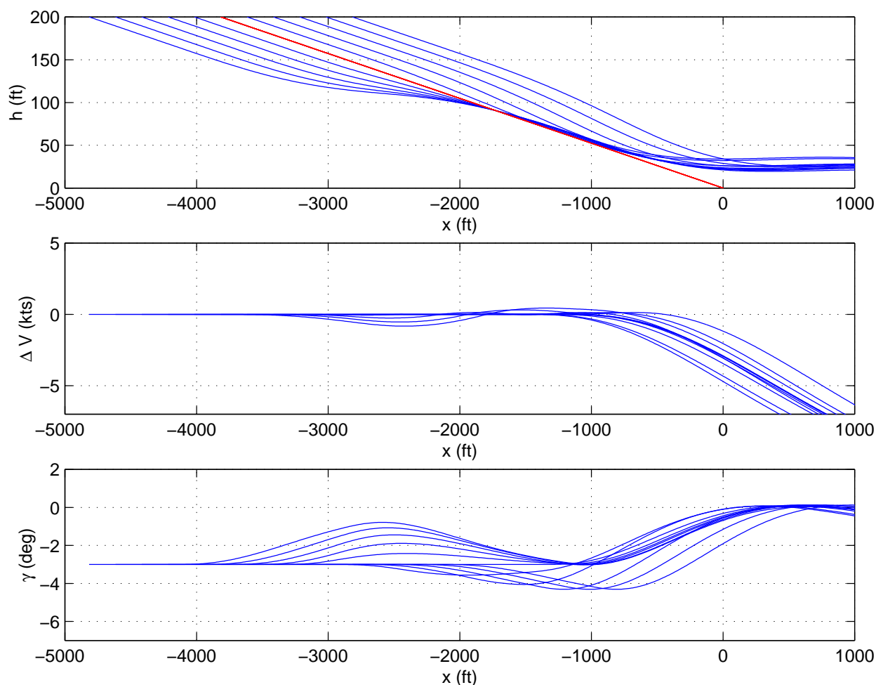
Figure 6.1: Front-Side Aircraft Refined Landing Strategy
