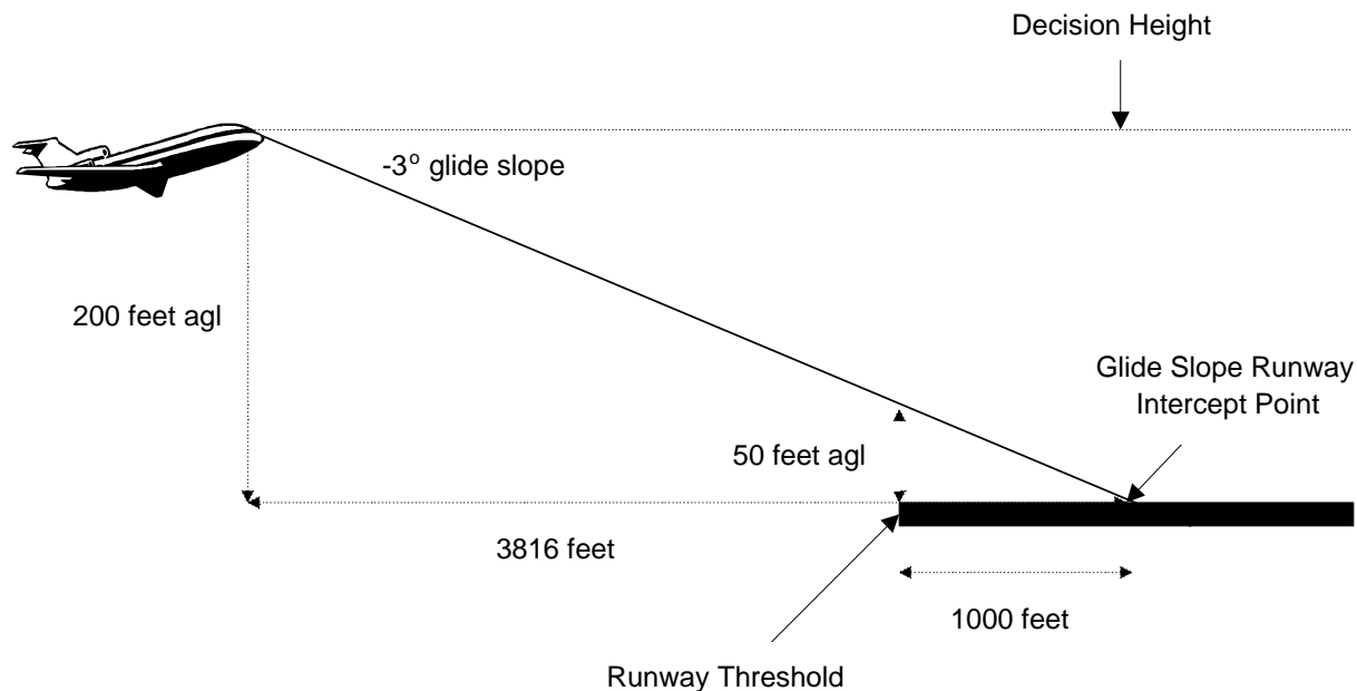
Figure 4.1: Nominal Precision Approach Geometry
