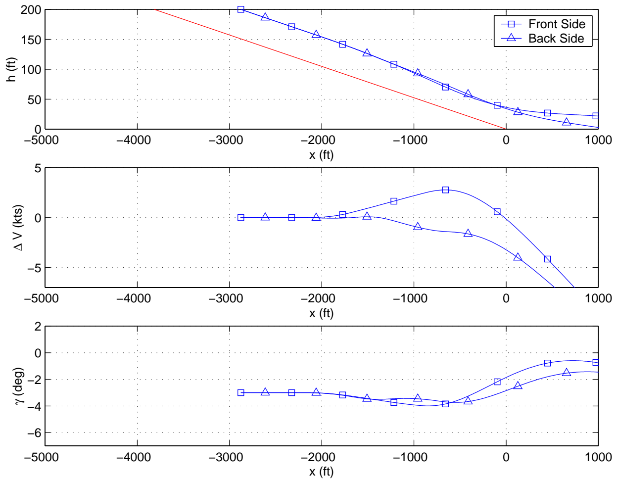
Figure 5.8: Back-Side-Aircraft Response for Long Initial Condition
