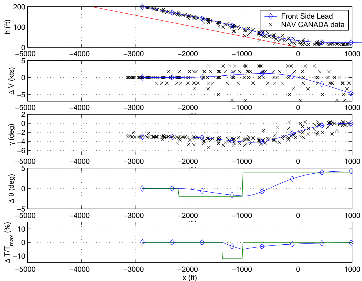
Figure 4.8: Long Initial Condition Response with Lead
