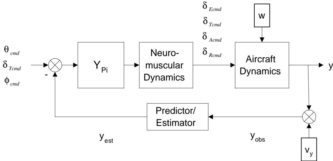
Figure 3.3: VSM Inner Pilot Augmented Loop
