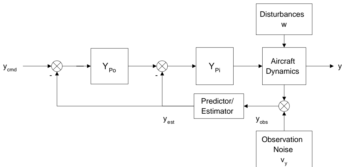
Figure 3.1: Inner/Outer Loop VSM
