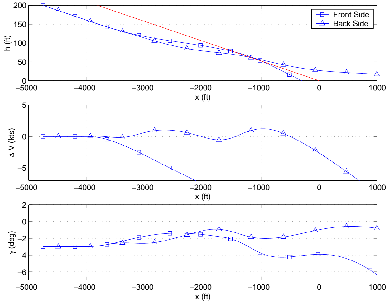
Figure 5.5: Back-Side-Aircraft Response for Short Initial Condition
