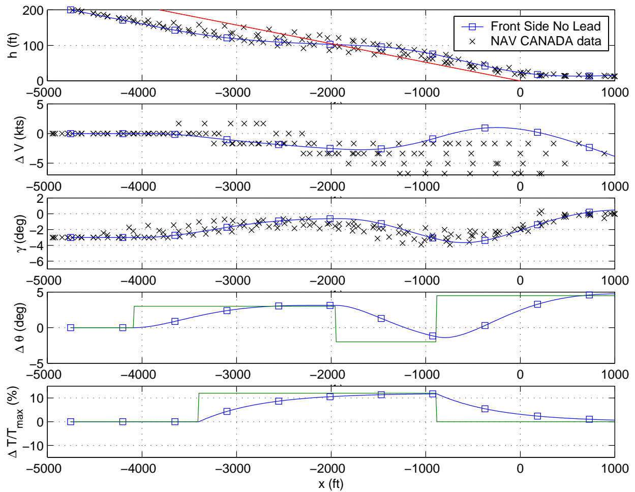
Figure 4.4: Short Initial Condition Response with No Lead
