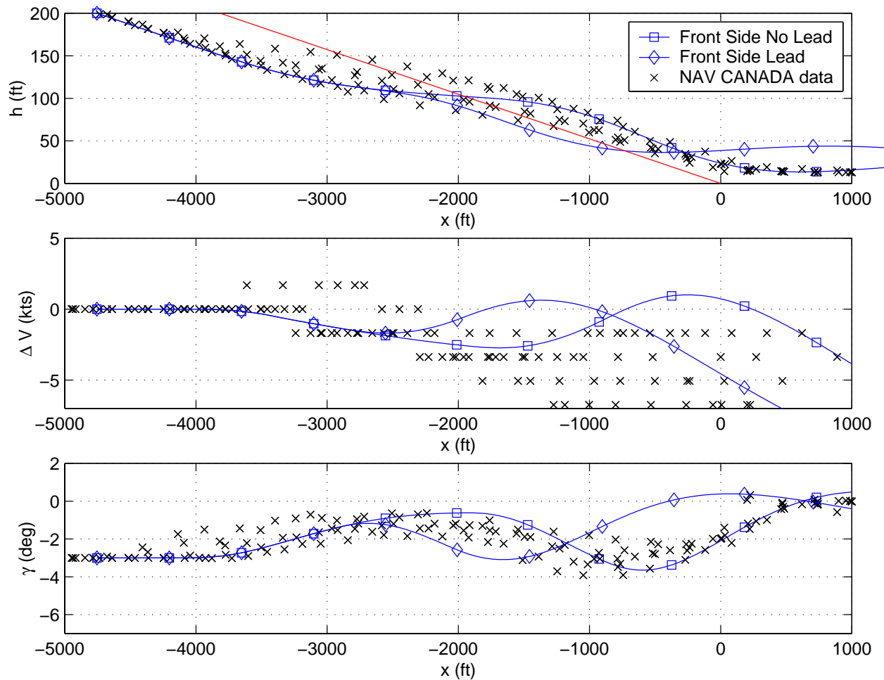
Figure 4.6: Summary Short Initial Condition Response
