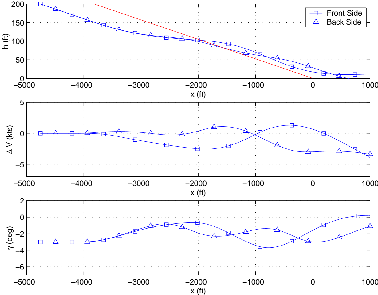
Figure 5.1: Front-Side Aircraft Response for Short Initial Condition
