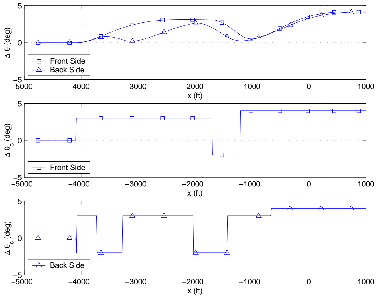
Figure 5.6: Back-Side-Aircraft Pitch Input for Short Initial Condition
