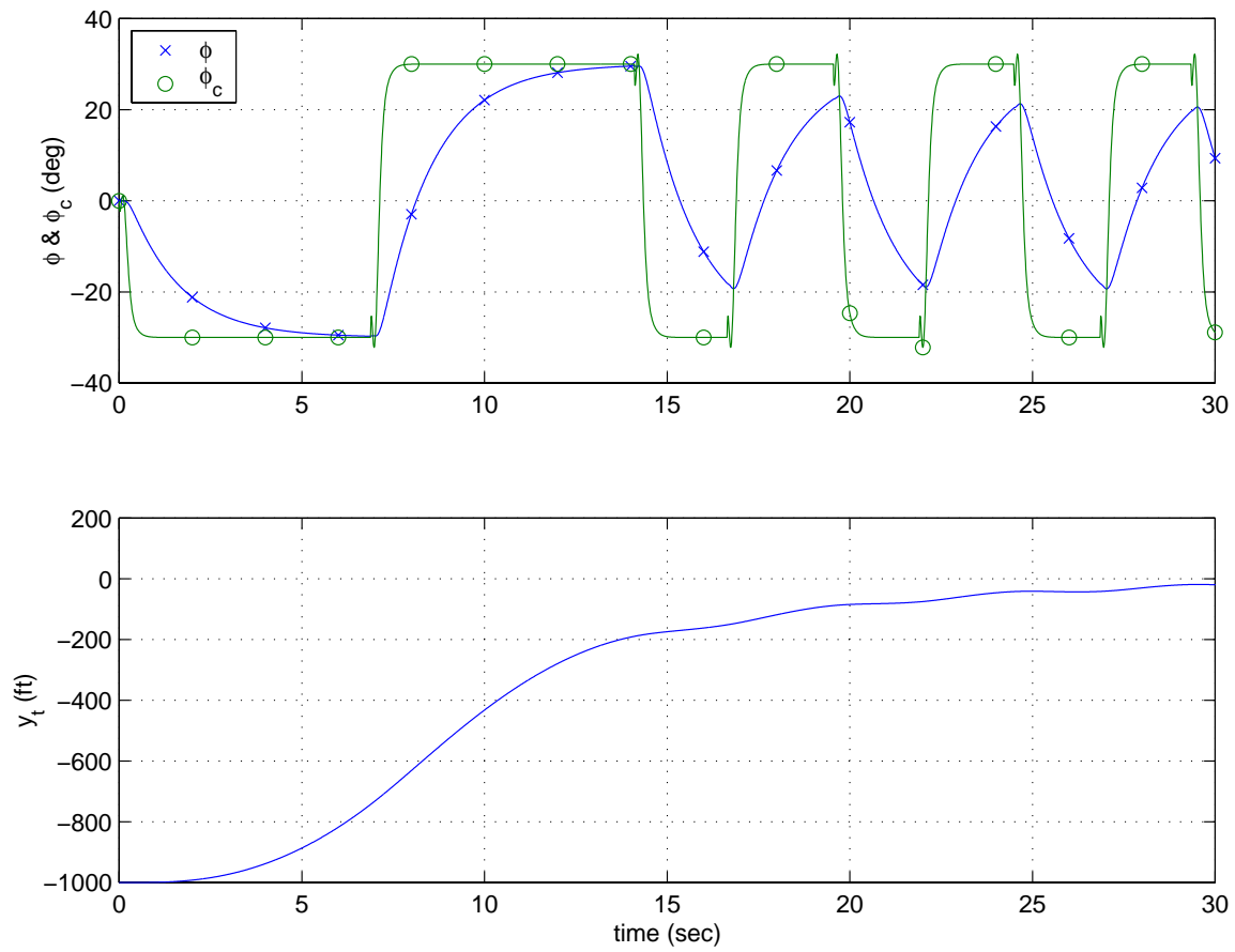
Figure 3.5: Acquisition VSM Time Response
