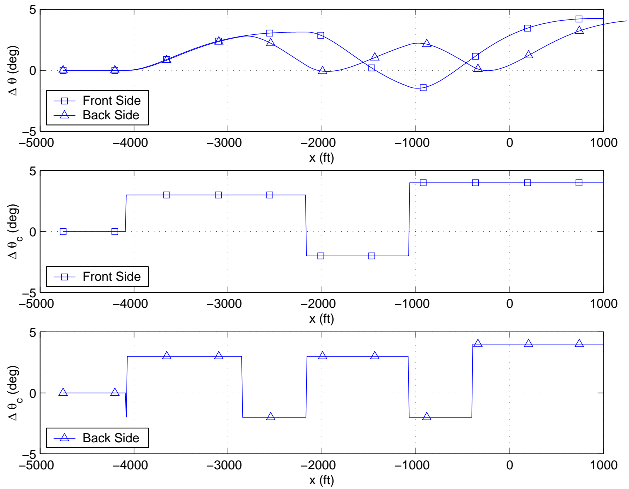
Figure 5.2: Front-Side-Aircraft Pitch Input for Short Initial Condition
