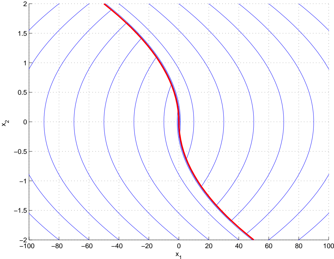
Figure 2.2: Second Order System Bang-Bang Example
