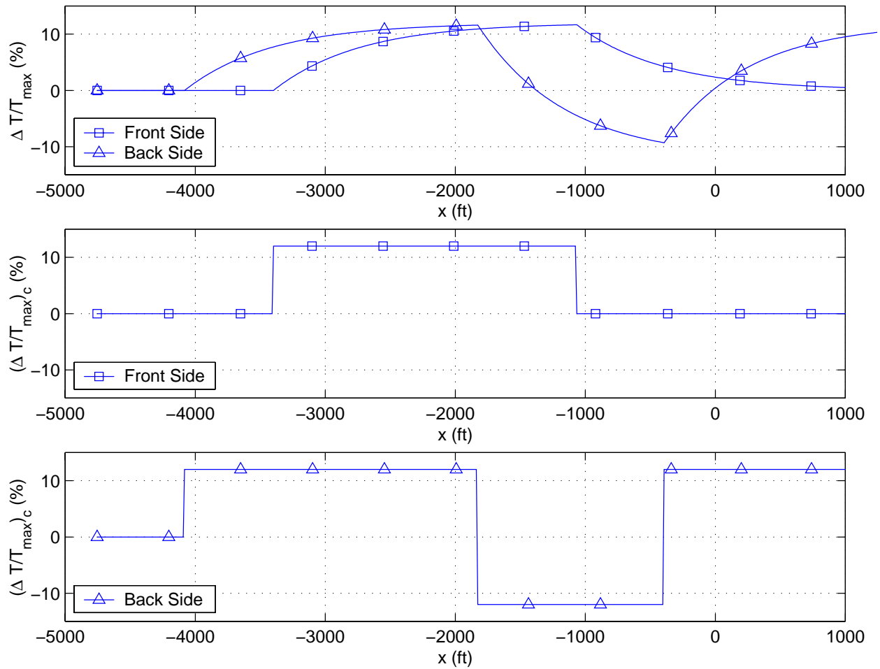
Figure 5.3: Front-Side-Aircraft Thrust Input for Short Initial Condition
