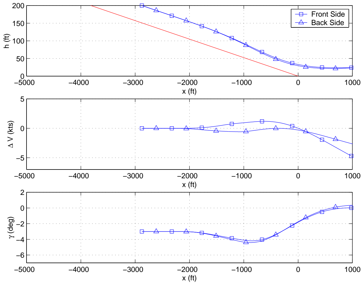
Figure 5.4: Front-Side-Aircraft Response for Long Initial Condition
