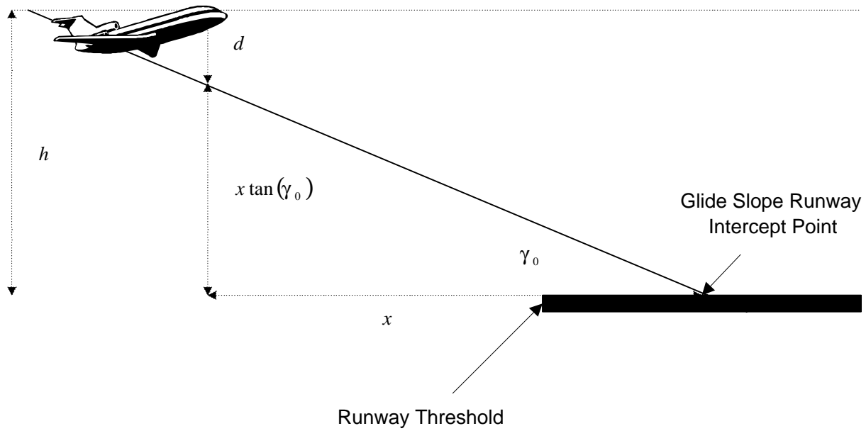
Figure 4.3: Glide Slope Deviation Geometry
