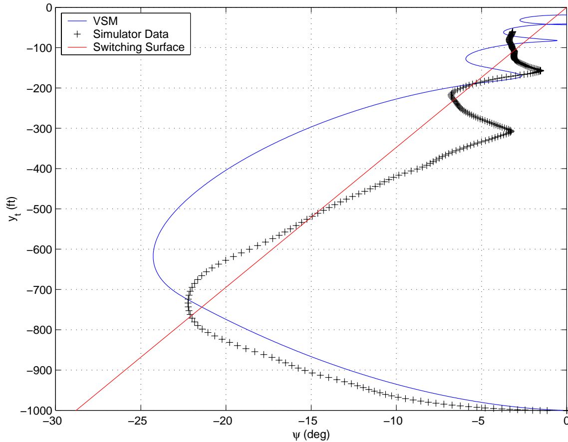
Figure 3.7: Acquisition VSM State Space
