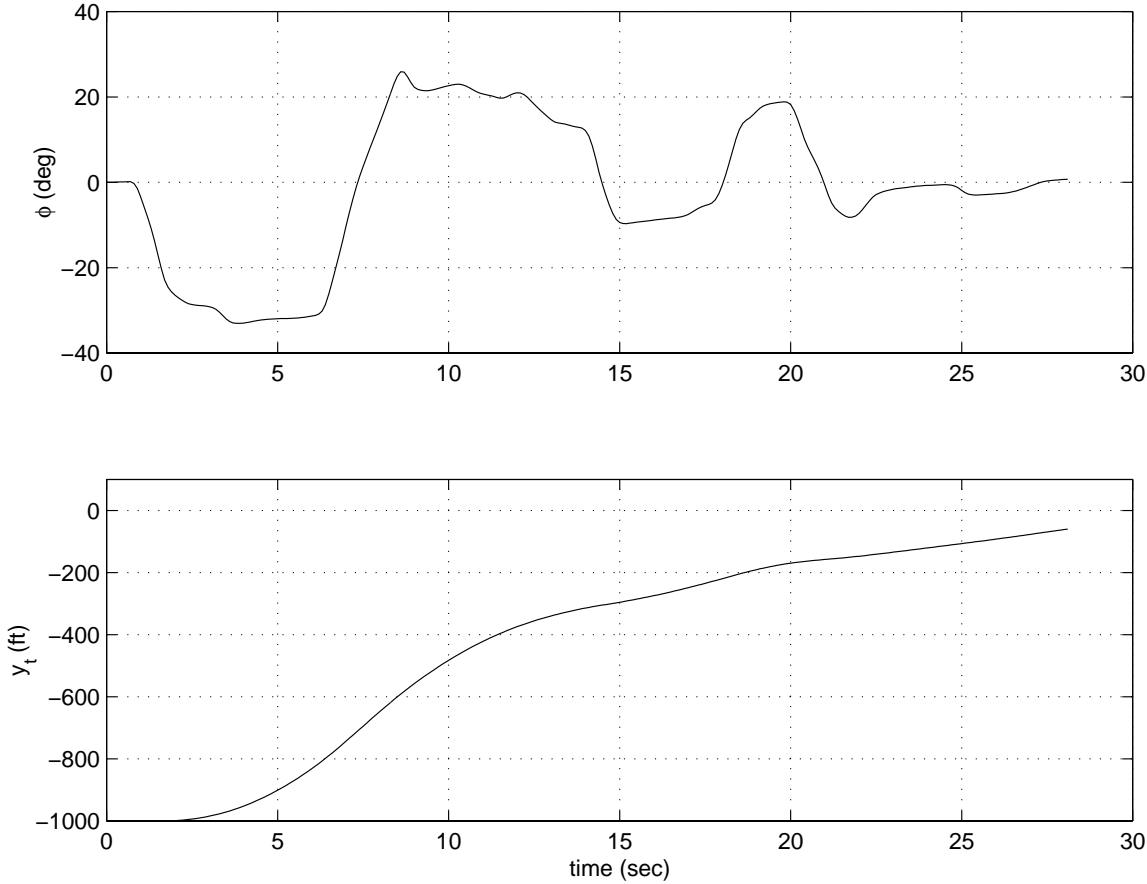
Figure 3.6: Pilot Input/Output Time History
