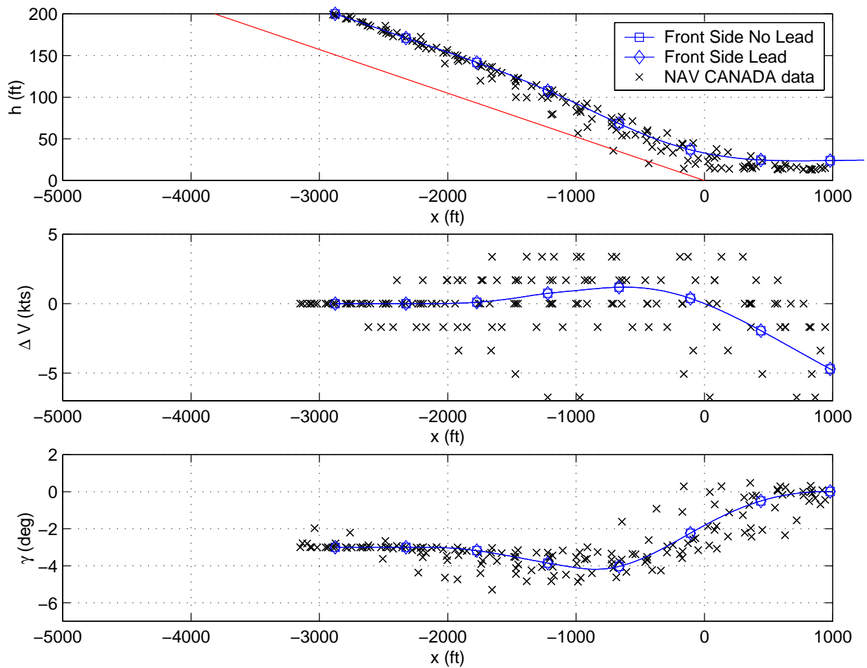
Figure 4.9: Summary Short Initial Condition Response
