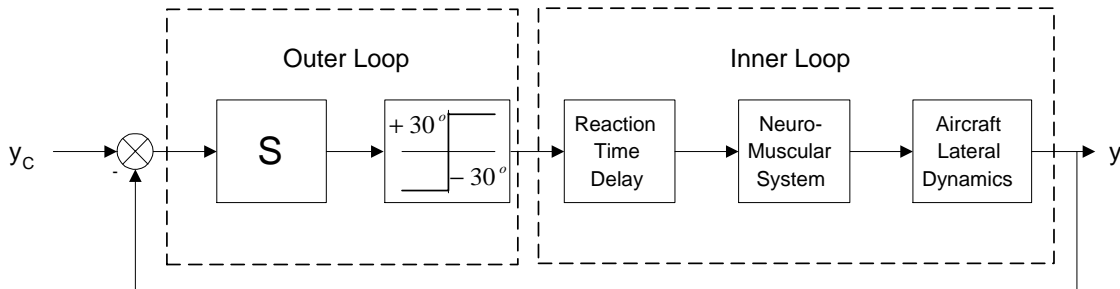
Figure 3.4: Lateral Course Regulation VSM Structure
