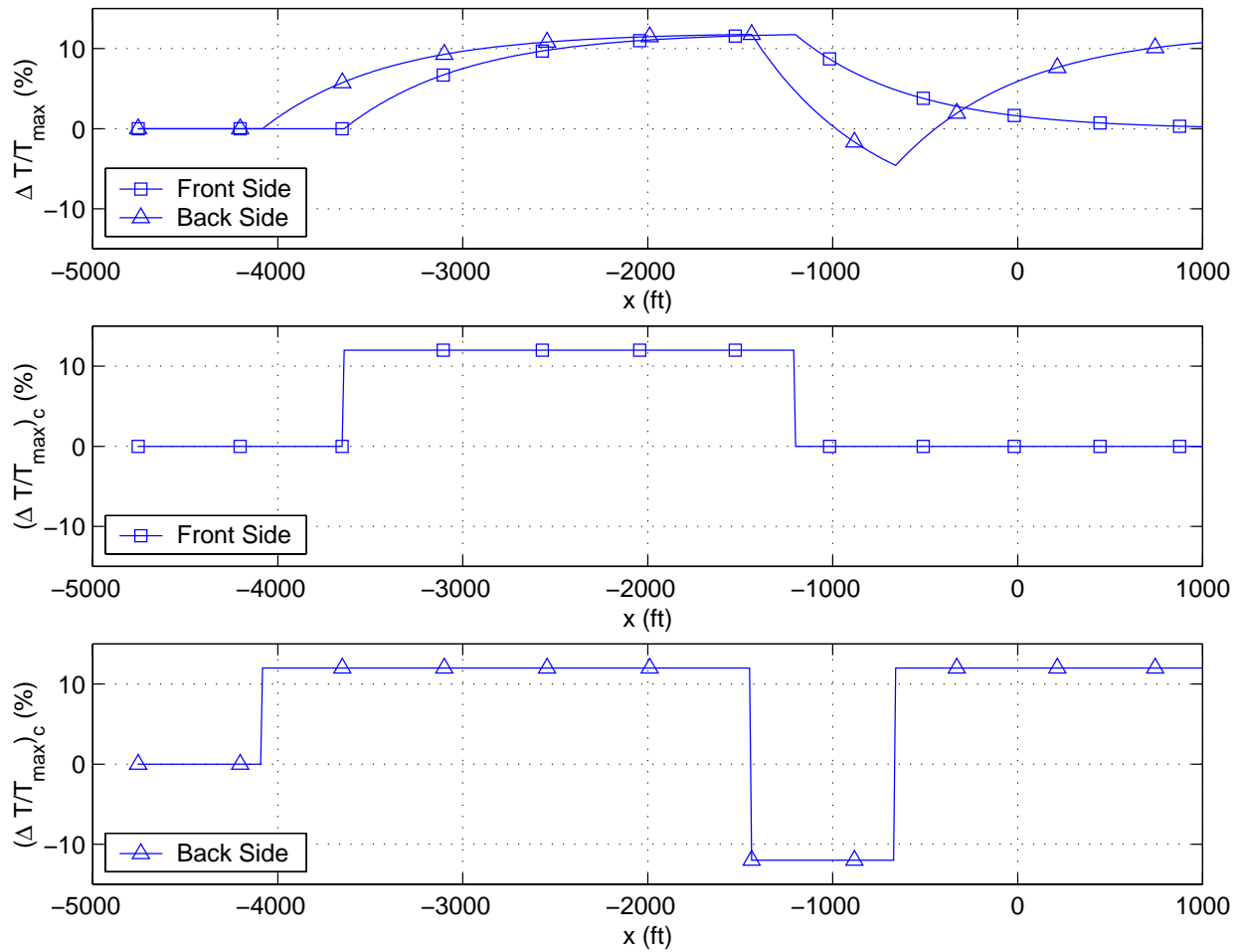
Figure 5.7: Back-Side-Aircraft Thrust Input for Short Initial Condition
