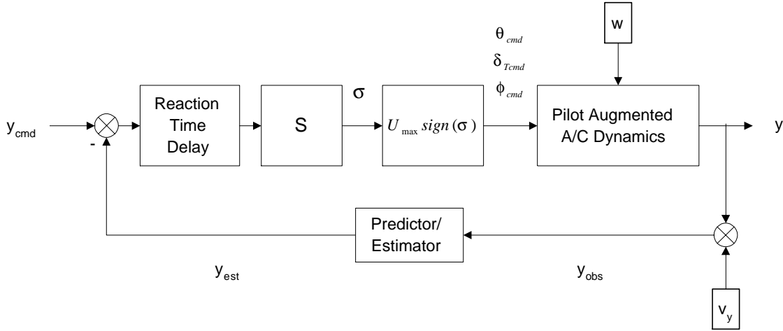
Figure 3.2: VSM Outer Acquisition Loop
