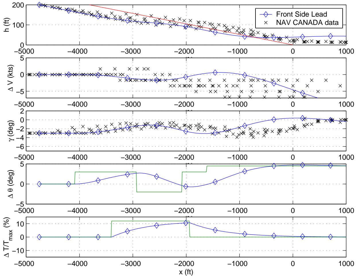
Figure 4.5: Short Initial Condition Response with Lead
