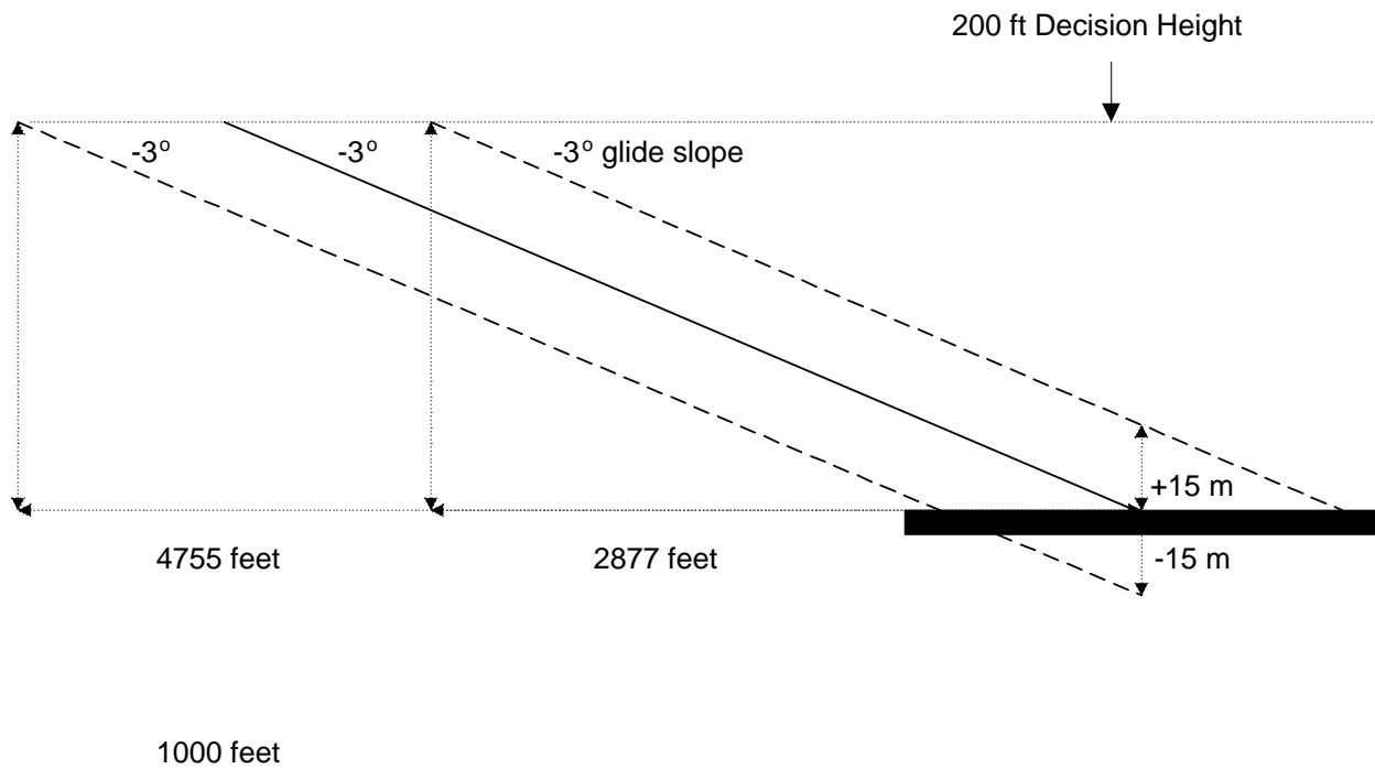
Figure 4.2: Precision Approach Geometry with Vertical Error
