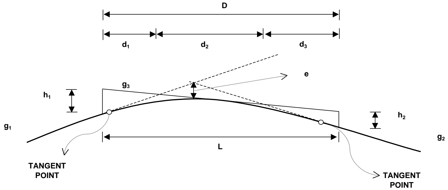
SIGHT DISTANCE GREATER THAN LENGTH OF VERTICAL CURVE
