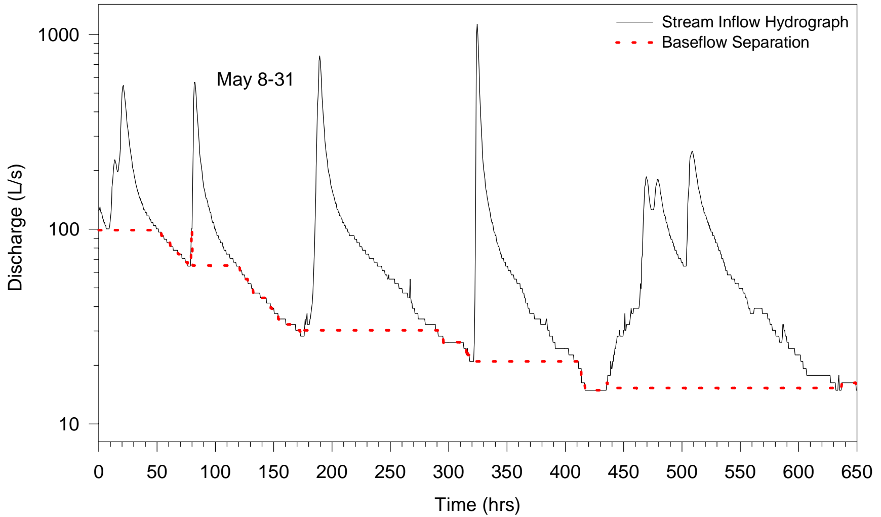
Figure 6. Illustration of the baseflow separation technique used to estimate the runoff component of the discharge hydrograph for May 1996.
