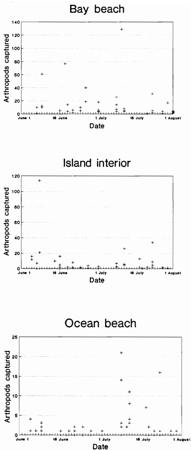
Figure 9. Arthropods captured (30 minute sampling period), by date, on the bay beach, island interior, and ocean beach on Assateague Island National Seashore, Maryland, 1988-1990. Each point represents one sample.
