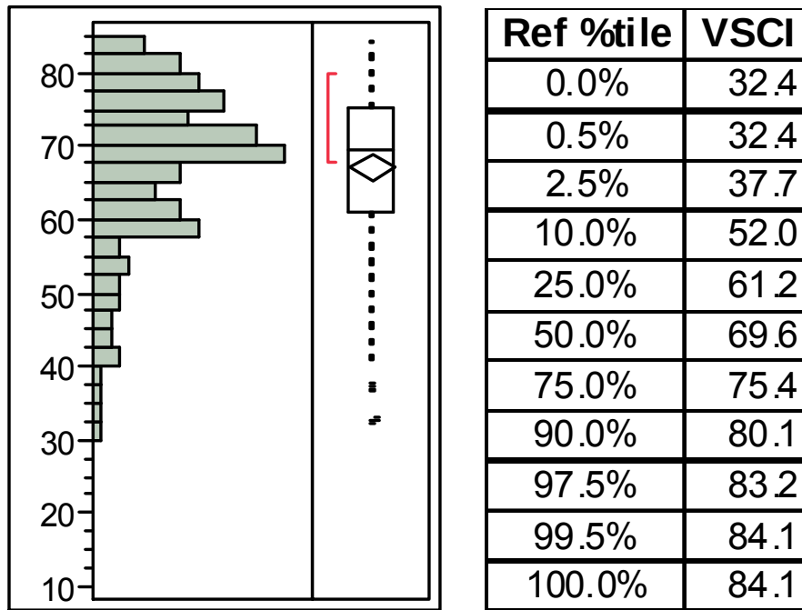
Figure 4. Distribution of SCI within the probabilistic monitoring locations defined through application of the reference-filter conditions of Table 2.
