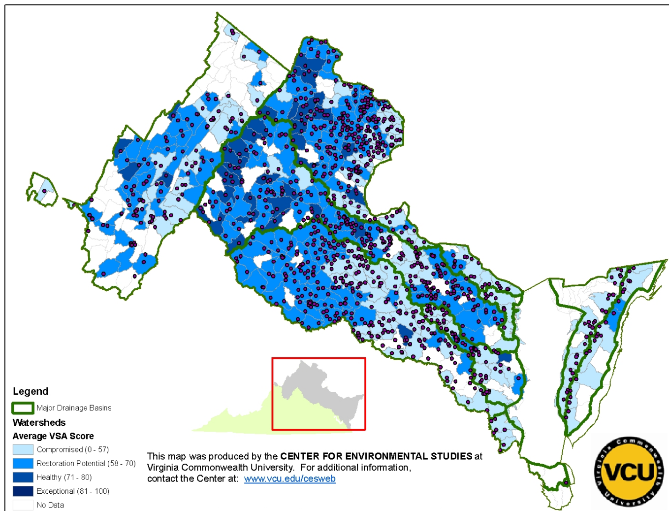
Figure 4. Stream health classification (INSTAR fish assemblage models) for streams in 6 th -order hydrologic units in the Chesapeake Bay basin, Virginia. Categories are based on the mean VSA score (percent comparability to appropriate virtual reference condition). Breakpoints for stream health categories are based on the mean, +/-1 standard error, and + 2 standard errors of the distribution of n=1,033 randomly selected VSA scores for INSTAR stream reaches. HUCs in the 'exceptional' and 'healthy' categories are dominated by streams exhibiting high ecological integrity. Points represent individual quantitative (electrofishing) collections for selected HUCs.
