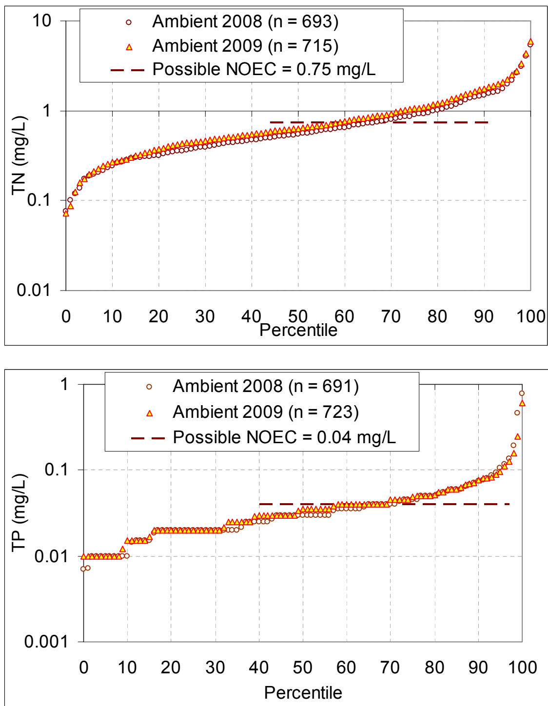
Figure 10. Distribution of DEQ ambient water monitoring sites, by TN (above) and TP (below) median concentrations for 2008 and 2009.
