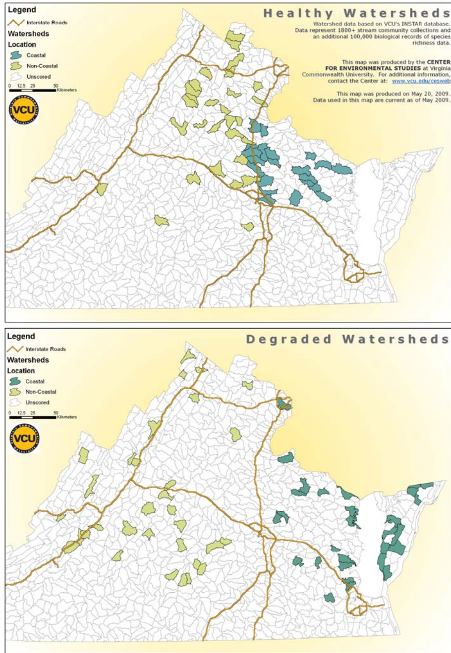
Figure 5. Watersheds (6 th -order HUCs) classified as 'healthy' or 'degraded' based on INSTAR assessment of fish community data. Refer to the text for a more detailed explanation.
