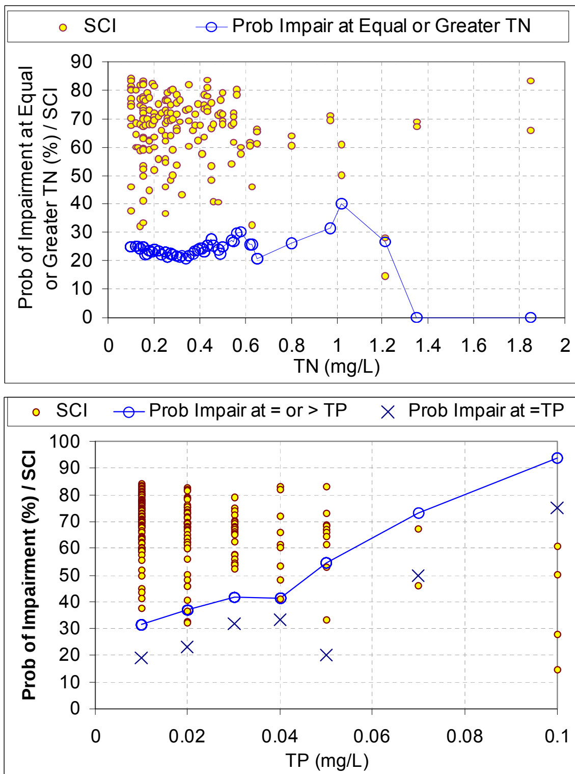
Figure 5. Reference-filtered subsets of 2001-2008 Probmon defined by applying all of the Table 1 and Table 2 reference filters except the TN and TP filters. Data are plotted as raw SCI concentrations; and as probabilities of impairment (SCI<60). See AAC (2009) for further explanation of the “Probability of Impairment” plotting and analysis method.
