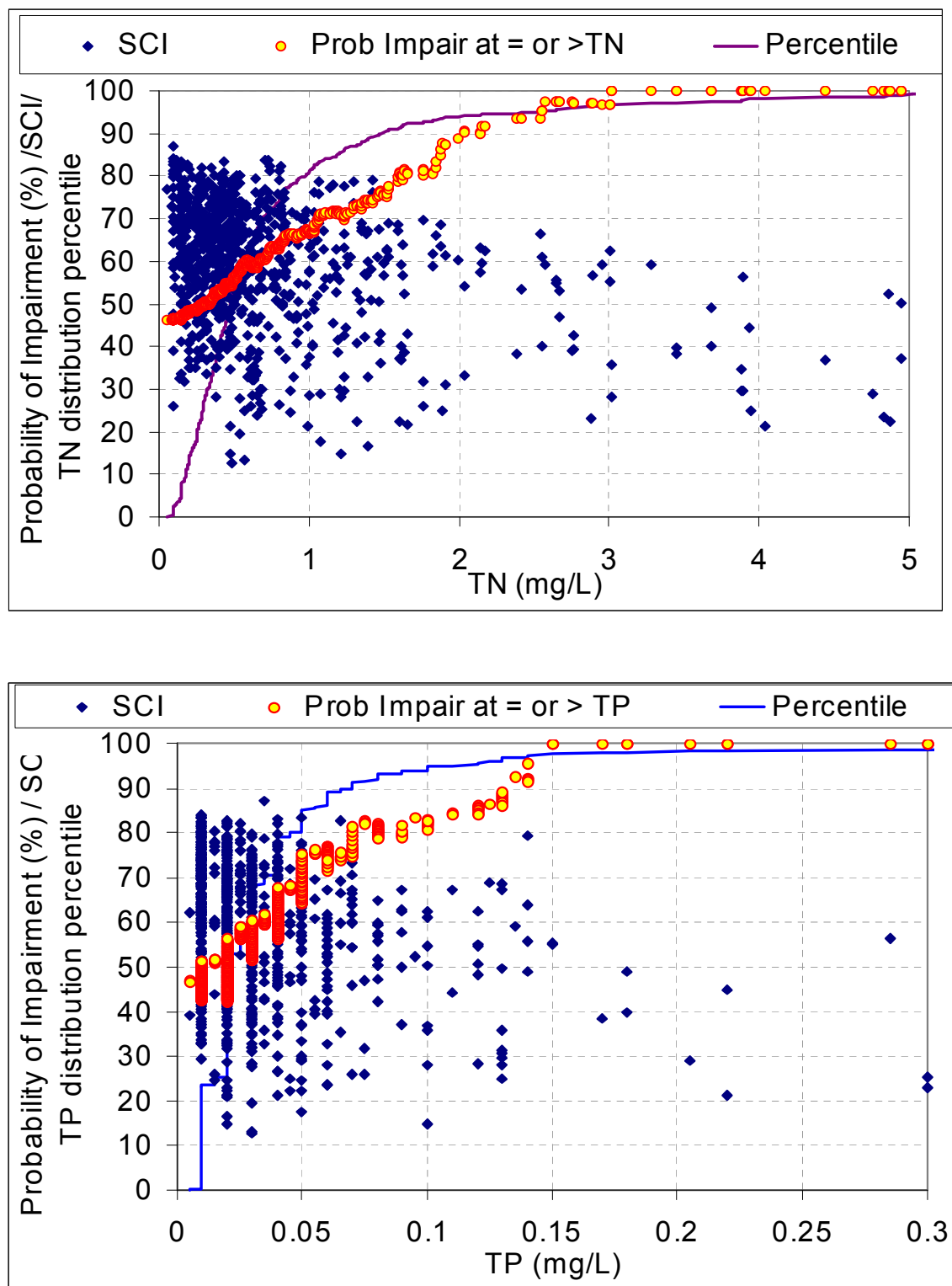
Figure 6. Nutrient concentrations vs. SCI (blue diamonds), and probability of SCI<60 impairment at equal or greater concentrations (red circles). Percentile distributions of nutrient concentrations are also plotted as solid blue lines. Probmon 2001-2008 data are plotted for TN (above) and TP (below). Several very high concentrations for both TN and TP, at impaired sites, are not shown.
