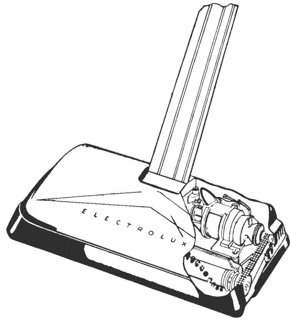
Power nozzle - Electrolux.
