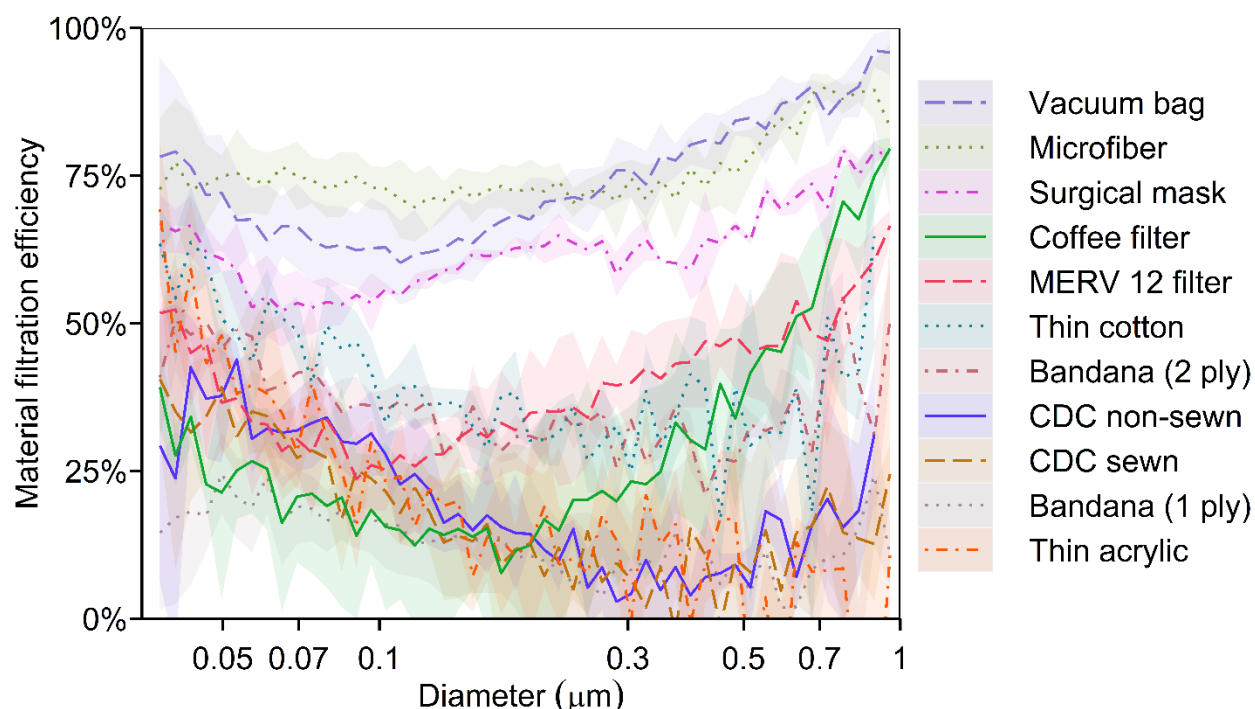
Figure 3-4. Material filtration efficiency of 10 mask materials as a function of aerodynamic diameter. The bandana appears twice because it was tested in both 1-ply and 2-ply configurations. Shading represents the standard deviations of triplicates.
