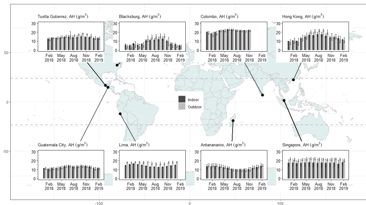
(c) Monthly absolute humidity
