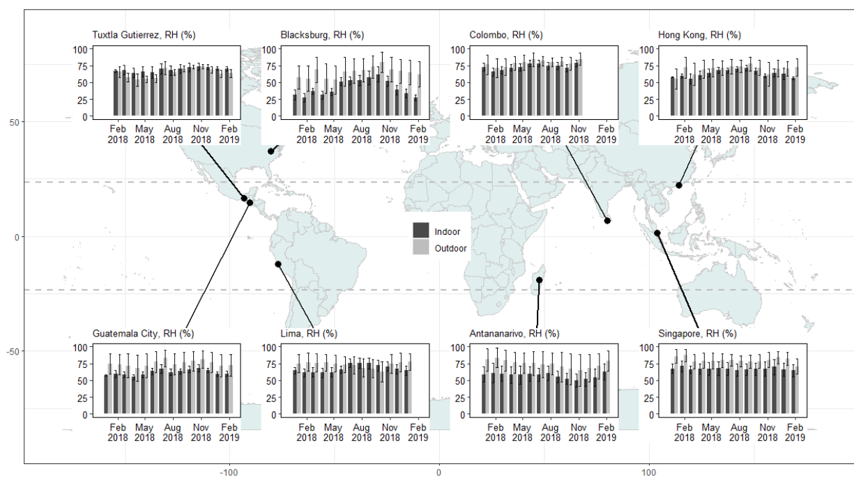
(b) Monthly relative humidity
