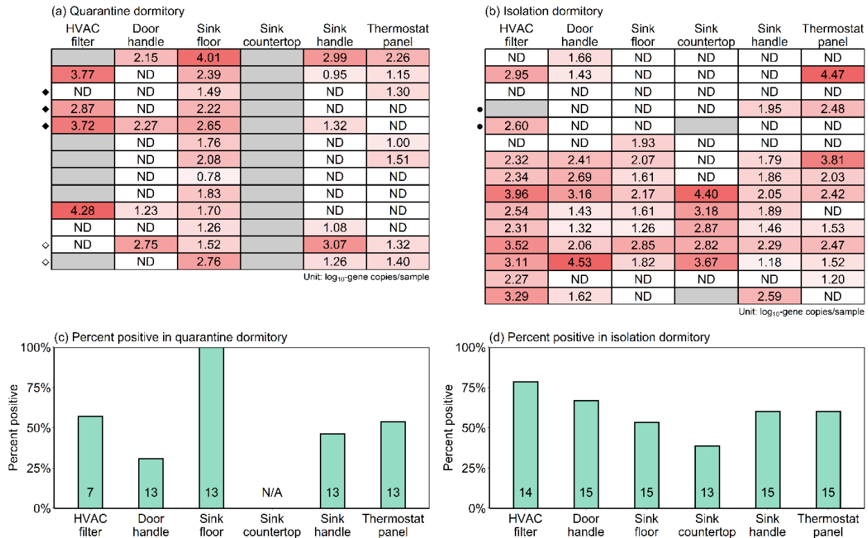
Figure 2-1. log 10 SARS-CoV-2 RNA gene copies per swab or 3×8 cm 2 HVAC filter piece in the (a) quarantine dormitory and (b) isolation dormitory. Each row represents one room. Rows with shared symbols indicate that these rooms were the same room sampled at different points in time following occupancy by different individuals. Red shading indicates log 10 -gene copies per sample; white with “ND” means “not detected”; gray means “not collected” for the sink countertop or “not available” for the HVAC filters. Percentage of positive samples for each type of sampling site in the (c) quarantine dormitory and (d) isolation dormitory. The numbers at the bottom of each column indicate the number of samples.
