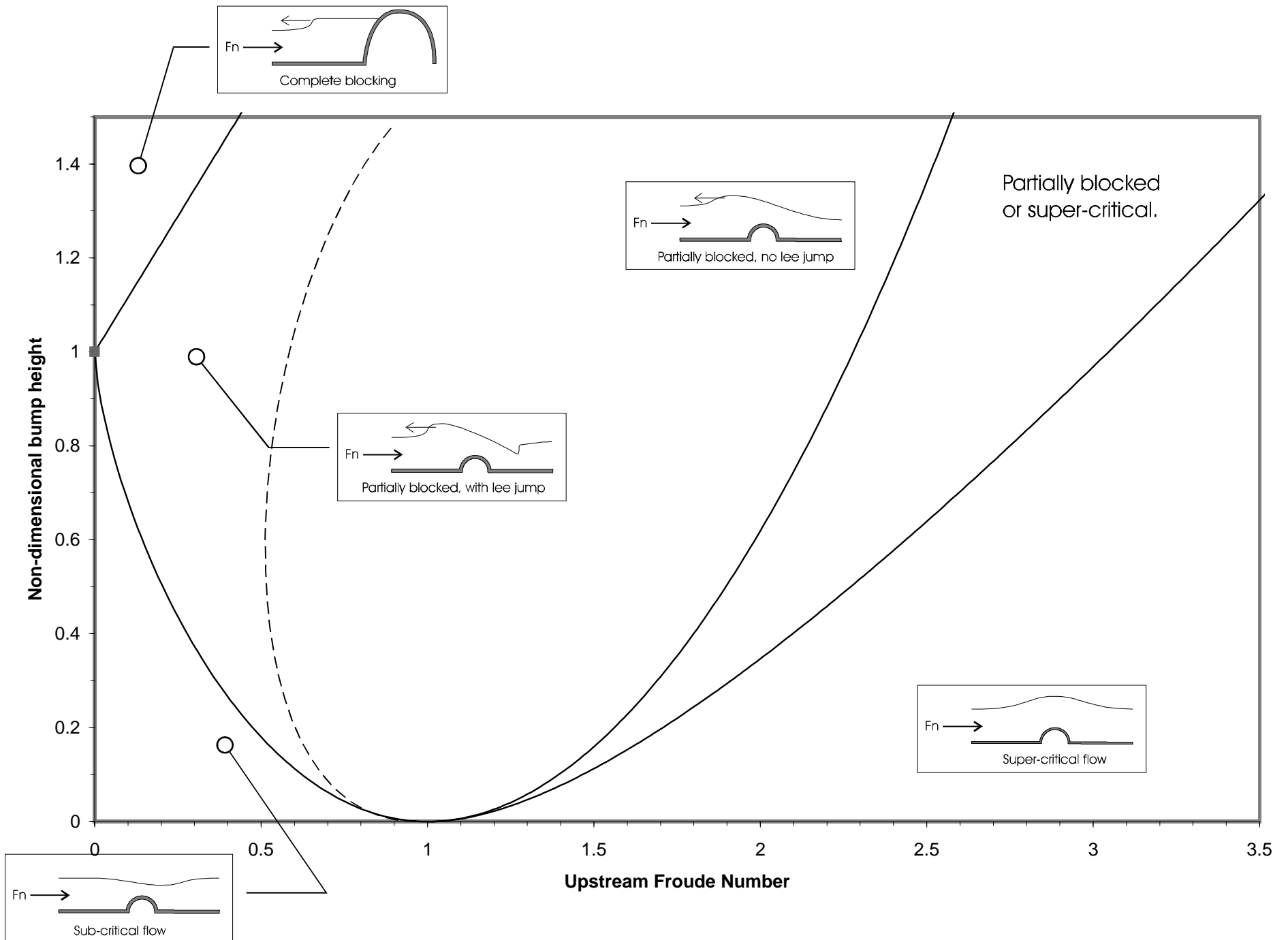
Figure II-1: The steady state flow regimes.
