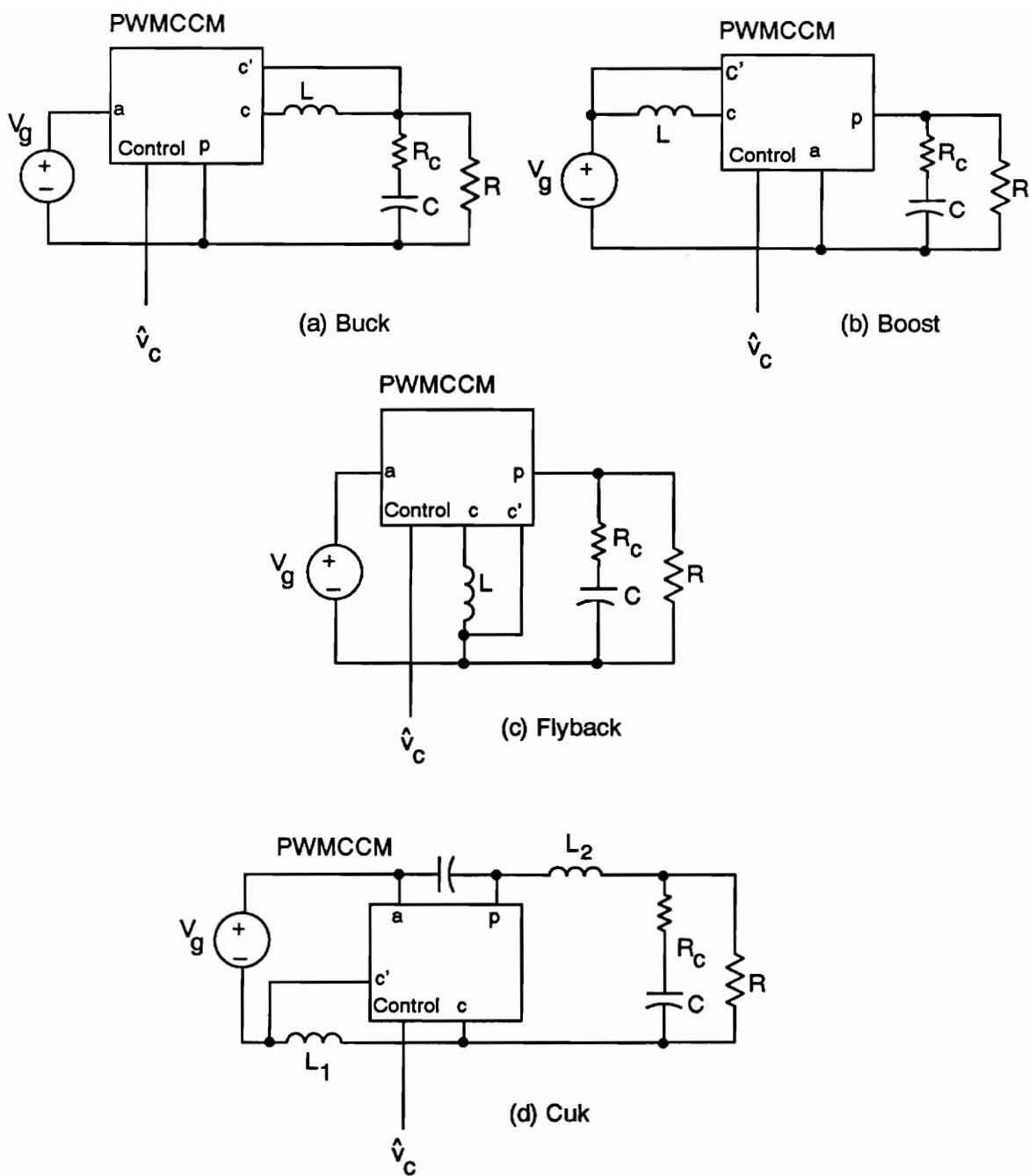
Figure B.3. Small-Signal Controller Placed in Different Converters: Connections of the controller of Fig. B.1 in four types of PWM circuits are shown. Care must be taken with polarities of current sensing for the boost converter, and with the correct value of equivalent inductance for the Cuk converter.
