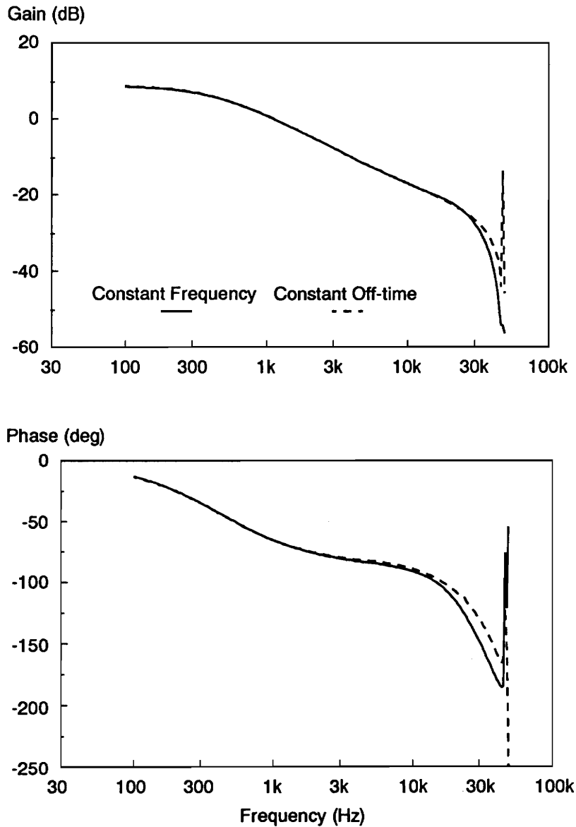
Figure 5.20. Control-to-Output Measurement for Constant-Frequency and Constant Off-Time, D=0.1 : For very low duty cycles, these transfer functions are almost identical. The phase lead introduced by the modulator is small at low duty cycles, less than 10^\circ at half the switching frequency. Like the constant-frequency control system, this transfer function has a pair of poles at half the switching frequency. These poles have a fixed Q of 2/\pi , regardless of duty cycle.
