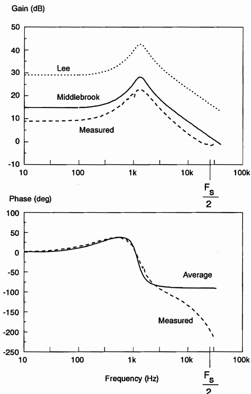
Figure 2.16. Predictions of Current-Loop Gain Transfer Function: Significant differences in measured results and predictions of two averaged models are shown here. Notice that both of the average models would indicate that the current-loop crossover frequency can exceed the Nyquist frequency of the system, yet still remain stable.
