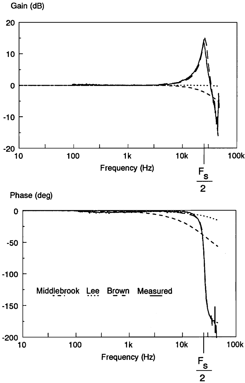
Figure 2.15. Predictions of Control-to-Inductor Current Transfer Function: The control-to-inductor-current transfer function is plotted here for two of the average models, [16] and [18], and the sampled-data model of [29]. The significant deviations of the average models and the observed results at half the switching frequency are apparent.
