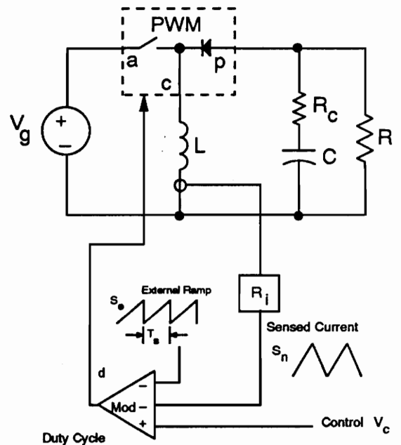
(c) Buck-Boost
