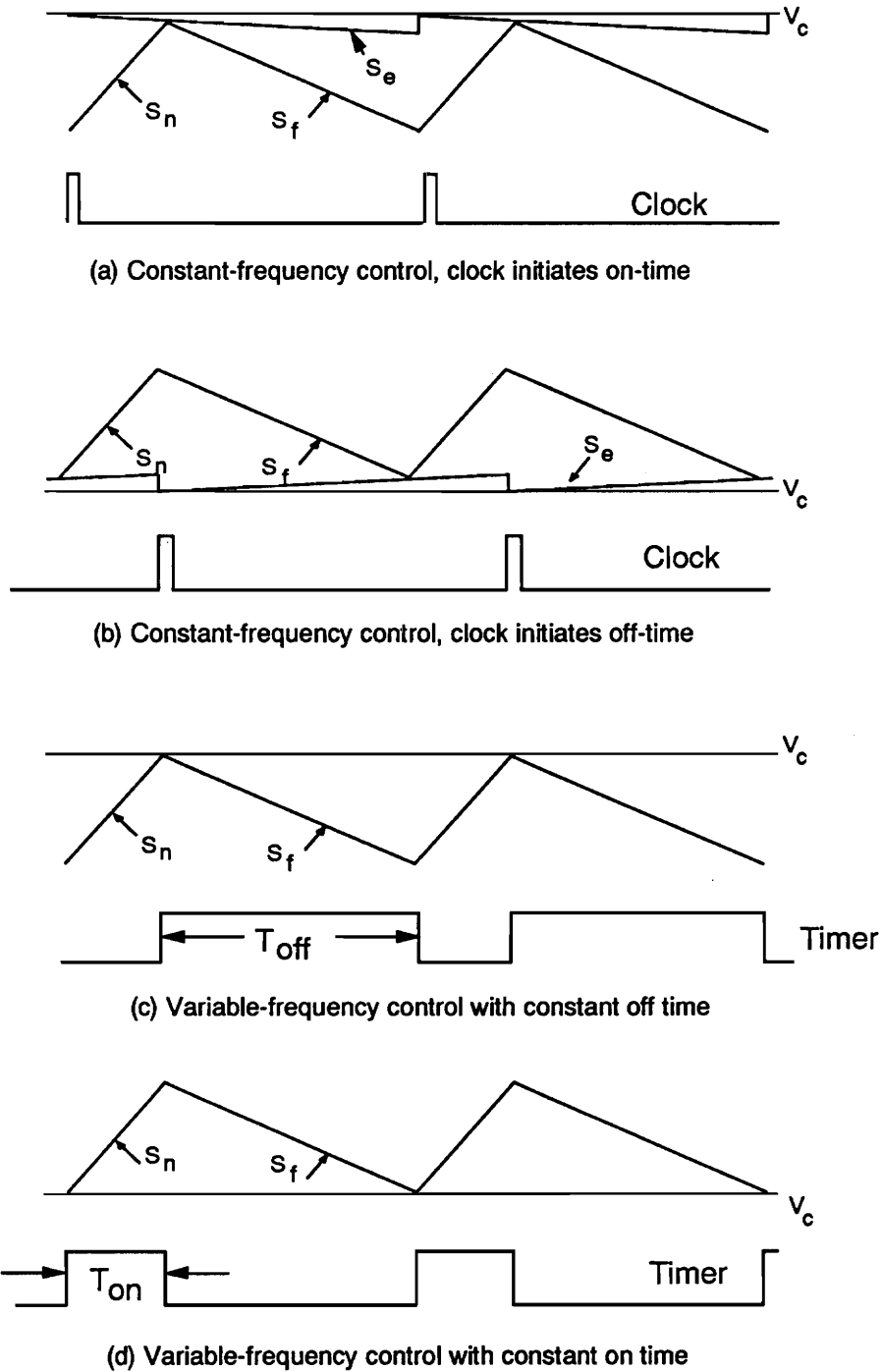
Figure 2.6. Different Modulation Schemes for Current-Mode Control: Four of the many possible modulation schemes are shown in this figure. Constant-frequency control with a clock initiating the on-time of the power switch is the most commonly-used approach.
