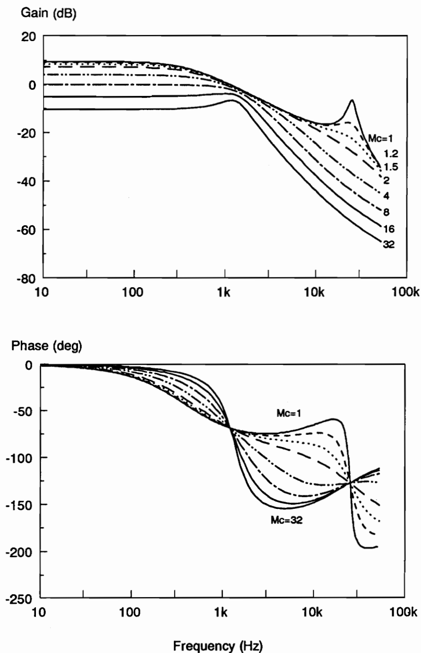
Figure 5.7. Control-to-Output Transfer Function with Current-Loop Closed: The low phase margin in the current loop of the system with small external ramp is manifested in the control-to-output transfer function by a pair of complex poles at half the switching frequency. The Q of these poles is controlled by the addition of the external ramp.
