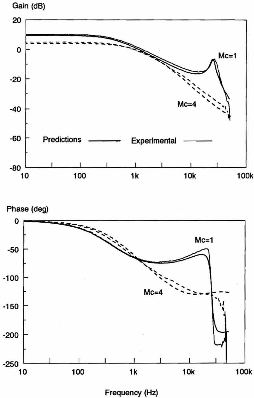
Figure 5.11. Control-to-Output Transfer Function - Experimental Results: The very high Q with no current ramp was accurately predicted by the model, and matched by the experimental results. Increase of the parameter m_c beyond a value of 4 was impractical on the experimental converter due to the limited supply voltage to the current-mode comparator. Larger values of m_c require too large an external ramp.
