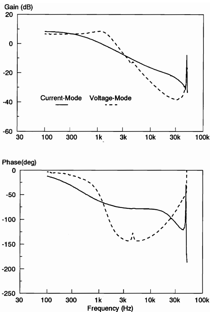
Figure 5.23. Control-to-Output Measurement for Voltage-Mode and Current-Mode Control: The modulator phase characteristics also affect voltage mode control, obtained when the current sense resistor, R_i , is zero. The intersection of the phase of the current-mode system and the voltage-mode system at half the switching frequency is further experimental confirmation of the existence of the double pole at half the switching frequency in the current mode transfer function.
