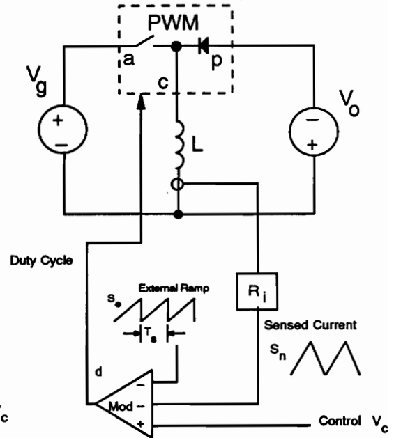
(c) Buck-Boost
