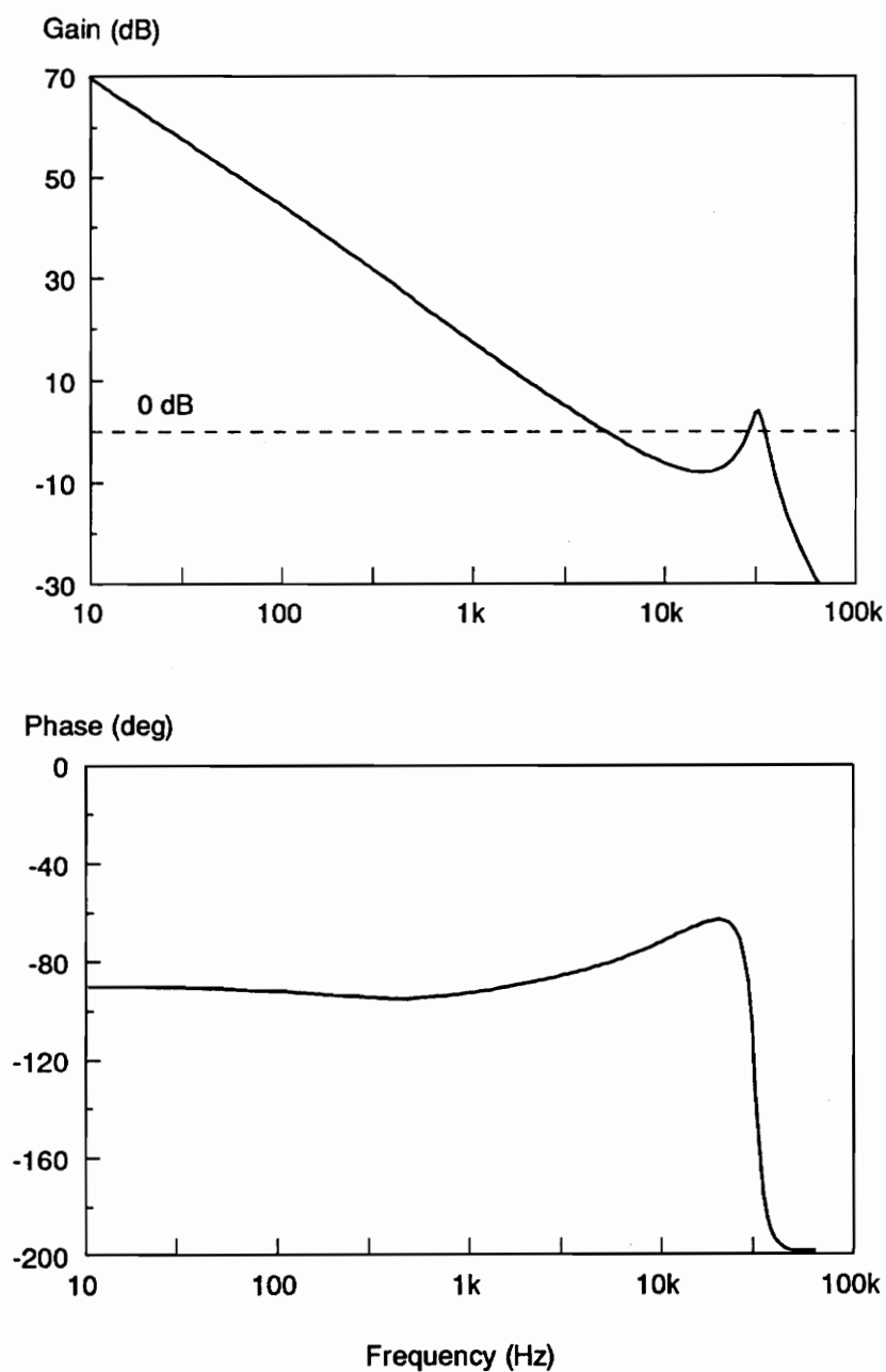
Figure 5.10. Loop Gain of Buck Converter without an External Ramp: If the high- Q poles of the system are not damped with an external ramp, introduction of outer-loop feedback can make the system unstable, even at duty cycles considerably less than 0.5.
