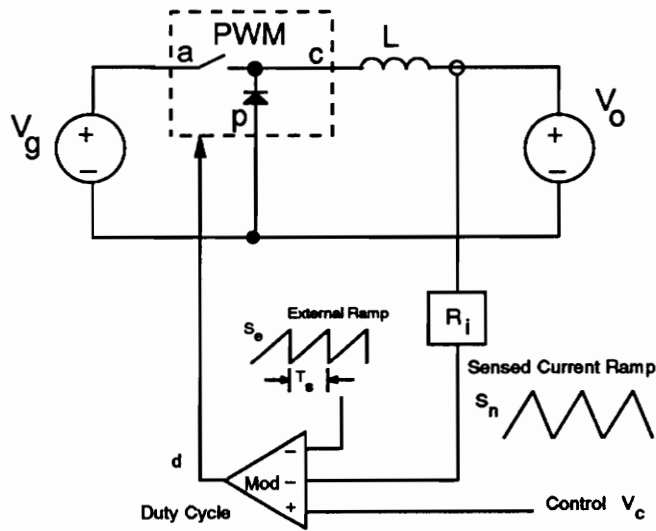
(a) Buck
