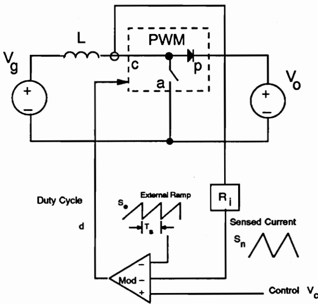
(b) Boost
