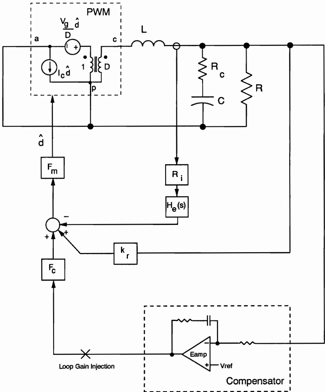
Figure 5.9. Buck Converter with Feedback Compensator and No External Ramp: With no external ramp, addition of a compensation network can cause the previously-stable current loop to oscillate. The loop gain of this system, measured at the output of the compensator, shows the cause of the instability.
