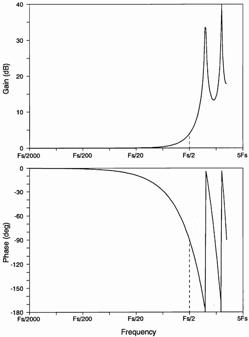
Figure 4.1. Exact Transfer Function for Sampling Gain: At half the switching frequency the gain has increased by about 4 dB, and the phase shows exactly 90^\circ lag. High- Q poles are apparent at the switching frequency and twice the switching frequency.
