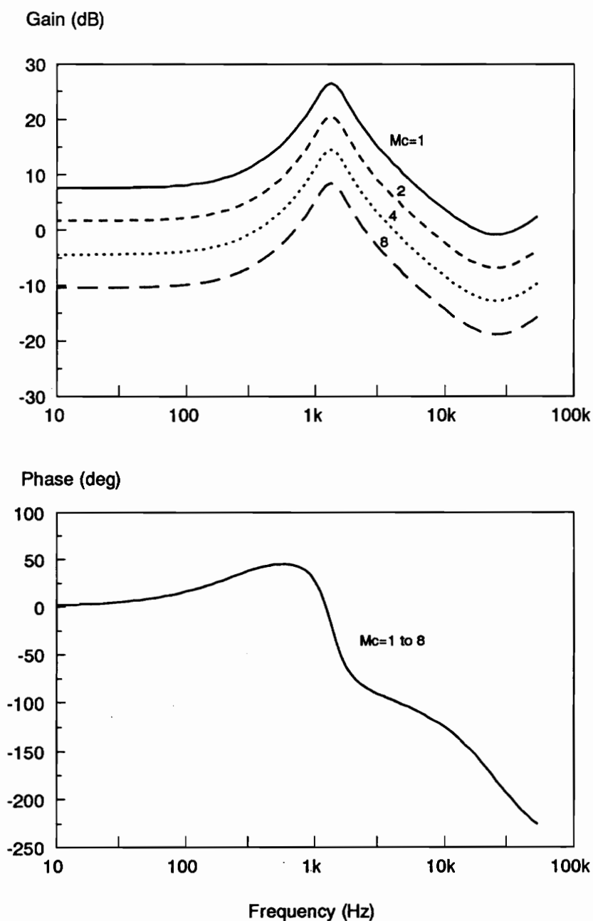
Figure 5.4. Buck Converter Current Loop Gain: This figure shows the effect of the RHP zeros of H_e(s) on the current loop stability. At half the switching frequency, the phase of the current loop is -180 degrees, and the system is unstable with too much gain. The gain of the current loop is reduced by adding an external ramp to the system.
