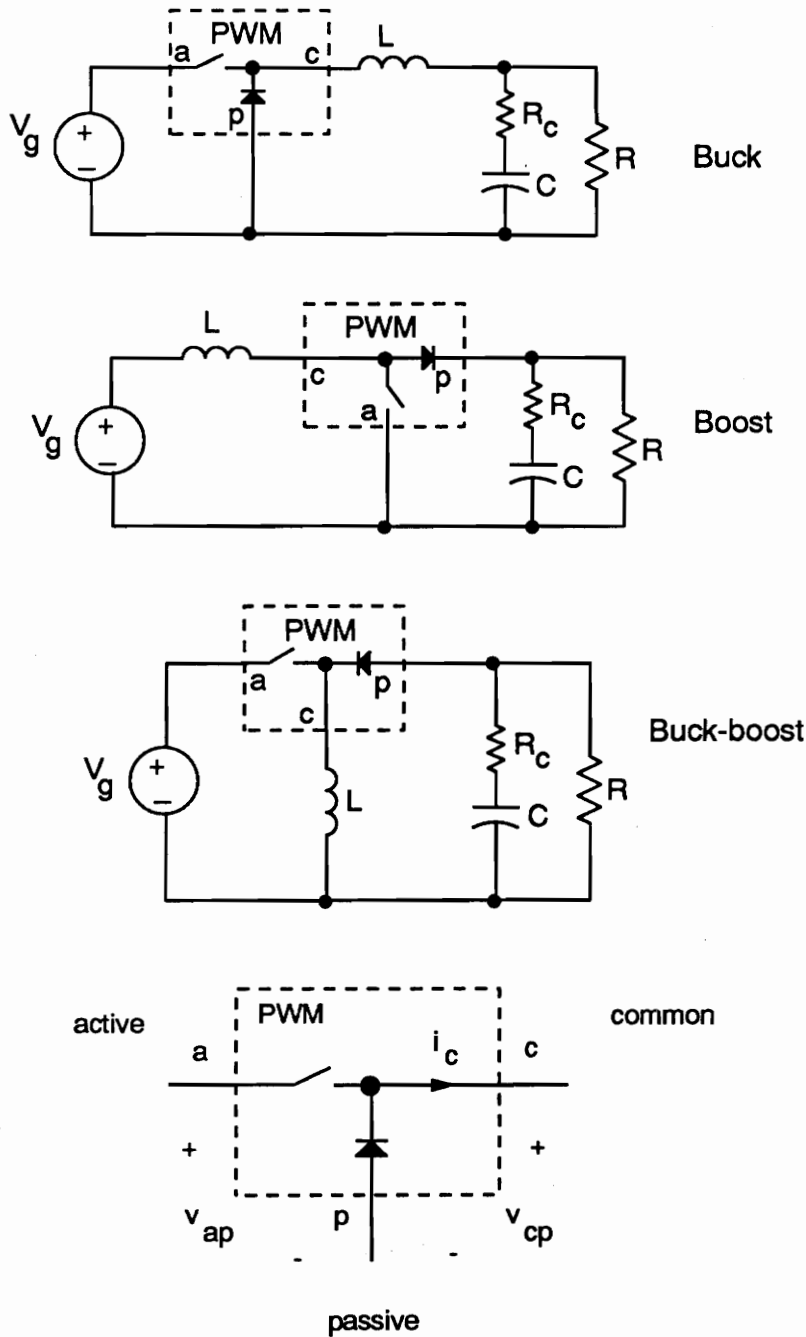
Figure 2.8. Basic Converters with Switch Definitions: An invariant nonlinear block can be identified for most PWM converters. The terminal with the controlled switch is called the active terminal, the diode is connected to the passive terminal, and the inductor is connected to the common terminal. The diode orientation will change according to the polarity of the common terminal current.
