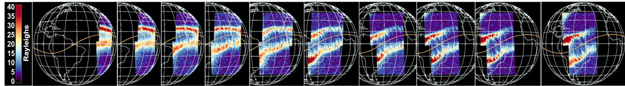
Figure 9. Typical sequence of nightside scans, example from 17 October 2018. The longitude ranges scanned in the Northern and Southern Hemispheres are selected to avoid locations illuminated by the Sun while observing near the terminator. Bubbles, seen most prominently on the equatorward edges of the EIA crests, are typical near equinox.
