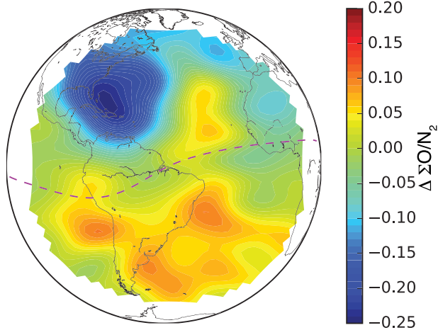
Figure 4. Difference in column density ratios ( \Delta\Sigma\text{O}/\text{N}_2 ) retrieved from GOLD observations at 14:40–15:10 UT (11:30–12:00 satellite LT) on 14 May 2019 from previous day. The largest decrease occurs near the largest temperature increases in Figure 3b, but the morphology differs.
