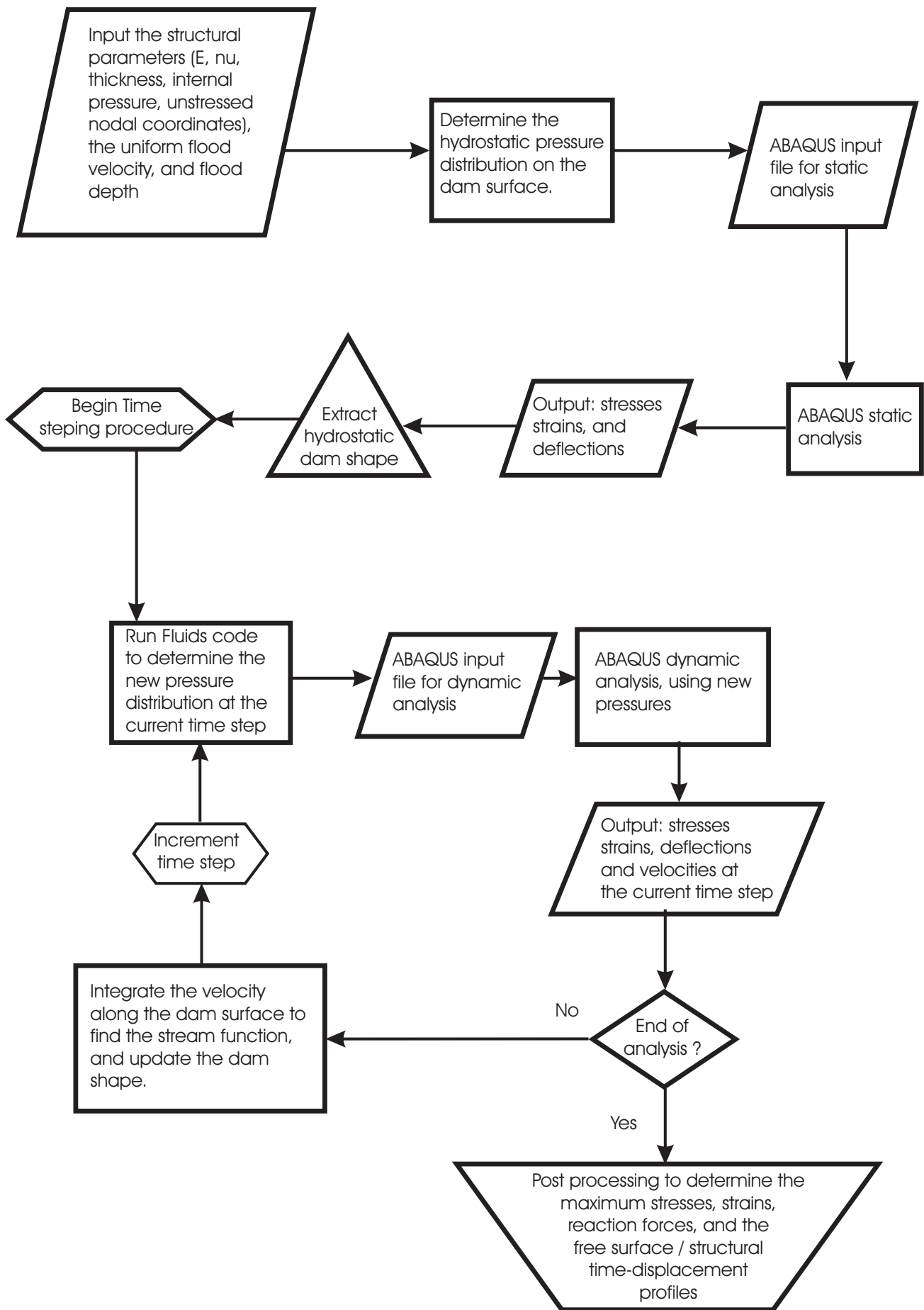
FIGURE I-3: FLOW CHART OF THE SOLUTION METHOD FOR THE NO OVERFLOW CASE
