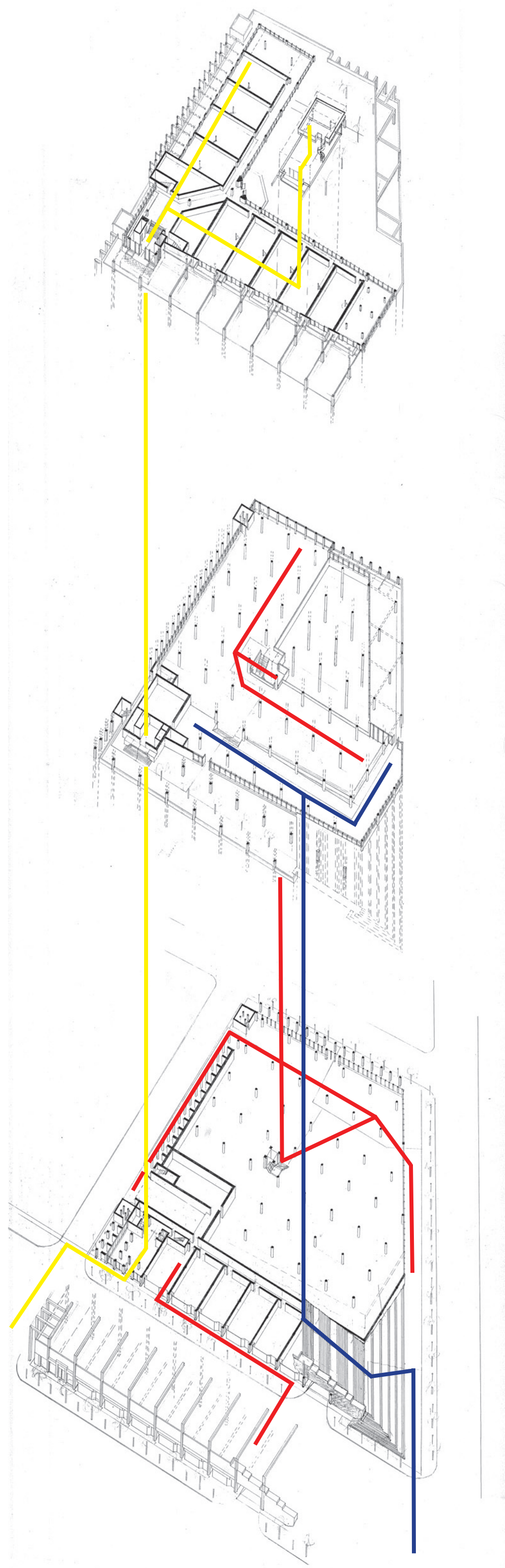
building axonometric
