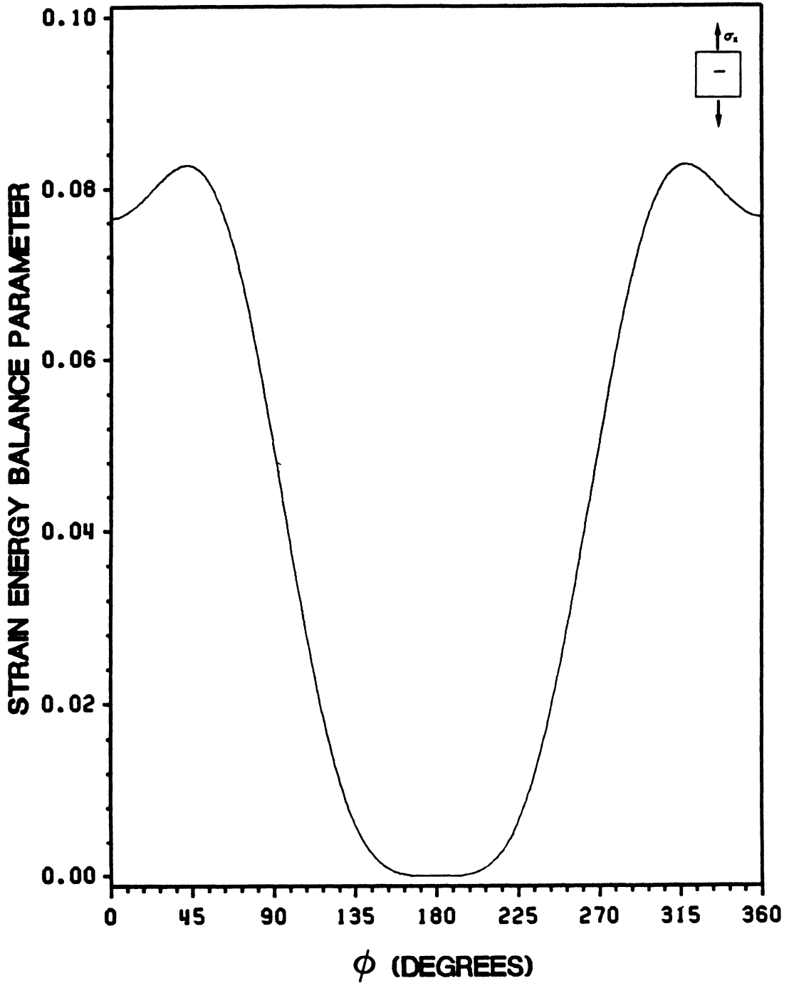
Figure 32. Strain Energy Balance Parameter vs. \phi for Mode I Isotropic Fracture: Center-Notched Infinite Plate of 6061-T6 Aluminum
