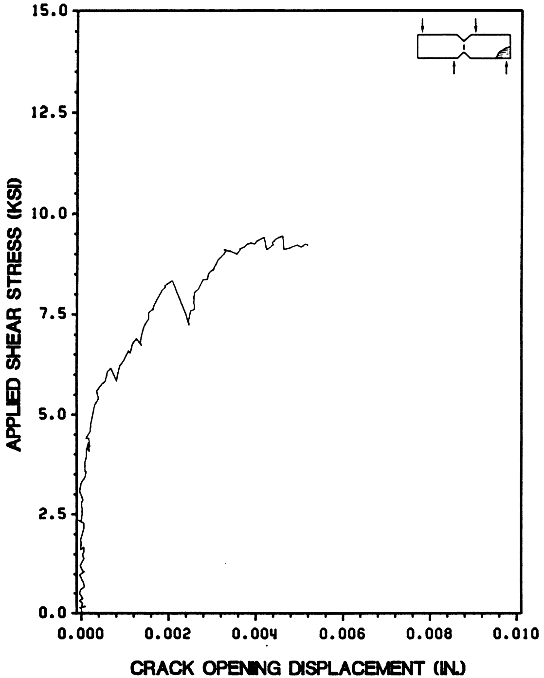
Figure 52. Applied Shear Stress vs. Crack Opening Displacement for a Typical Notched 15° Iosipescu Test
