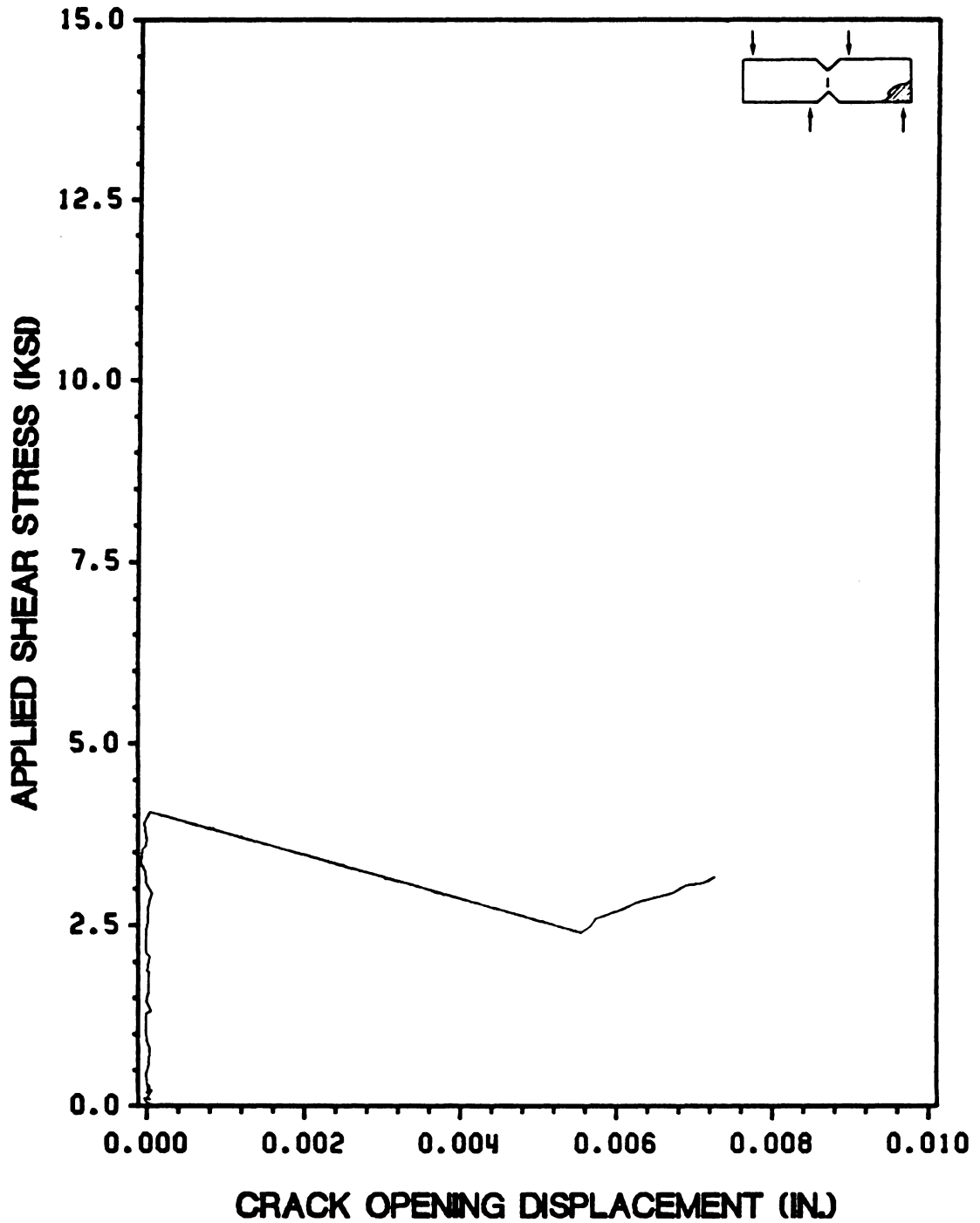
Figure 56. Applied Shear Stress vs. Crack Opening Displacement for a Typical Notched 45° Iosipescu Test
