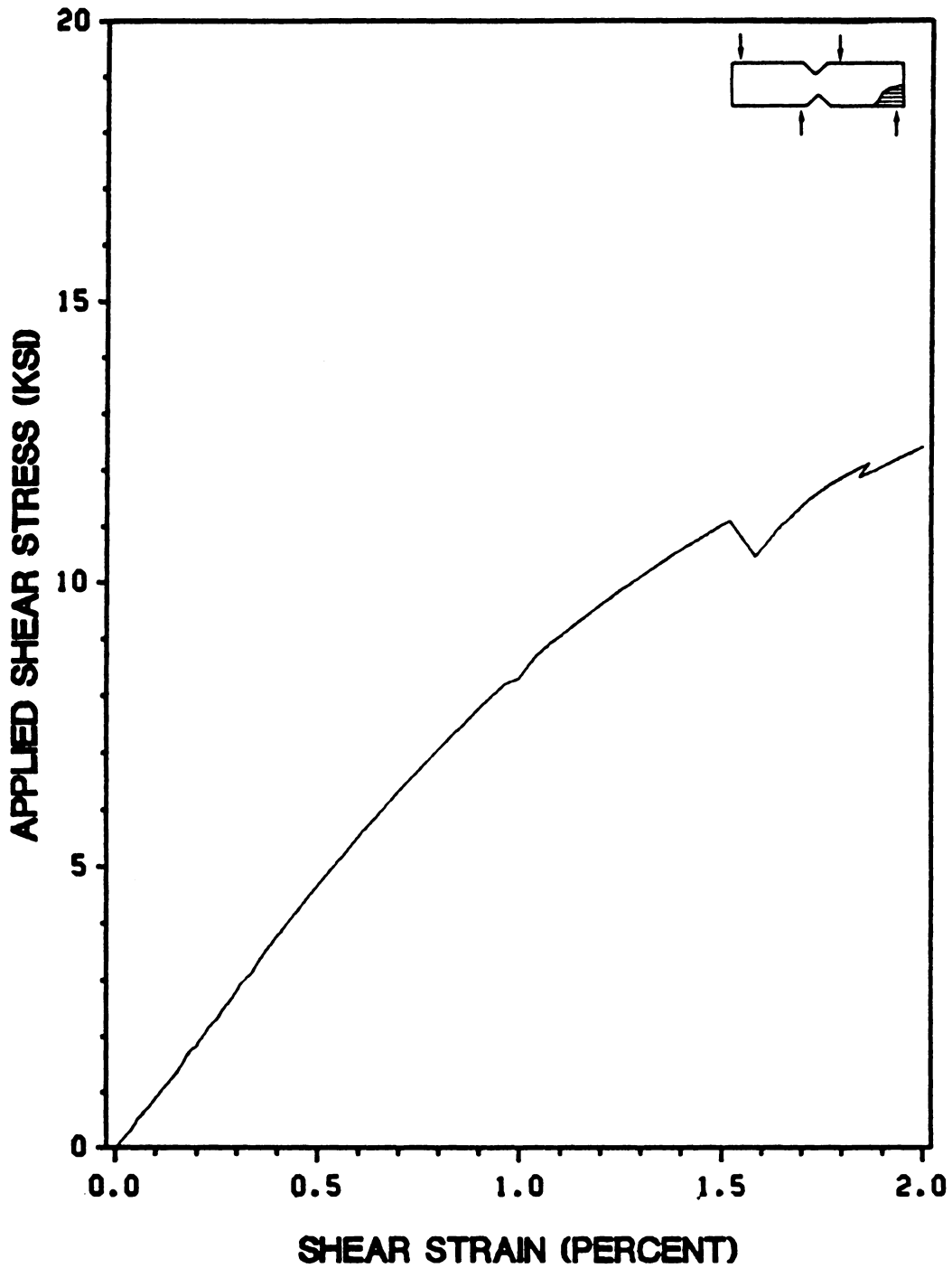
Figure 73. Shear Stress vs. Shear Strain for a Typical 0° Iosipescu Shear Test: AS4/3501-6 Graphite-Epoxy
