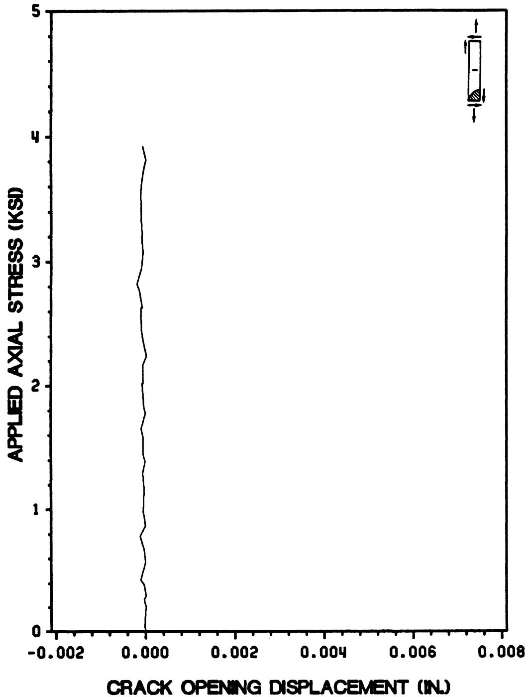
Figure 45. Applied Axial Stress vs. Crack Opening Displacement for a Typical Notched 45° Off-Axis Tensile Coupon Test
