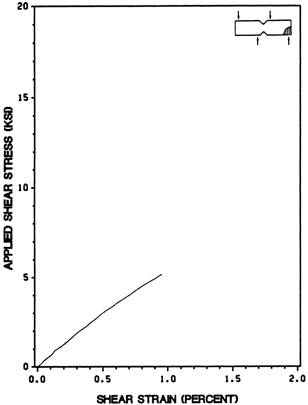
Figure 72. Shear Stress vs. Shear Strain for a Typical 90° Iosipescu Shear Test: AS4/3501-6 Graphite-Epoxy
