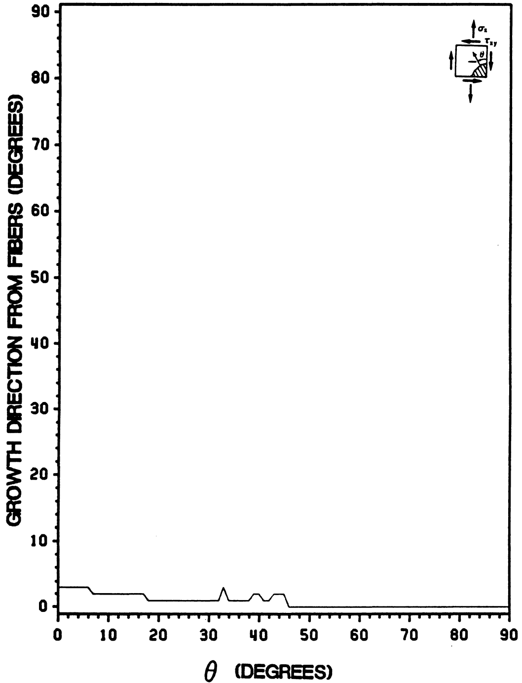
Figure 34. Normal Stress Ratio Predictions for Center-Notched Tensile Coupons: Horizontal Center Notches, Crack Growth Direction Predictions vs. Fiber Angle, AS4/3501-6 Graphite-Epoxy, Shear Coupling Effects Included
