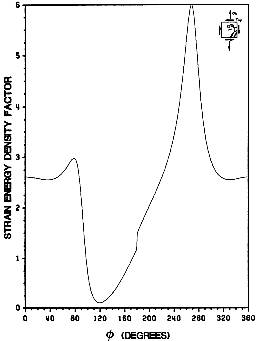
Figure 6. Strain Energy Density Factor vs. \phi : 15° Off-Axis Tensile Coupon, AS4/3501-6 Graphite-Epoxy, Aspect Ratio = 8, 105° Notch
