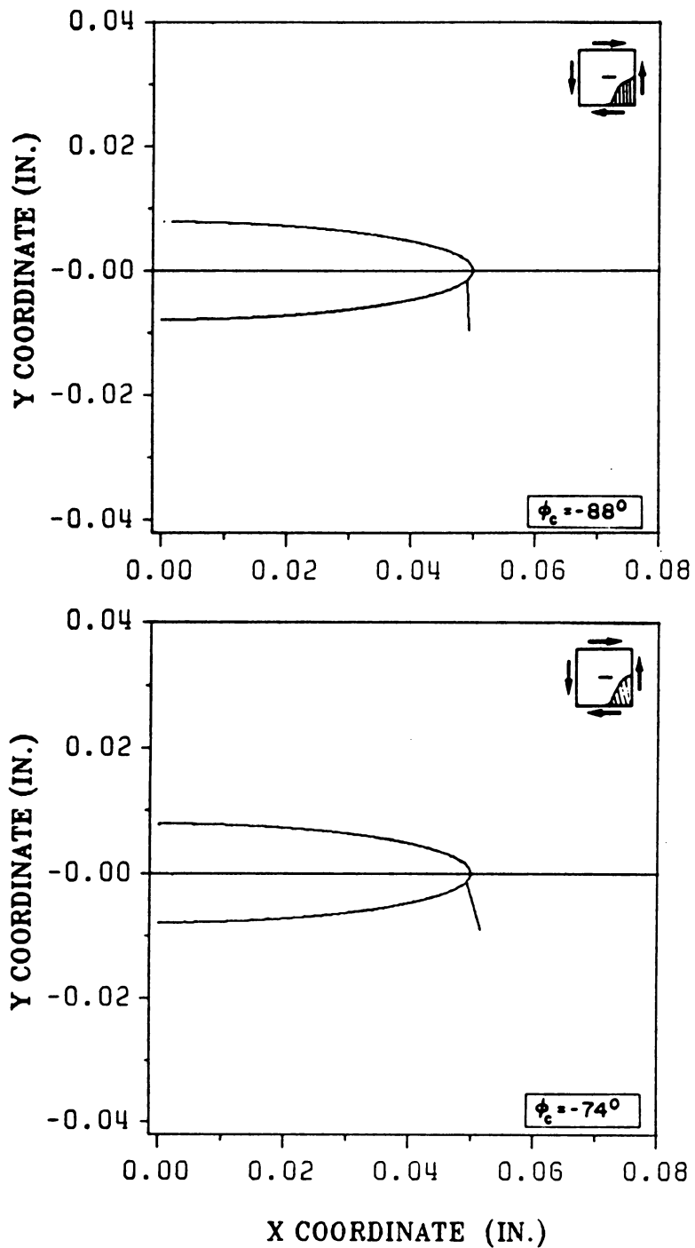
Figure 62. Predicted Locations of Crack Initiation for 0° and 15° Iosipescu Shear Specimens
