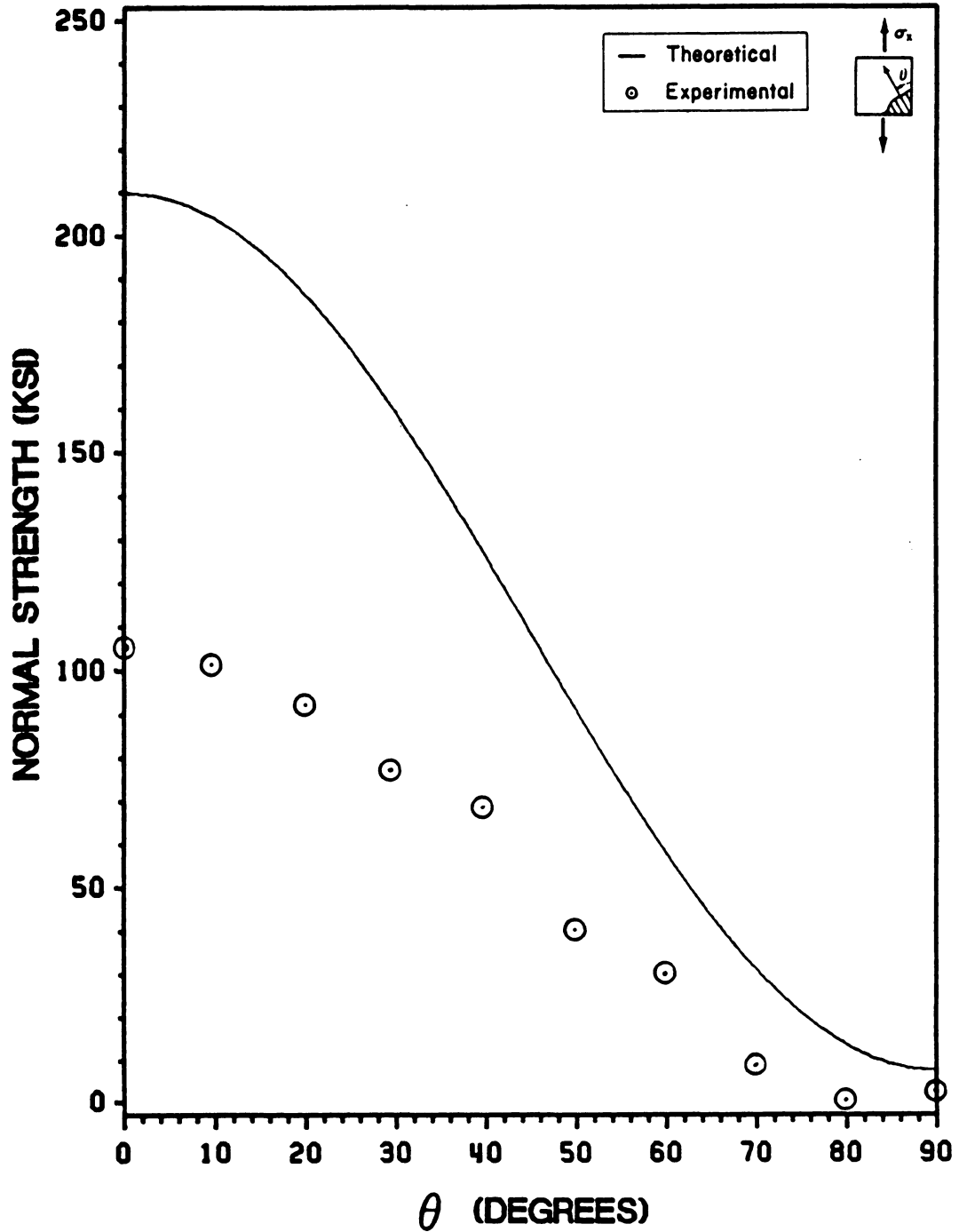
Figure 77. Possible Theoretical and Troughed Specimen Normal Strengths vs. Fiber Orientation
