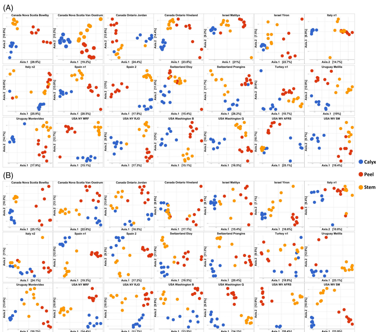
Fig 5. PCoA plots showing the variation in fungal (A) and bacterial (B) community composition among apple tissue types (Calyx, stem and peel). Analysis was based on Bray Curtis dissimilarity metric of CSS normalized OTU table. The figure is arranged in seven columns and three rows for fungi (A) and bacteria (B). Each subpanel corresponds to an orchard. From left to right, the first row shows the results of Nova Scotia Bowlby (Canada), Nova Scotia Van Oostrum (Canada), Ontario Jordan (Canada), Ontario Vineland (Canada), Matitya (Israel), Yiron (Israel) and orchard n1 (Italy). The second row shows the results from orchard n2 (Italy), Corbins (Spain), Alcarràs (Spain), MRFs (Switzerland), Etoy (Switzerland), orchard 1 (Turkey), Melilla (Uruguay). The third row shows the results from Montevideo (Uruguay), RJO (NY, USA), Washington B (USA), Washington Q (USA), AFRS (WV USA), SM (WV USA). A and B are arranged in the same order. [Color figure can be viewed at wileyonlinelibrary.com ]
