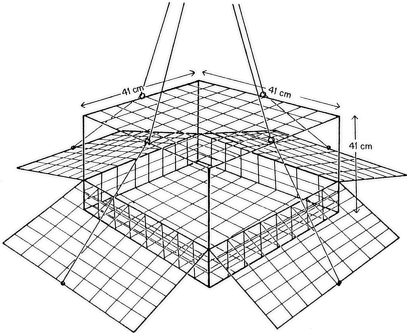
Figure 11. Type 1, Scrap Containment Device.
