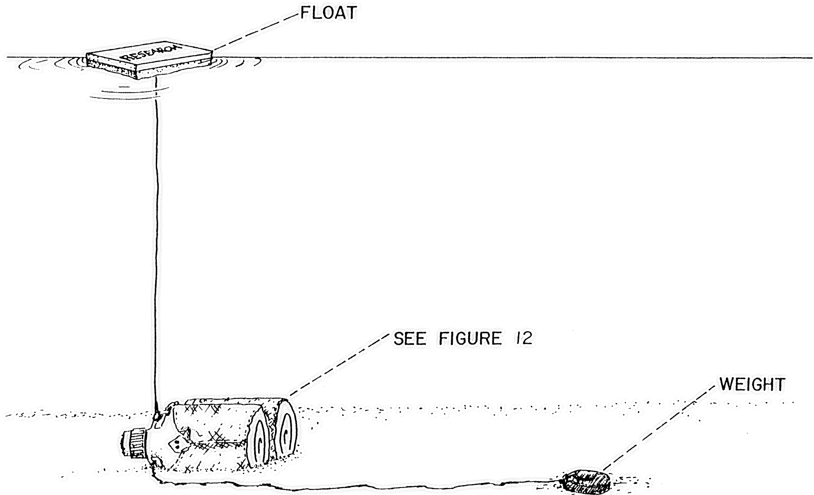
Figure 13. Anchorage of the Type 2, Scrap Containment Device.
