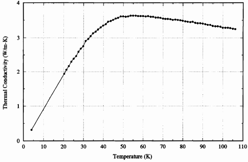
Figure 4.3. Thermal Conductivity of YBa 2 Cu 3 O 7-x (Christopher Newport University, 1993)
