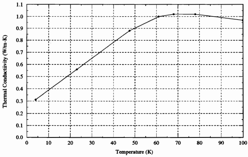
Figure 4.4. Thermal Conductivity of BiSrCaCu 2 O x (Peacor and Uher, 1989)
