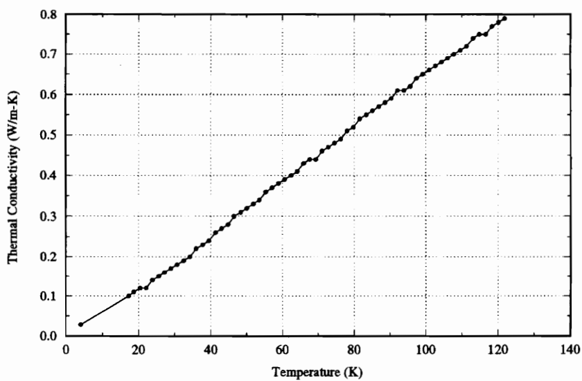
Figure 4.6. Thermal Conductivity of Fused Silica (Christopher Newport University, 1993)
