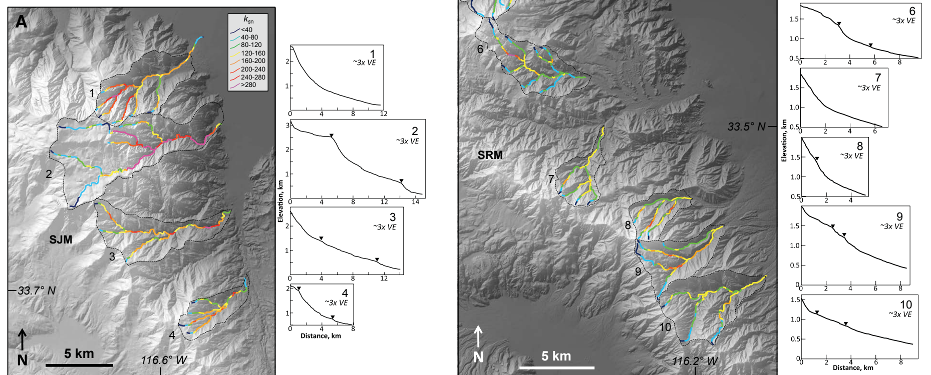
Figure 8. Normalized steepness index ( k_{sn} ) maps and longitudinal profiles of main streams in studied basins in the San Jacinto Mountains (SJM) (A), Santa Rosa Mountains (SRM) (B), and Little San Bernardino Mountains (LSBM) (C). Values of k_{sn} range from <40 to >280 as shown in the legend. Black triangles denote prominent knickzones on longitudinal profiles. Longitudinal profiles within each region are shown at the same scale. Profiles for the SJM and SRM are plotted with ~3x vertical exaggeration (VE), whereas those for the LSBM are shown with ~8x VE due to the lower relief. Locations of the maps are shown on Figure 3A. SBM—San Bernardino Mountains. (Continued on following page.)
