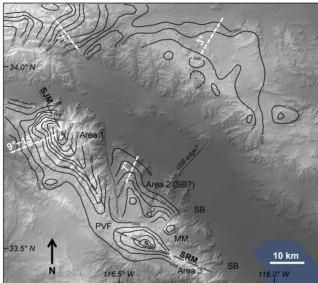
Figure 13. Structure contour map of the weathered erosion surface in the San Jacinto Mountains (SJM), Little San Bernardino Mountains, and southern San Bernardino Mountains. Contour interval is 200 m. Thick dashed gray line indicates the axes of the SJM and Santa Rosa Mountains (SRM), respectively. Thin dashed lines are selected faults (Rogers, 1965) that seem to disrupt contours. Dashed line labeled “cSB edge?” marks the proposed northern limit to the tilted central Salton block at about the location of Point Happy (location shown on Figure 14) as proposed by Dorsey and Langenheim (2015). Areas 1–3 are locations discussed in the text. White dashed lines illustrate directions along which mean surface gradients have been estimated (values shown). DC—Deep Canyon; MM—Martinez Mountain; PVF—Pinon and Vandeventer flats; SB—Salton block (Dorsey and Langenheim, 2015).
