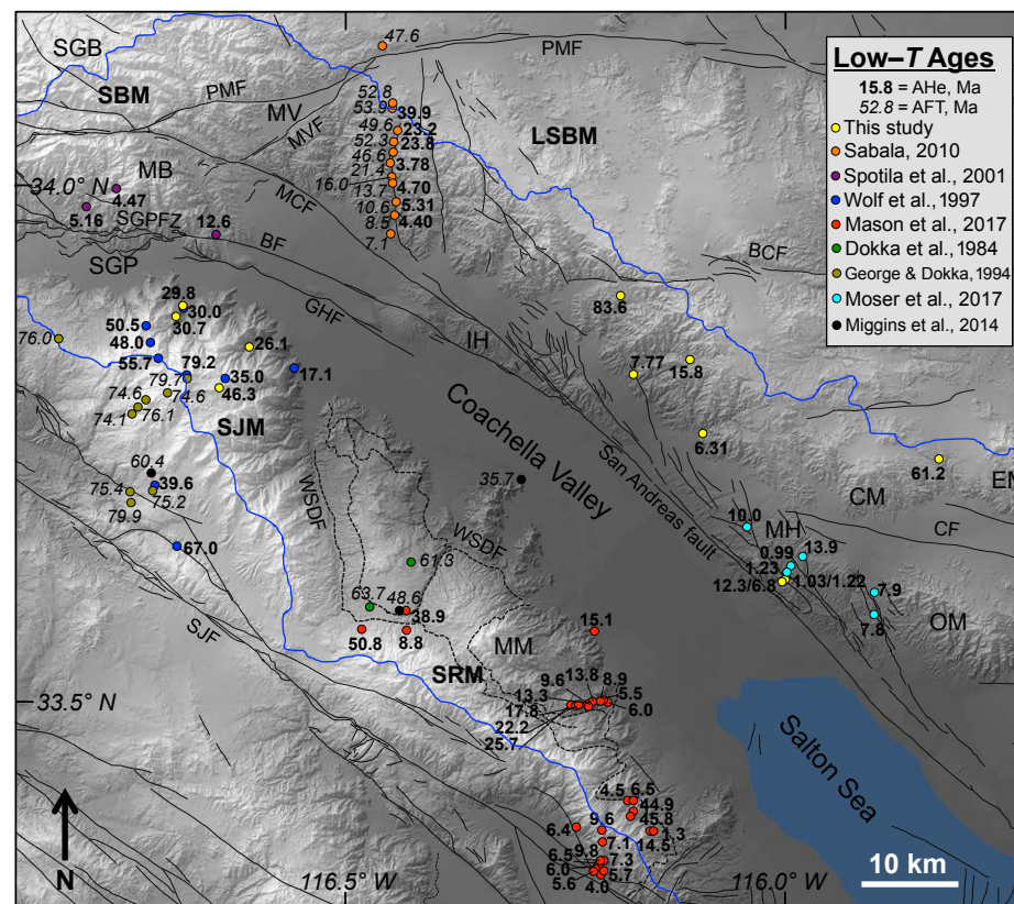
Figure 2. Map of the Coachella Valley showing published and new low-temperature (low-T) apatite (U-Th)/He (AHe) and apatite fission-track (AFT) thermochronometry ages. Blue line indicates the catchment boundary of the northern Coachella Valley. Ages from Moser et al. (2017) from the Mecca Hills are shown as averages (not calculated in the original study), in some cases with one outlier age dropped. The two ages we measured in the Mecca Hills are listed as doubles (e.g., 12.3/6.8), given that Moser et al. (2017) dated basically the same location (our age is listed first, Moser et al. [2017] age is given second). Note that some Sabala (2010) locations have both AHe and AFT ages. Locations shown are: CM—Cottonwood Mountains; EM—Eagle Mountains; IH—Indio Hills; LSM—Little San Bernardino Mountains; MB—Morongo block; MH—Mecca Hills; MM—Martinez Mountain; MV—Morongo Valley; OM—Orocopia Mountains; SBM—San Bernardino Mountains; SGB—San Geronio block; SGP—San Geronio Pass; SJM—San Jacinto Mountains; SRM—Santa Rosa Mountains. Faults shown as solid black lines are: BCF—Blue Cut fault; BF—Banning fault; CF—Chiriaco fault; GHF—Garnet Hill fault; MCF—Mission Creek fault; MVF—Morongo Valley fault; PMF—Pinto Mountain fault; SJF—San Jacinto fault; SGPZ—San Geronio Pass fault zone; WSDF (dashed)—West Salton detachment fault (WSDF after Axen and Fletcher, 1998).
