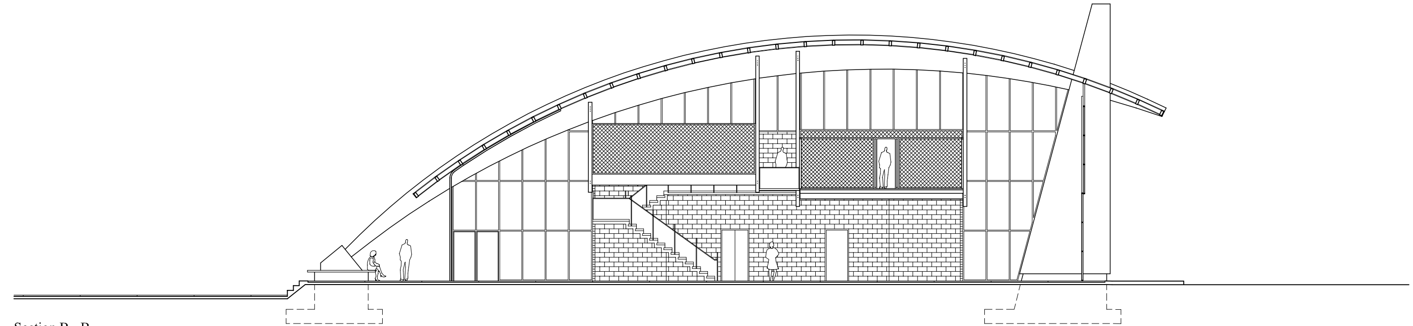
Section B - B
