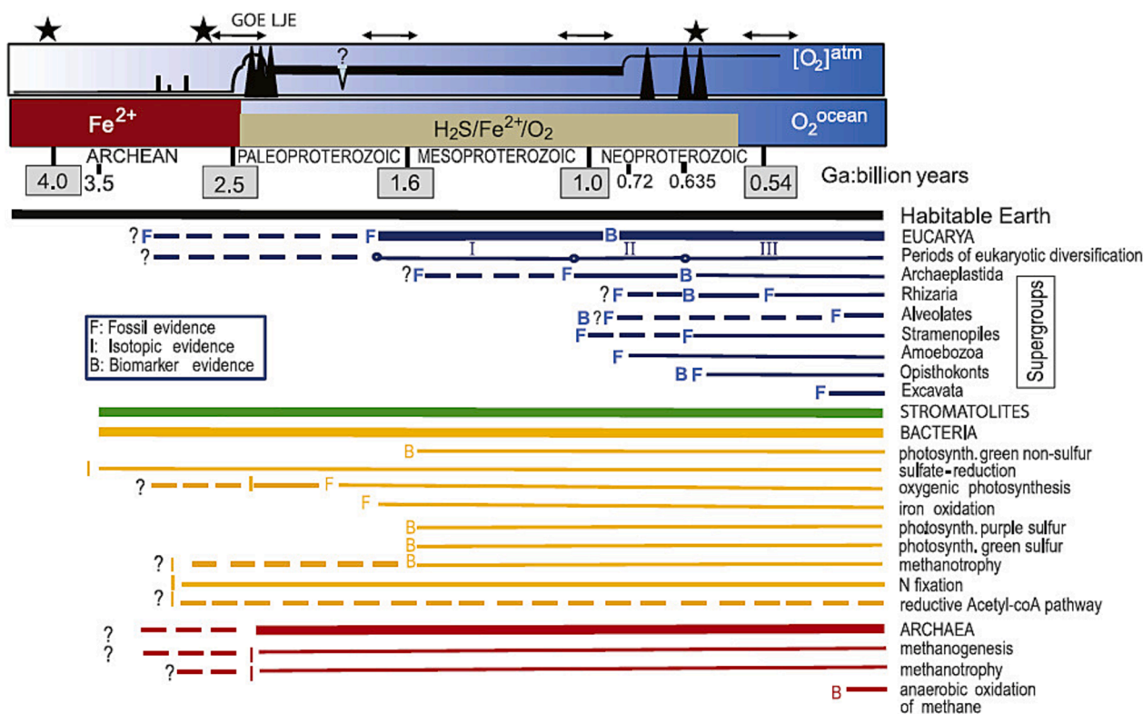
Fig. 13. Temporal evolution of microbial metabolisms with the global evolution of atmospheric and oceanic composition throughout geological time (Javaux and Lepot, 2018).
