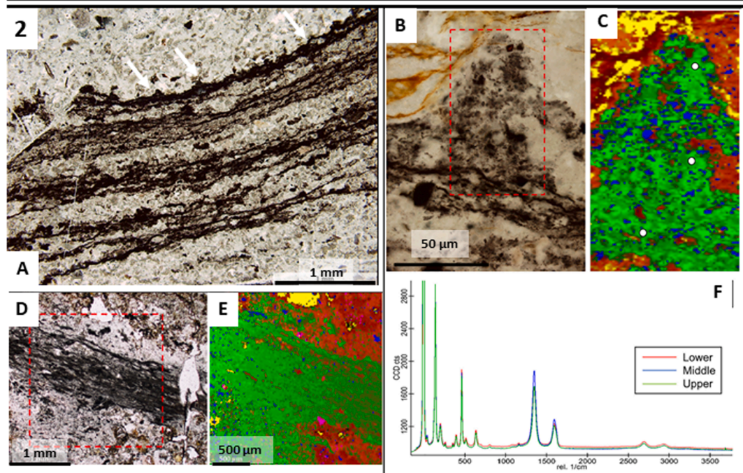
Fig. 5. Fossilised Archaean MISS. Panel 1. Variety of MISS textures found in the 3.48 Ga Dresser Formation tidal flat sediments (Pilbara) and their modern counterparts including (A) mud cracks, (B) tufted textures, (C) parallel mat laminations (Noffke et al., 2013). Panel 2. MISS textures from the 3.47 Ga Middle Marker Formation, Barberton. (A) Tufted mat texture with detail of tuft in optical microscopy, (B) and Raman spectral map (C) showing the carbonaceous nature of the tuft, (D) optical and (E) Raman spectral map of the fine, carbonaceous laminations of the microbial mats (Raman spectral maps: green = carbon; yellow/orange = quartz; blue = anatase), (F) Raman spectrum showing the mature nature of the carbonaceous matter with the D and G peaks centred around 1350 and 1580 \text{cm}^{-1} (Hickman-Lewis et al., 2018).
