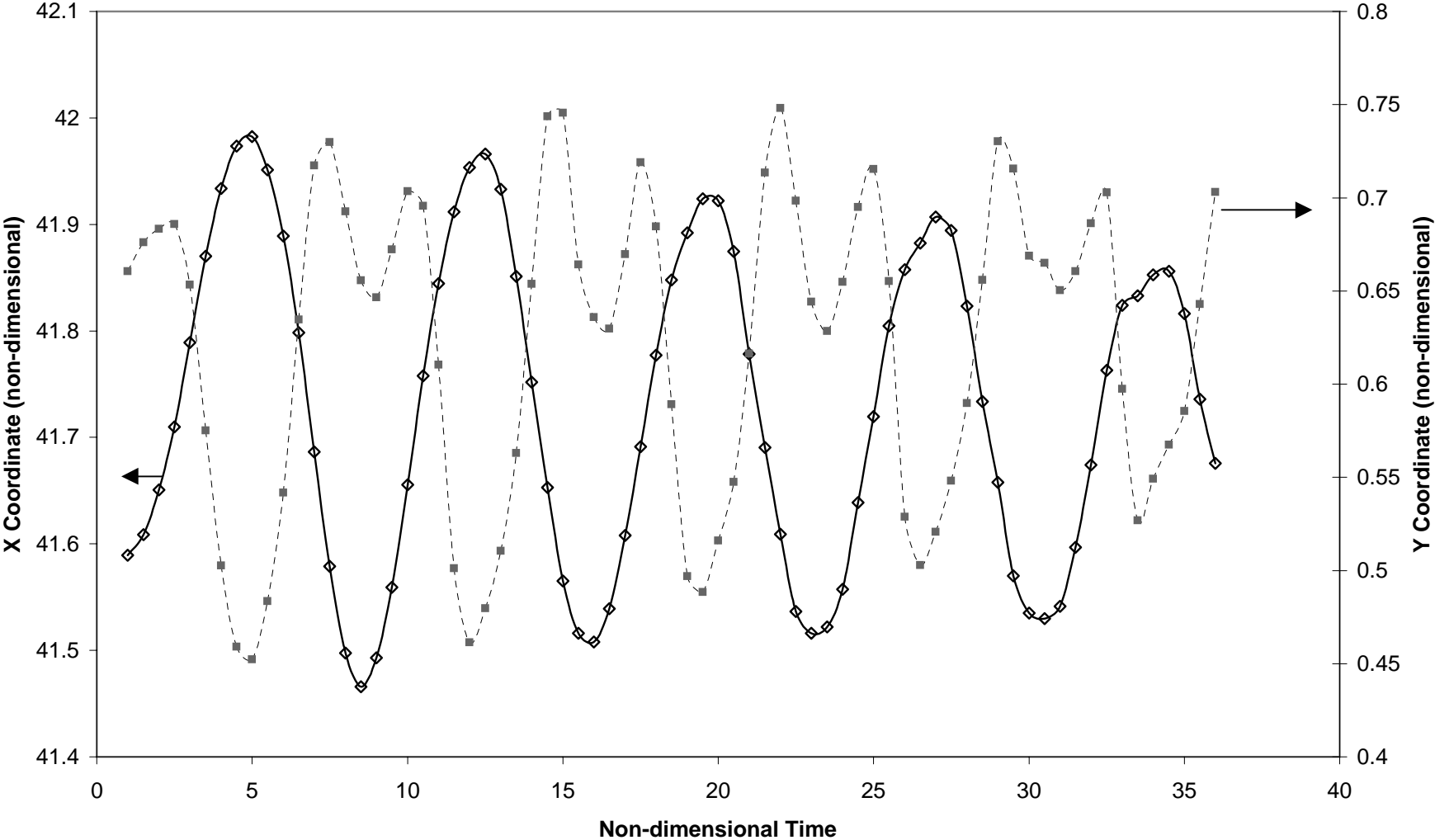
Figure I-10: The motion of the uppermost node of an oscillating inflatable dam as a function of time.
