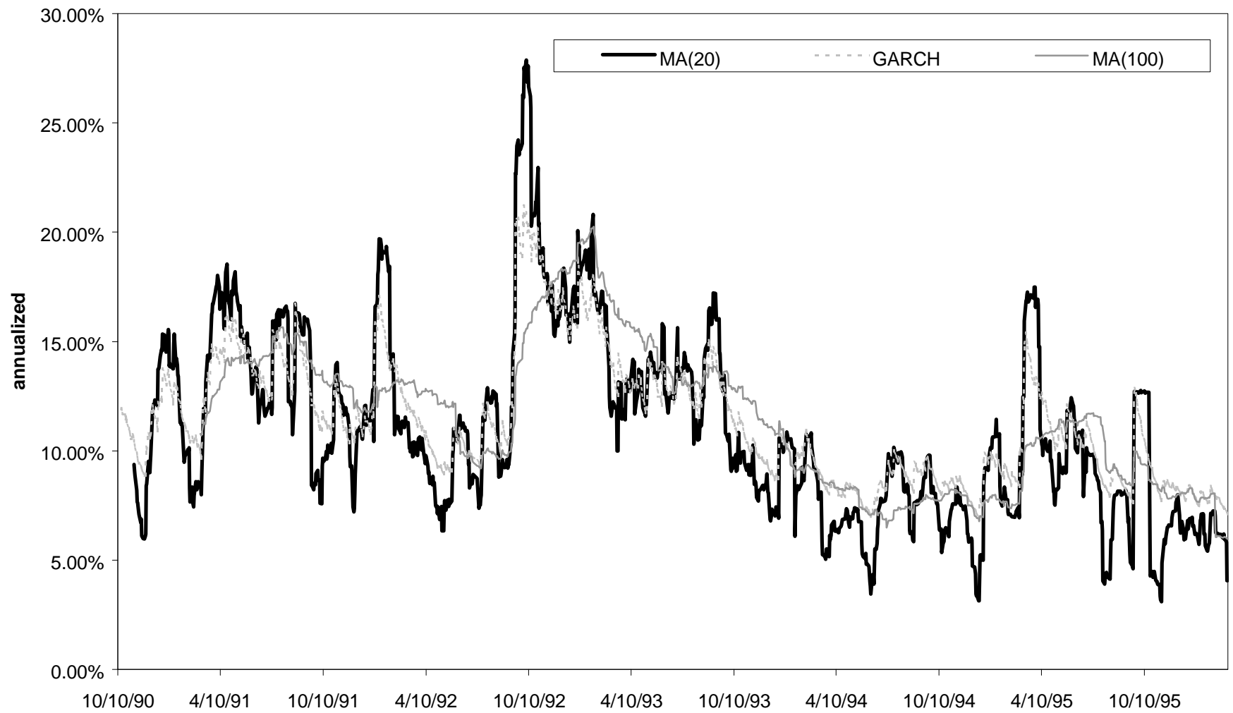
Figure 3: Time Series Volatility Measures
