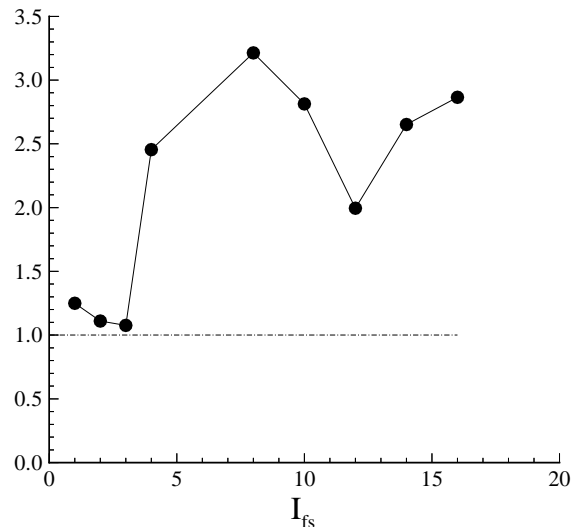
(b) Supercritical M_\infty = 0.85 .
