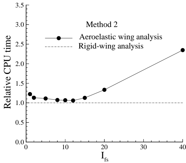
(a) Subcritical M_\infty = 0.7 .
