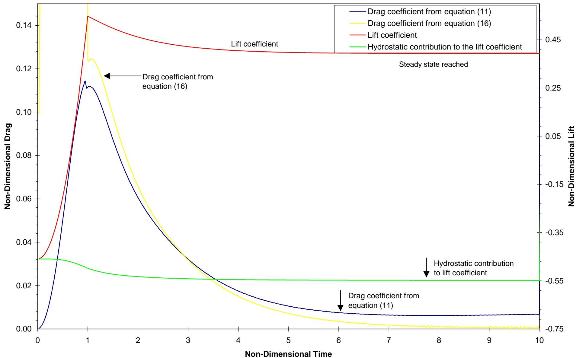
Figure II-13: Sample plot of the transient lift and drag for supercritical flow
