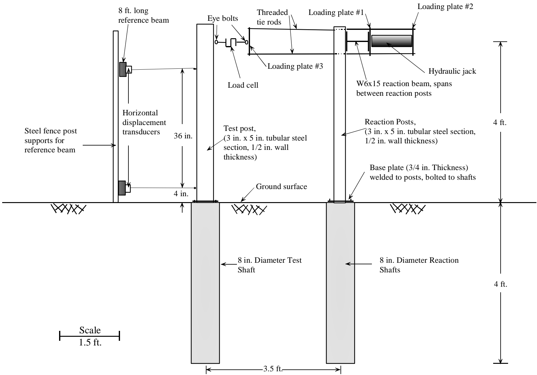
Figure 3.4: Section View of Test Setup
