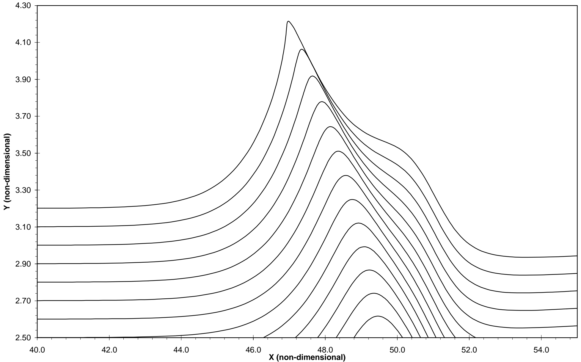
Figure II-11: Sample free surface profile for a upstream breaking wave.
