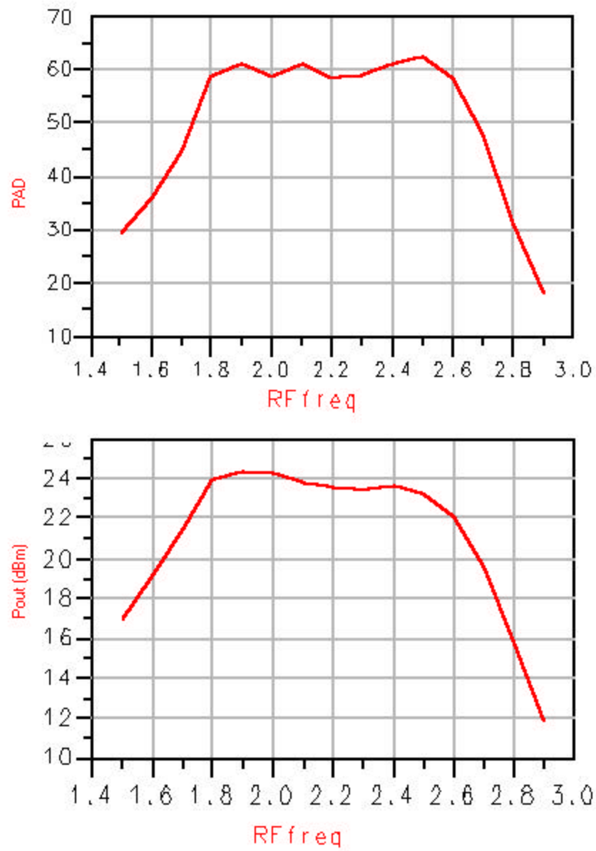
Figure 5.13. Transmission-line broadband class-E amplifier's power added efficiency and output power.
