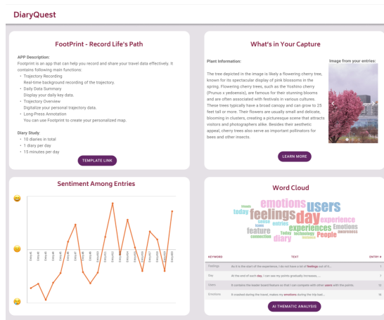
Figure 1: DiaryQuest System
