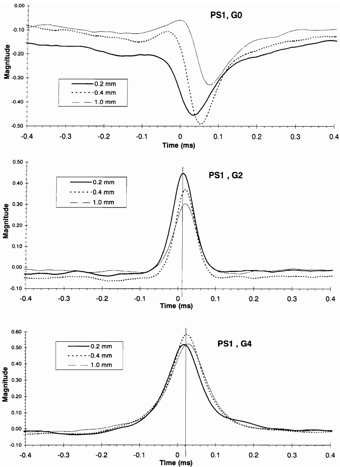
Figure 6.5.2 PS1 HF/PHW cross-correlation vs. y_{wire} for G0, G2, and G4.
