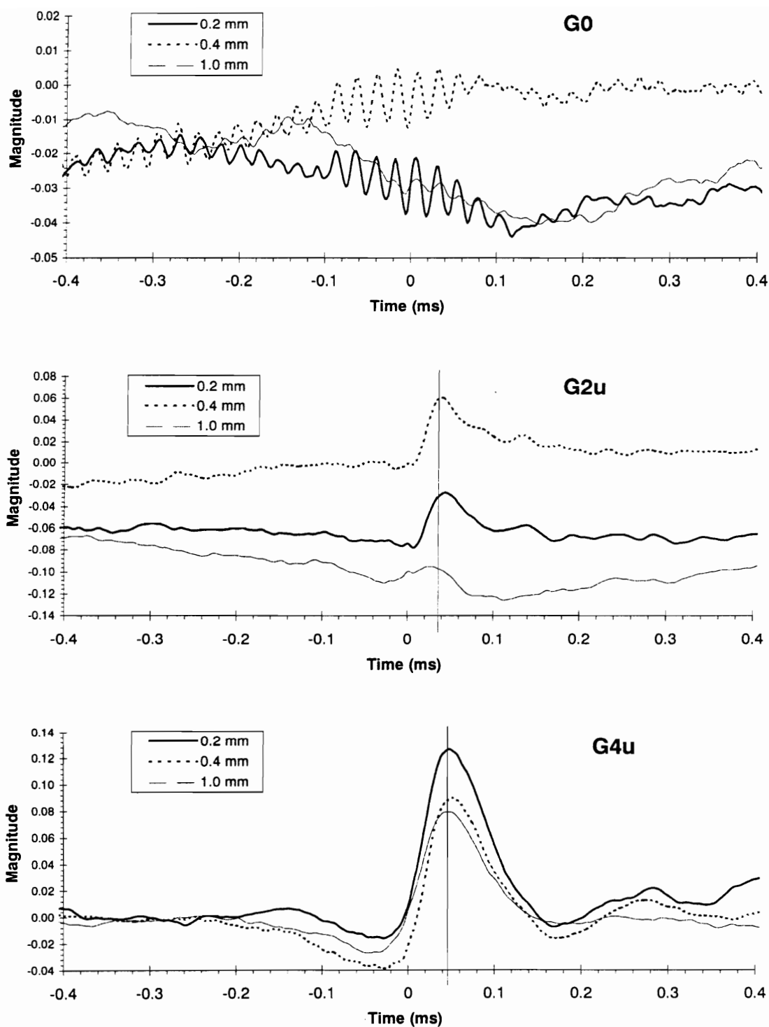
Figure 6.5.1 DS1 cross-correlation vs. y_{wire} for G0, G2u, and G4u.
