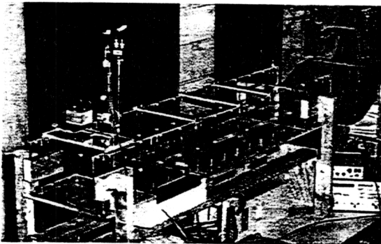
Fig.1 Wall-jet facility
