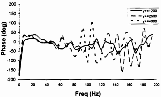
Fig.18 vq phase across boundary layer
