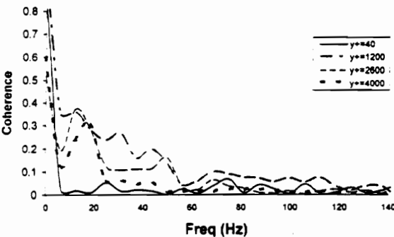
Fig.17 vq coherence across boundary layer
