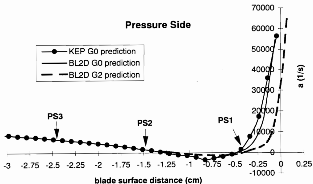
Figure 5.1.6 BL2D pressure side (PS) strain ( a=dU/dx ) prediction for G0 and G2 based on measured blade surface pressure distributions.
