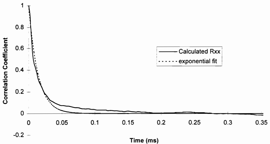
Figure 2.2.2 Example of the measured auto-correlation and the exponential fit used to find the integral time scale.
