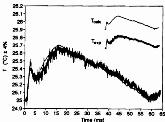
Fig. 6 Calculated and experimental surface temperature
