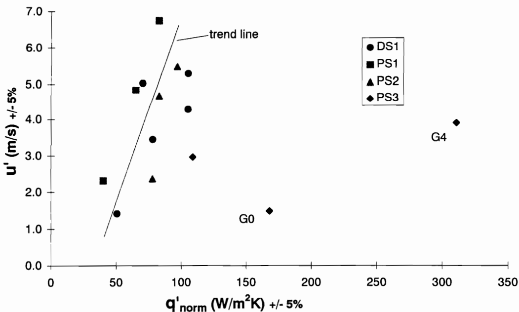
Figure 7.9 u' vs. q' .
