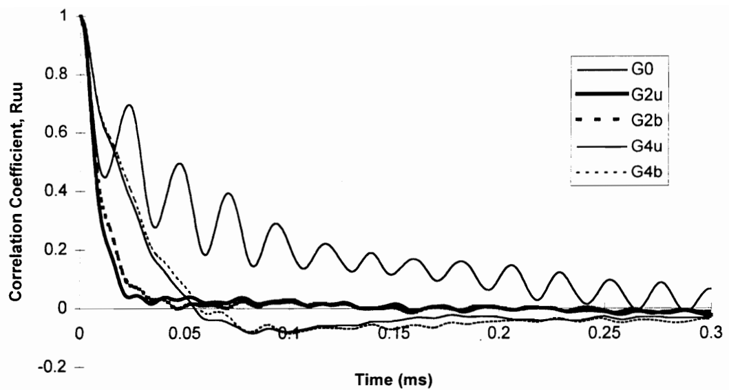
Figure 2.2.1 Examples of the auto-correlation function calculated from the energy spectrum for the five grid conditions measured above DS1.
