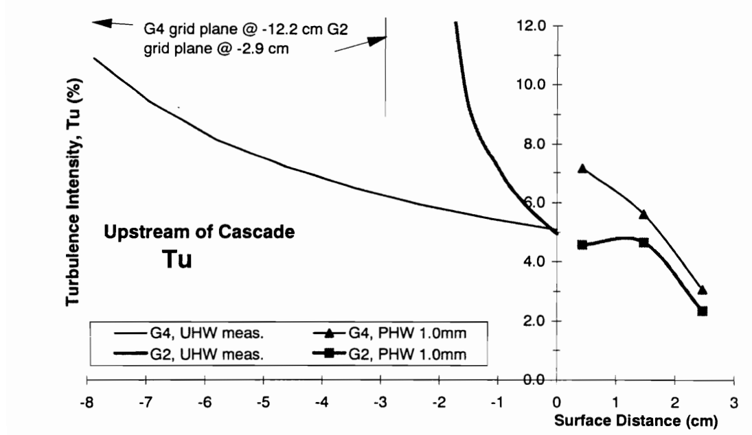
Figure 5.2.3 Fluctuating velocity ( u' ) upstream and into passage (1 mm wire position above PS), Grid 4 vs. Grid 2.
