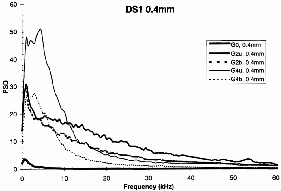
Figure 6.1.2 Hot-wire Energy spectra over DS1 at y = 0.4 mm
