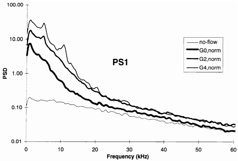
Figure 6.2.4 Heat flux spectra at PS1 comparing grids.
