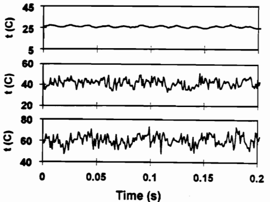
Fig.10 Temperature signal at y^+=10, 100 , and 2600 .
