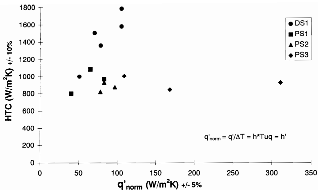
Figure 7.8 Heat transfer coefficient vs. q' .
