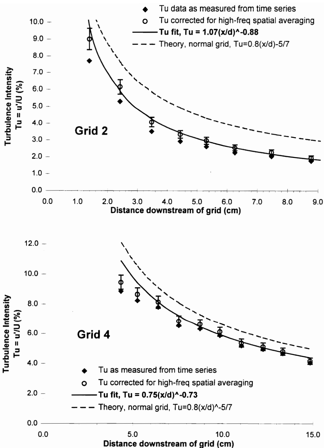
Figure 4.2.1 Grid turbulence: Tu decay behind G2 and G4, U = 120 m/s.
