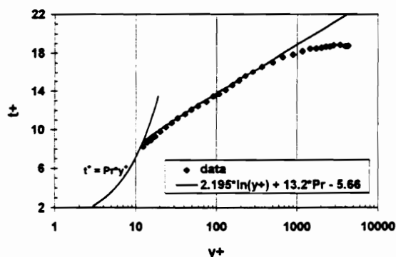
Fig.4 Mean temperature profile across boundary layer
