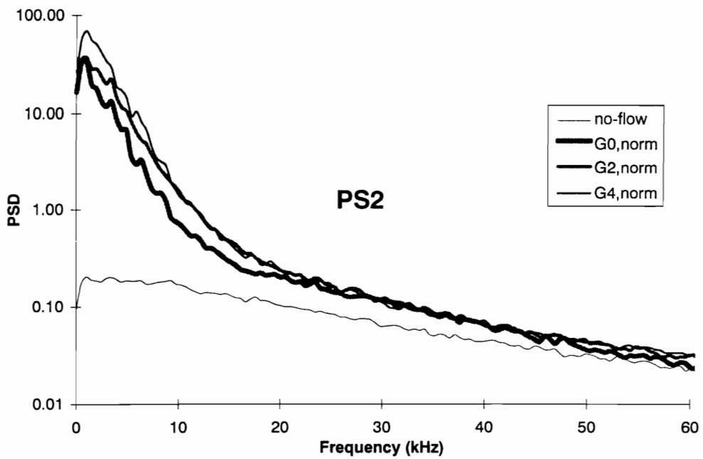
Figure 6.2.5 Heat flux spectra at PS2 comparing grids.
