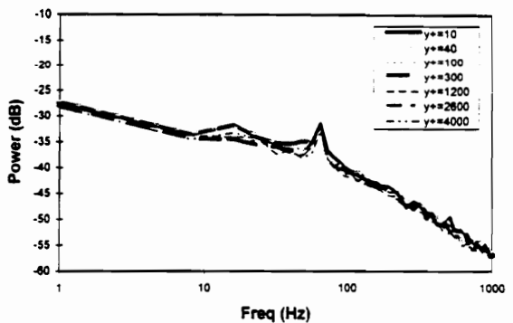
Fig.14 Heat flux autospectrum across boundary layer
