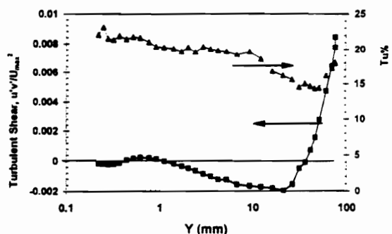
Fig.6 Tu_\delta\% and u'v' across boundary layer
