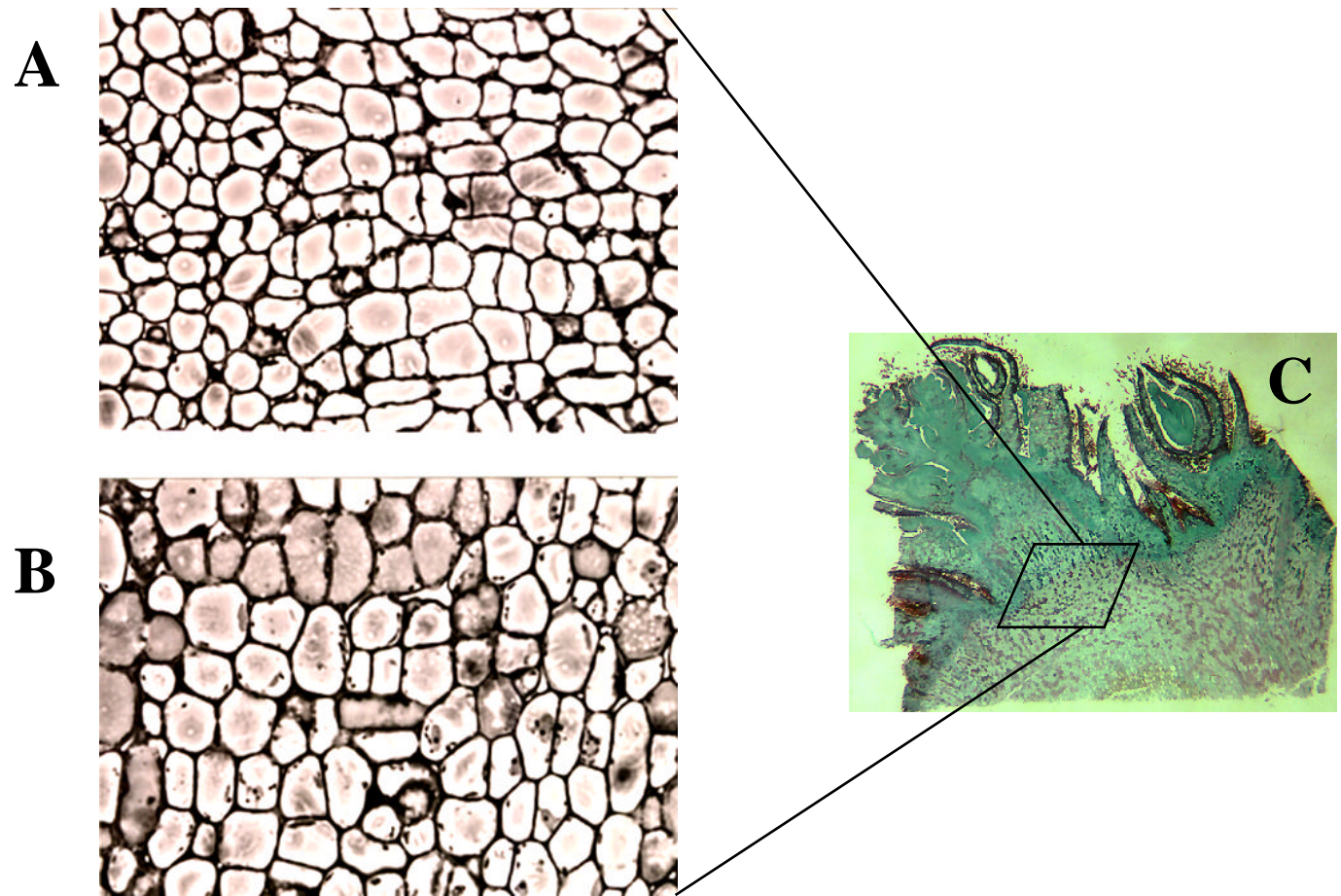
Fig. 3.1. Bud sections of the primary axis of 'Riesling' vines without any cellular abnormalities (40X) at 46 and 56 days after budbreak. A) 'Riesling' buds from Somerset Vineyard were sampled at 46 days after budbreak on 30 May, 1994. B) 'Riesling' buds from Somerset Vineyard were sampled at 56 days after budbreak on 9 June, 1994. C) A section of 'Riesling' bud with primary bud axis and two secondary bud axes.
