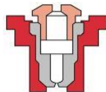
Figure 7. Pre-orifice flat-fan nozzles reduce the volume of driftable droplets.
