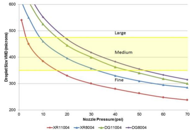
Figure 8. Comparing the mean droplet size of two extended range flat-fans (XR) with two pre-orifice flat-fans (DG).
