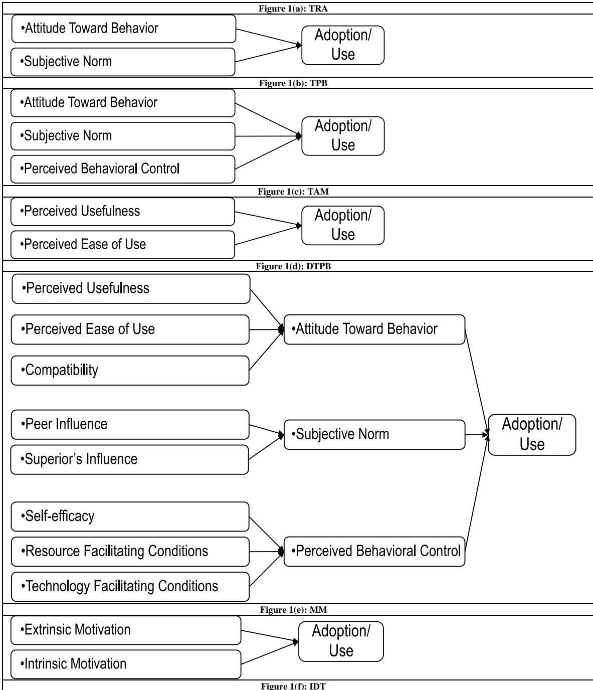
Figure 1: Visualization of the Models Tested in Our Research
