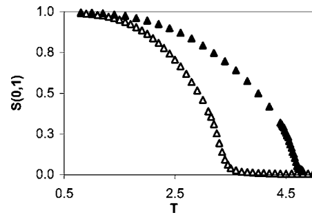
FIG. 3. S(0,1) as a function of T for f=0.50 , E=2.0 . Open (solid) triangles are for the 40 \times 40 ( 60 \times 60 ) system.
