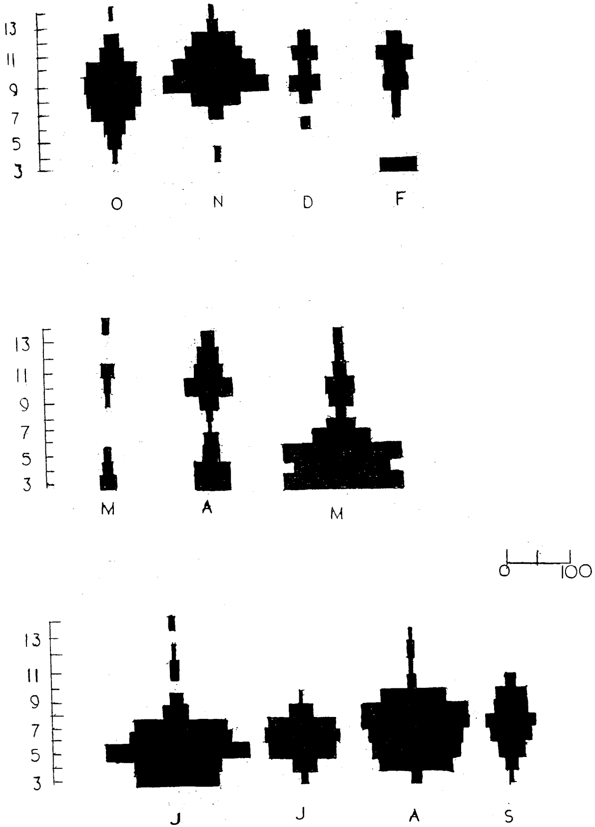
FIG. 2. Number of animals in each size class at Bradley Run from October 1986 to September 1987. Numbers on left are size classes in mm. Scale on right indicates number of animals.
