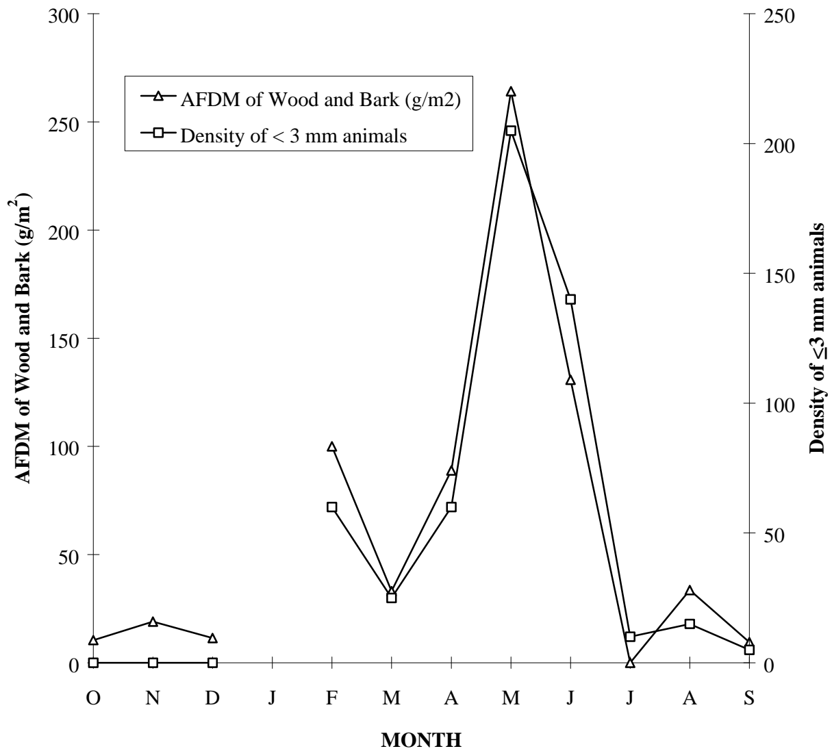
FIG. 10. Relationship of quantity of ash-free dry mass of wood and bark to density of smallest size class at Bradley Run.
