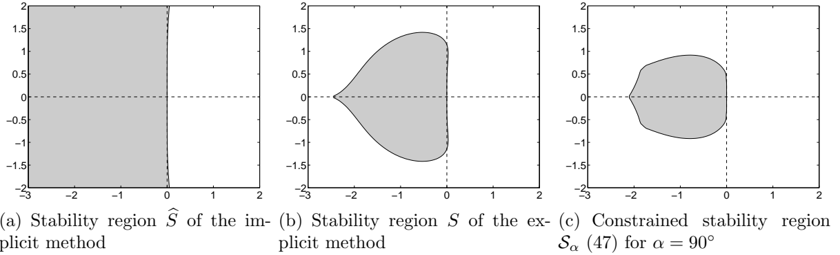
Figure 1: Stability regions for the IMEX-DIMSIM-2B pair
