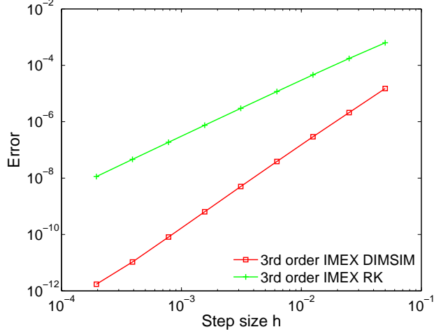
Figure 4: Convergence results for third-order IMEX schemes on the van der Pol equation.
