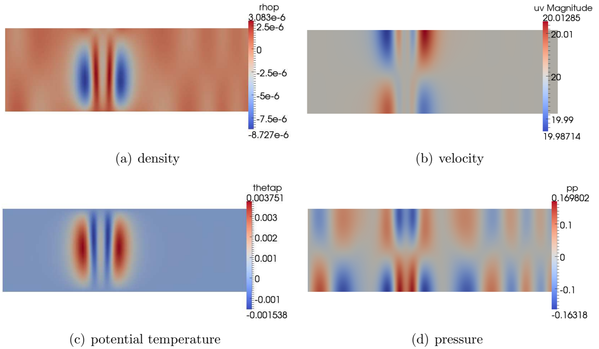
Figure 5: Solution of the gravity waves after 900 simulation seconds. The results are obtained with a third-order discontinuous Galerking space discretization and third-order IMEX DIMSIM time integration.
