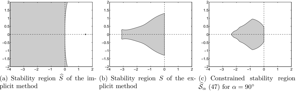
Figure 3: Stability regions for the IMEX-DIMSIM-3B pair of schemes
