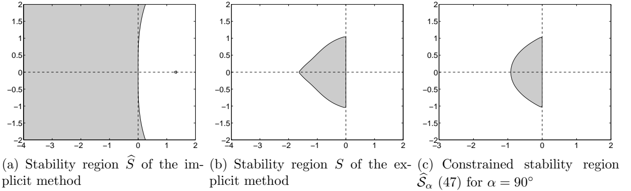
Figure 2: Stability regions for the IMEX-DIMSIM-3A pair of schemes
