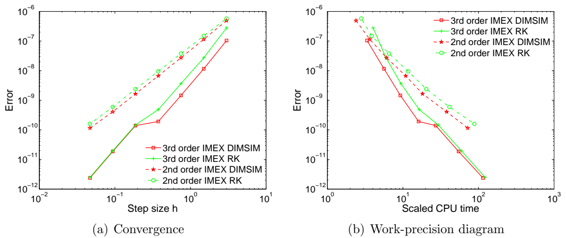
Figure 6: Integrated L_2 errors against time steps (a) and CPU time (b) for difference IMEX schemes. The errors are computed after 30 s of simulation. A geometric sequence of step sizes, \tau , \tau/2 , \tau/4 and so on, is used.
