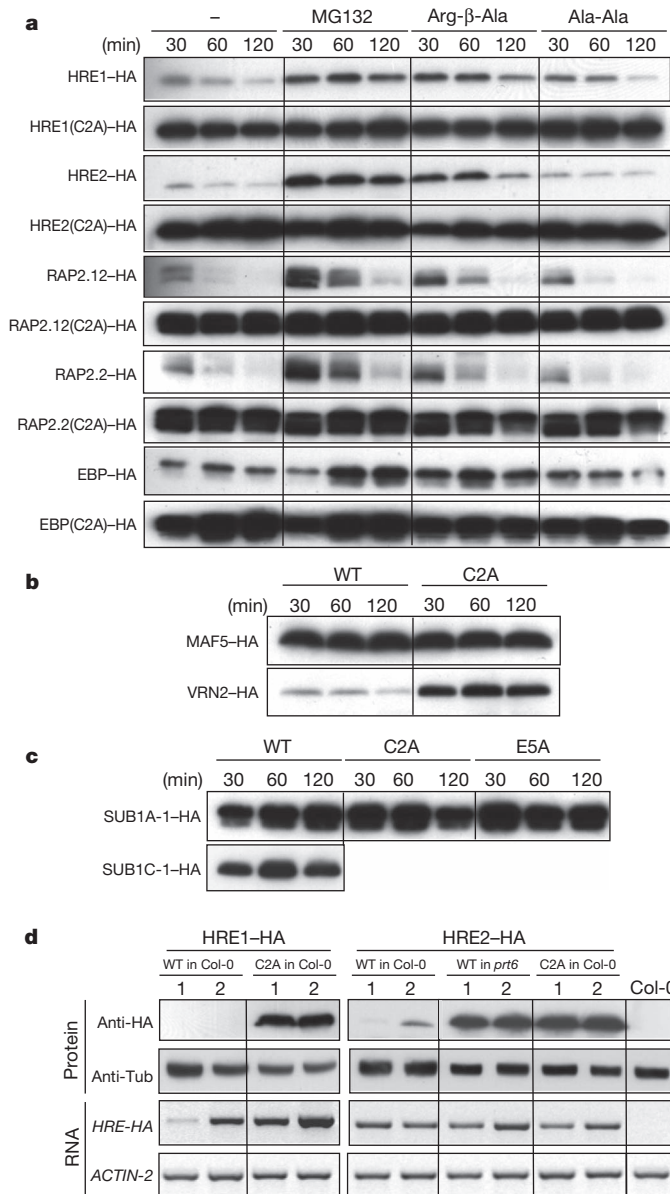
Figure 2 | Group VII ERF transcription factors are substrates for the N-end rule pathway in vitro and in vivo . a , Western blot analysis of in vitro stability of HA-tagged wild-type and C2A variants of Arabidopsis group VII ERFs in the absence or presence of MG132, N-end rule pathway competitive dipeptide (Arg-β-Ala) or non-competitive dipeptide (Ala-Ala). b , In vitro stability of wild-type and C2A VRN2-HA and MAF5-HA. c , In vitro stability of HA-tagged rice ERFs. d , In vivo protein stability and RNA expression levels of wild-type and C2A variants of HRE1-HA and HRE2-HA ectopically expressed in Arabidopsis , shown for two independent transformed lines (1 and 2).
